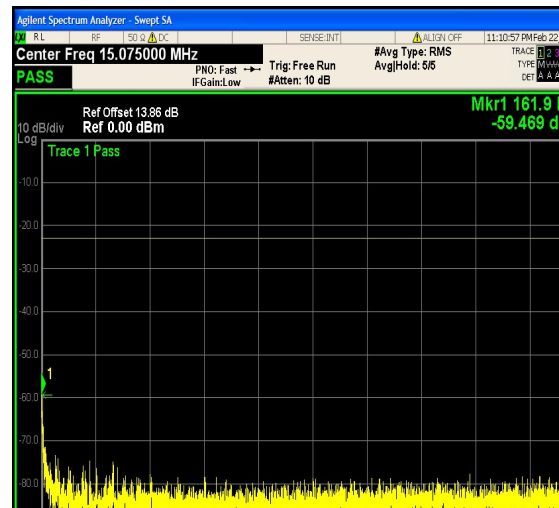
1-N5-PC3-15-10-H-24-CP-64QAM-Outer_Ful I-52@0.15-30-Ant1--59.47--23-PASS
