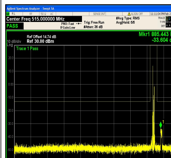
1-N5-PC3-15-10-H-24-CP-64QAM-Outer_Ful I-52@0-0.009-0.15-Ant1--54.83--33-PASS
