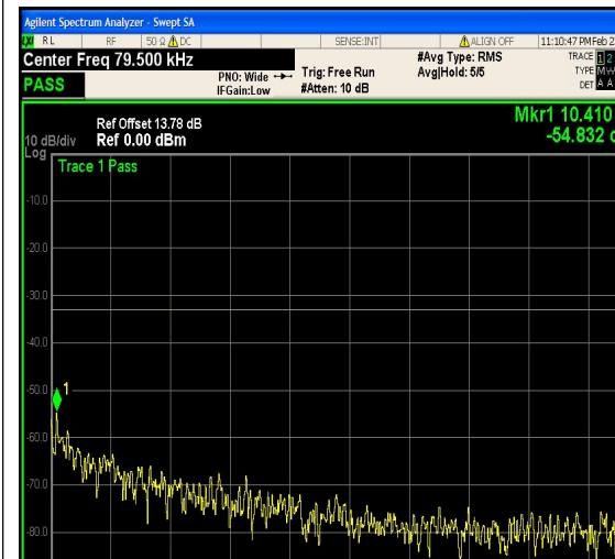
1-N5-PC3-15-10-H-24-CP-64QAM-Outer_Ful I-52@0-0.009-0.15-Ant1--54.83--33-PASS
