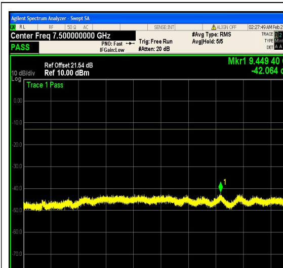
1-N5-PC3-15-20-M-17-CP-QPSK-Edge_1RB _Right-1@105-3000-12000-Ant1--42.06--13- PASS
