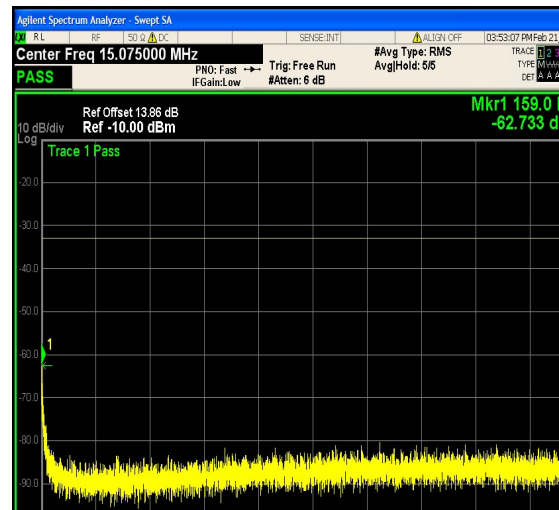
1-N66-PC3-15-5-M-17-CP-QPSK-Edge_1RB _Right-1@24-0.15-30-Ant1--62.73--33-PASS
