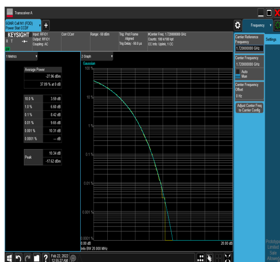
1-N66-PC3-15-20-L-3-DFT-16QAM-Outer_Fu ll-100@0-8.42-100%-0.00-8.42-PASS-≤13
