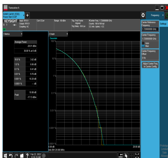
1-N66-PC3-15-20-L-2-DFT-QPSK-Outer_Full -100@0-8.41-100%-0.00-8.41-PASS-≤13
