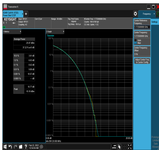
1-N66-PC3-15-15-H-9-CP-256QAM-Outer_F ull-79@0-8.42-100%-0.00-8.42-PASS-≤13
