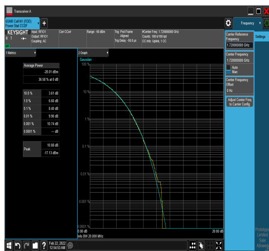
1-N66-PC3-15-20-L-1-DFT-PI2BPSK-Outer_ Full-100@0-8.40-100%-0.00-8.40-PASS-≤13
