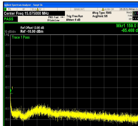
1-N66-PC3-15-10-L-11-DFT-64QAM-Edge_1 RB_Right-1@51-0.15-30-Ant1--65.47--33-PA SS
