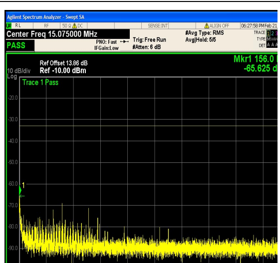
1-N66-PC3-15-10-M-15-DFT-256QAM-Out _Full-50@0-0.15-30-Ant1--65.62--33-PASS
