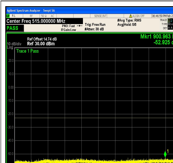
1-N66-PC3-15-10-H-1-DFT-PI2BPSK-Edge_ 1RB_Left-1@0-30-1000-Ant1--52.92--23-PA SS
