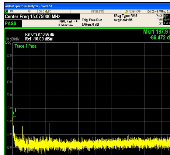
1-N66-PC3-15-10-H-9-DFT-16QAM-Outer_F ull-50@0-0.15-30-Ant1--66.47--33-PASS
