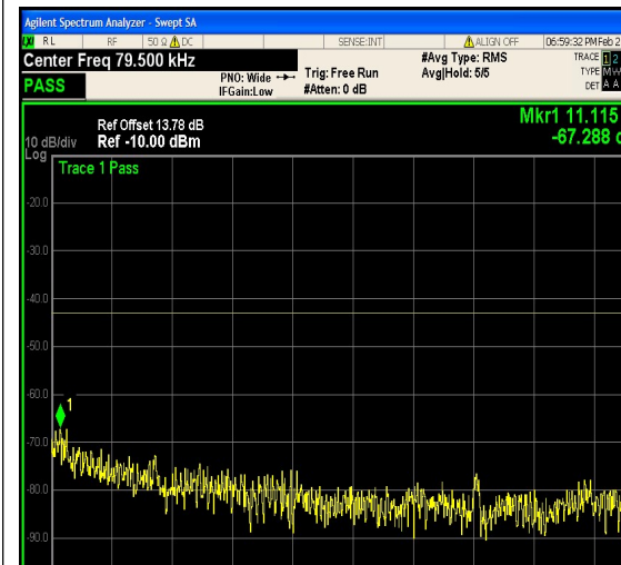
1-N66-PC3-15-10-H-9-DFT-16QAM-Outer_F ull-50@0-0.009-0.15-Ant1--67.29--43-PASS
