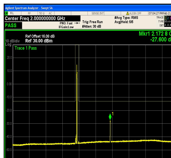
1-N66-PC3-15-10-H-12-DFT-64QAM-Outer_ Full-50@0-0.15-30-Ant1--63.58--33-PASS
