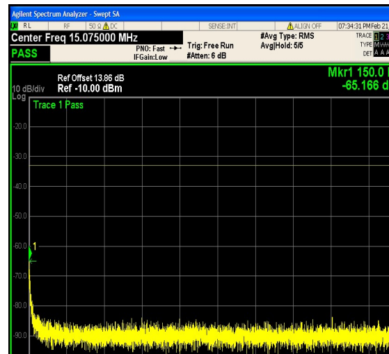
1-N66-PC3-15-15-L-5-DFT-QPSK-Edge_1RB _Right-1@78-0.15-30-Ant1--65.17--33-PASS
