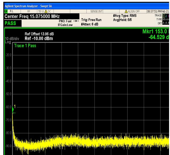
1-N66-PC3-15-15-M-21-CP-16QAM-Outer_F ull-79@0-0.15-30-Ant1--64.53--33-PASS
