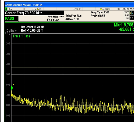
1-N66-PC3-15-15-M-24-CP-64QAM-Outer_F ull-79@0-0.009-0.15-Ant1--65.66--43-PASS
