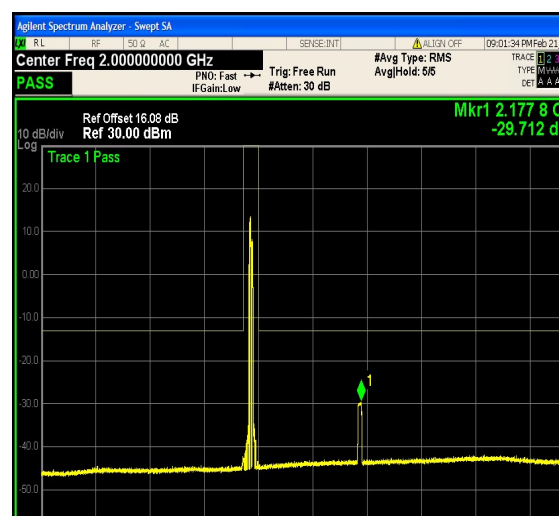
1-N66-PC3-15-15-H-9-DFT-16QAM-Outer_F ull-75@0-0.15-30-Ant1--63.49--33-PASS
