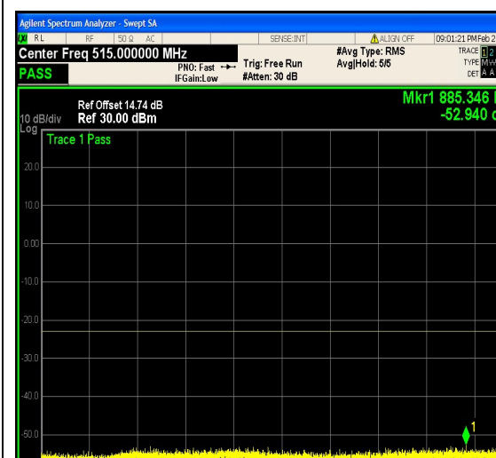
1-N66-PC3-15-15-H-9-DFT-16QAM-Outer_F ull-75@0-0.009-0.15-Ant1--67.61--43-PASS
