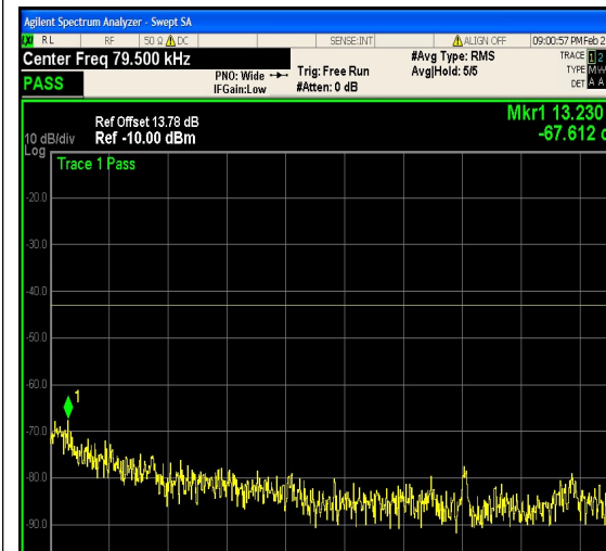
1-N66-PC3-15-15-H-9-DFT-16QAM-Outer_F ull-75@0-0.009-0.15-Ant1--67.61--43-PASS
