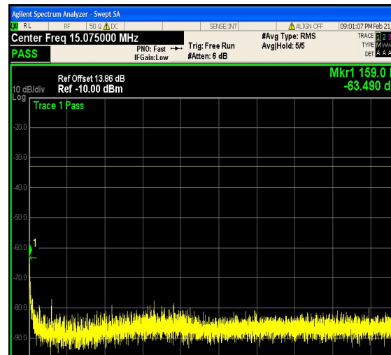
1-N66-PC3-15-15-H-9-DFT-16QAM-Outer_F ull-75@0-0.15-30-Ant1--63.49--33-PASS
