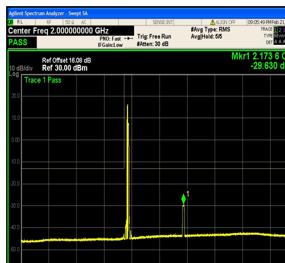
1-N66-PC3-15-15-H-12-DFT-64QAM-Outer_ Full-75@0-0.15-30-Ant1--64.54--33-PASS
