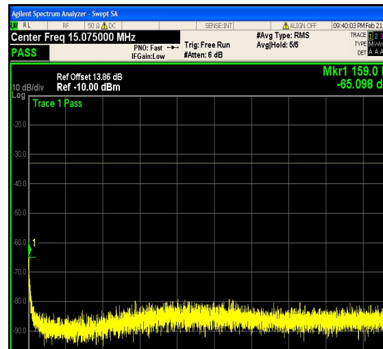
1-N66-PC3-15-20-L-8-DFT-16QAM-Edge_1R B_Right-1@105-0.15-30-Ant1--65.10--33-PA SS
