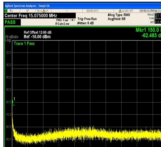
1-N66-PC3-15-20-L-21-CP-16QAM-Outer_F ull-106@0-0.15-30-Ant1--62.48--33-PASS
