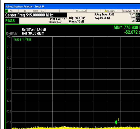
1-N66-PC3-15-20-H-9-DFT-16QAM-Outer_F ull-100@0-0.009-0.15-Ant1--65.18--43-PASS
