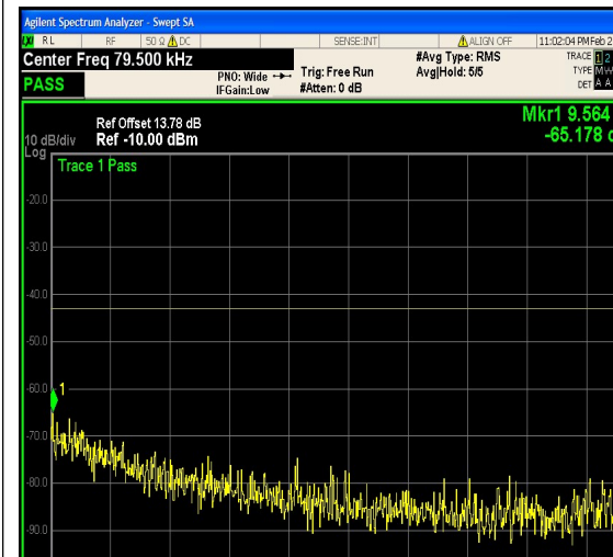
1-N66-PC3-15-20-H-9-DFT-16QAM-Outer_F ull-100@0-0.009-0.15-Ant1--65.18--43-PASS
