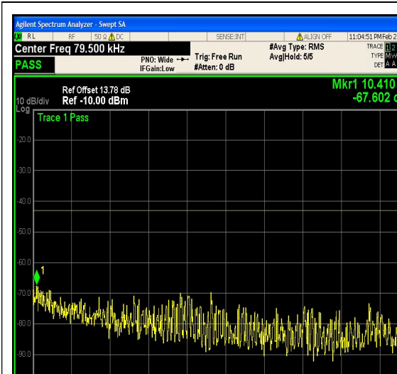
1-N66-PC3-15-20-H-11-DFT-64QAM-Edge_1 RB_Right-1@105-0.009-0.15-Ant1--67.60--4 3-PASS
