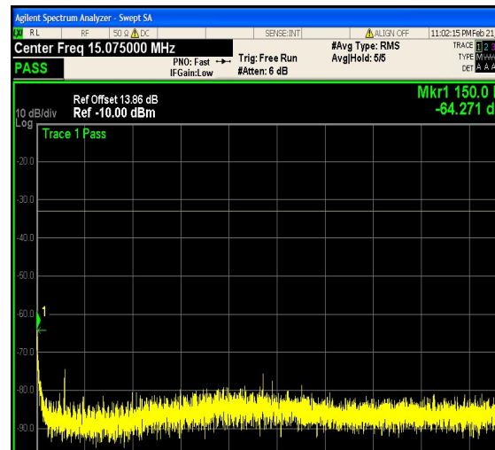
1-N66-PC3-15-20-H-9-DFT-16QAM-Outer_F ull-100@0-0.15-30-Ant1--64.27--33-PASS
