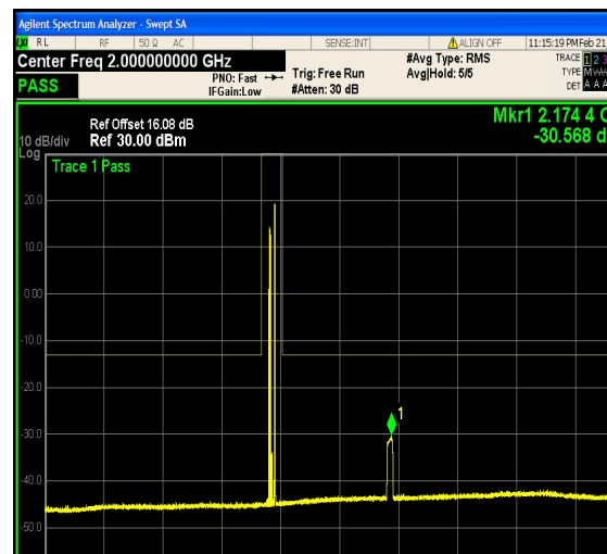
1-N66-PC3-15-20-H-18-CP-QPSK-Outer_Ful I-106@0-0.15-30-Ant1--64.77--33-PASS
