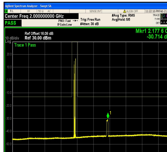
1-N66-PC3-15-20-H-23-CP-64QAM-Edge_1 RB_Right-1@105-1000-3000-Ant1--30.71--1 3-PASS
