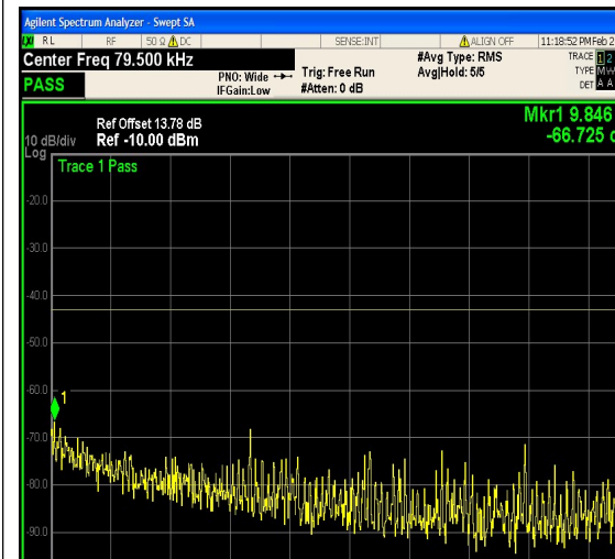
1-N66-PC3-15-20-H-21-CP-16QAM-Outer_F ull-106@0-0.009-0.15-Ant1--66.72--43-PASS
