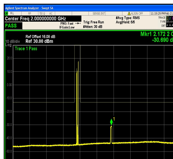
1-N66-PC3-15-20-H-21-CP-16QAM-Outer_F ull-106@0-0.15-30-Ant1--66.14--33-PASS
