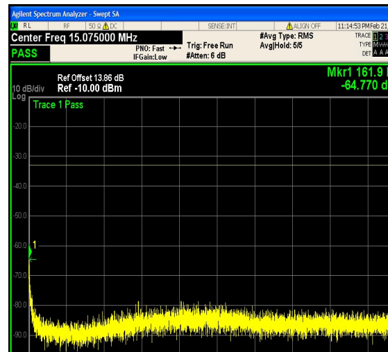
1-N66-PC3-15-20-H-18-CP-QPSK-Outer_Ful I-106@0-0.15-30-Ant1--64.77--33-PASS
