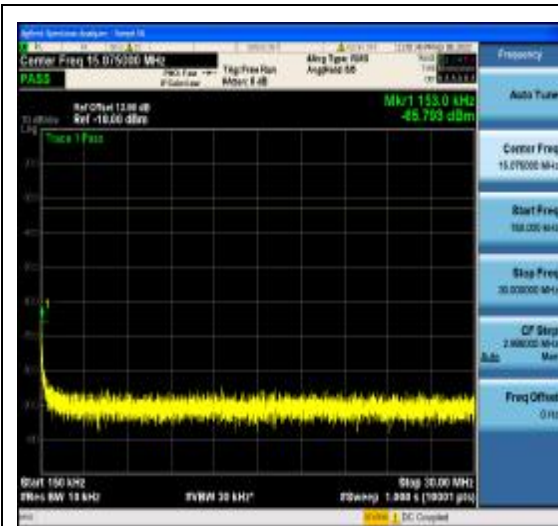
1-N77-3700-3980-PC2-30-40-M-14-DFT-256 QAM-Edge_1RB_Right-1@105-0.15-30-Ant1 --65.79--33-PASS
