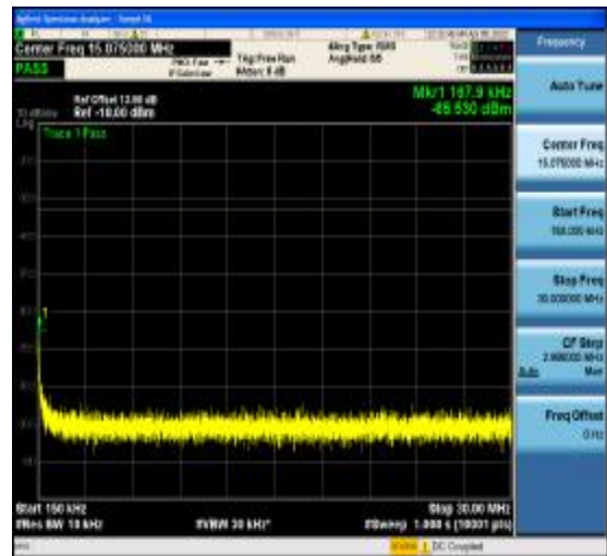
1-N77-3700-3980-PC2-30-40-H-8-DFT-16QA M-Edge_1RB_Right-1@105-0.15-30-Ant1--6 5.53--33-PASS
