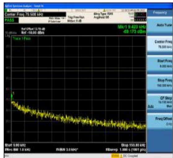
1-N77-3700-3980-PC2-30-40-H-11-DFT-64Q AM-Edge_1RB_Right-1@105-0.009-0.15-Ant 1--69.17--43-PASS
