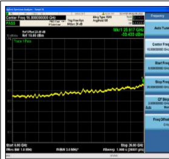
1-N77-3700-3980-PC2-30-60-H-26-CP-256Q AM-Edge_1RB_Right-1@161-6000-26000-A nt1--33.43--13-PASS
