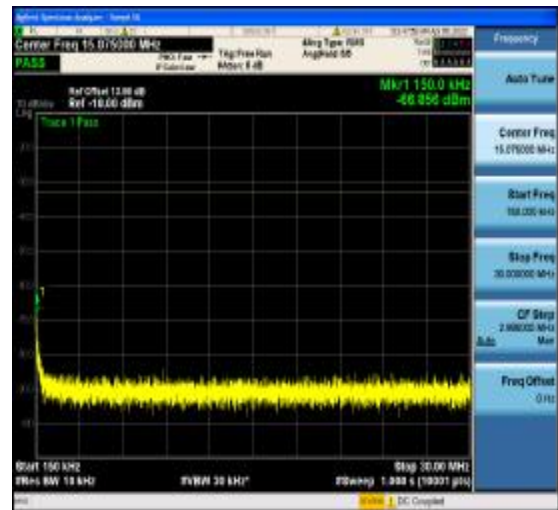
1-N77-3700-3980-PC2-30-60-H-27-CP-256Q AM-Outer_Full-162@0-0.15-30-Ant1--66.86-- 33-PASS
