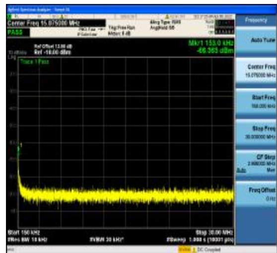
1-N77-3700-3980-PC2-30-60-H-11-DFT-64Q AM-Edge_1RB_Right-1@161-0.15-30-Ant1-- 66.36--33-PASS
