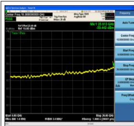
1-N77-3700-3980-PC2-30-60-H-10-DFT-64Q AM-Edge_1RB_Left-1@0-6000-26000-Ant1-- 33.44--13-PASS
