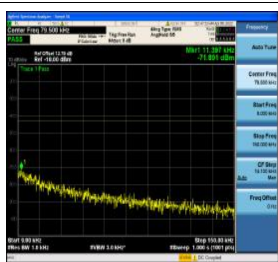
1-N77-3700-3980-PC2-30-60-M-23-CP-64Q AM-Edge_1RB_Right-1@161-0.009-0.15-Ant 1--71.89--43-PASS
