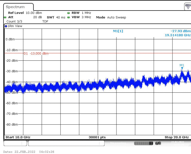
Band2-9262-4-10000~20000MHz
