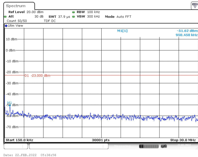
Band2-9538-1-0.15~30MHz
