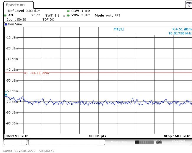
Band2-9538-1-0.009~0.15MHz
