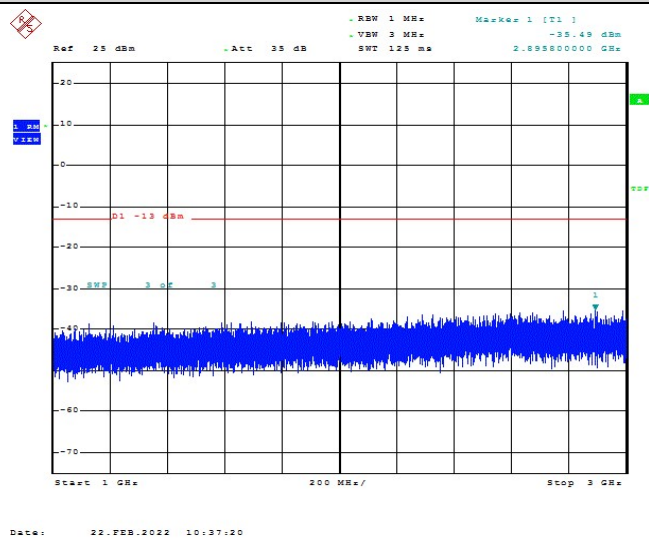
Band5-4132-3-1000~3000MHz
