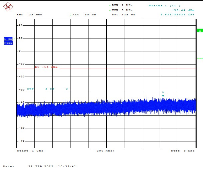
Band5-4132-1-1000~3000MHz
