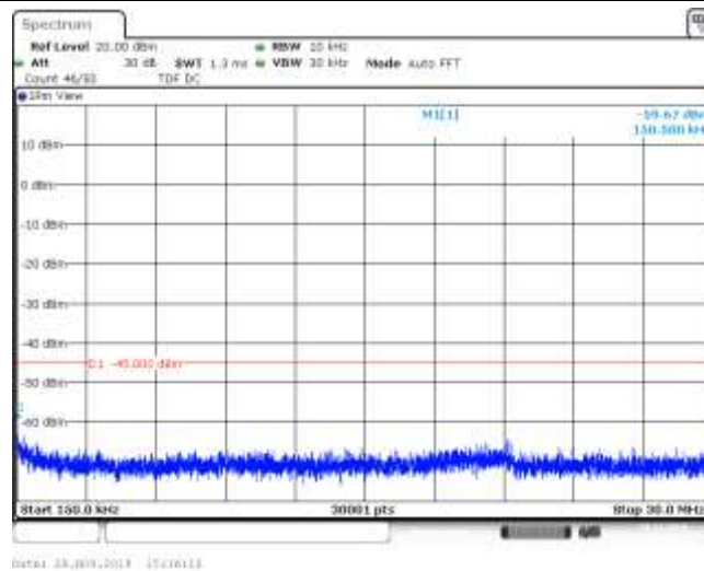
Band41_20MHz_QPSK_41140_1RB#0
