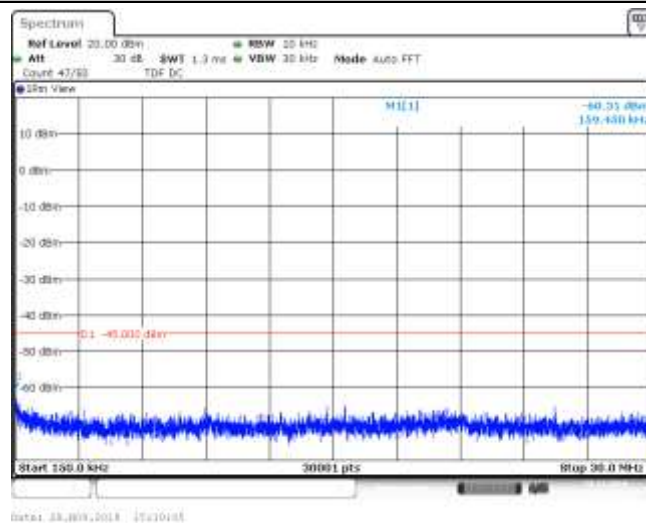
Band41_20MHz_16QAM_41140_1RB#0
