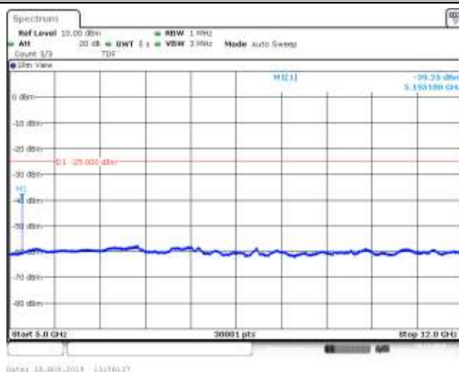
Band41_5MHz_QPSK_40690_1RB#0
