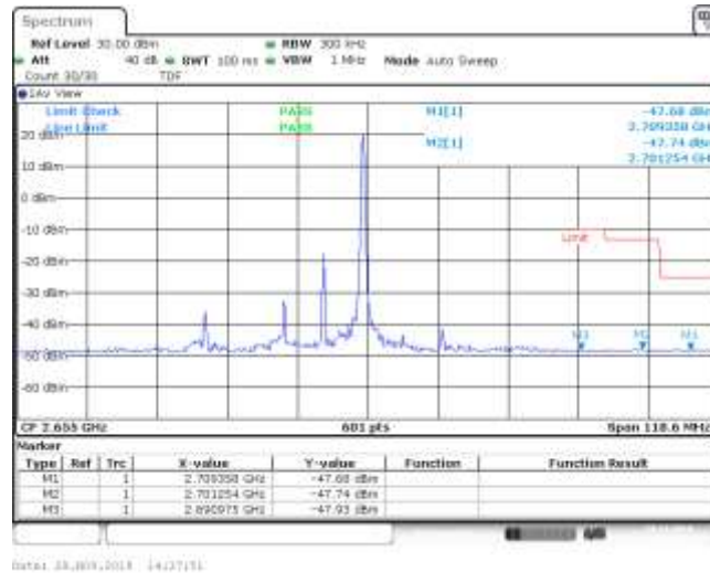
Band41_15MHz_QPSK_41165_75RB#0
