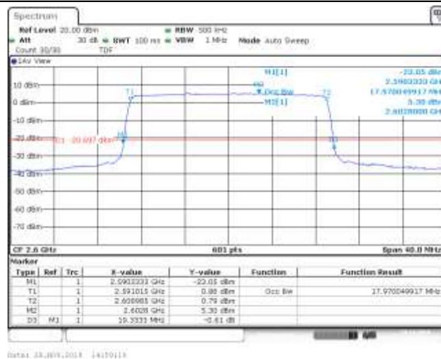
Band41_20MHz_QPSK_40690_100RB#0
