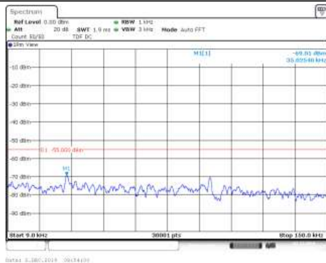
Band41_10MHz_16QAM_40290_1RB#0
