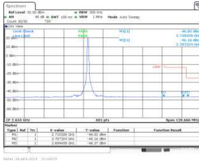
Band41_20MHz_QPSK_41140_1RB#99
