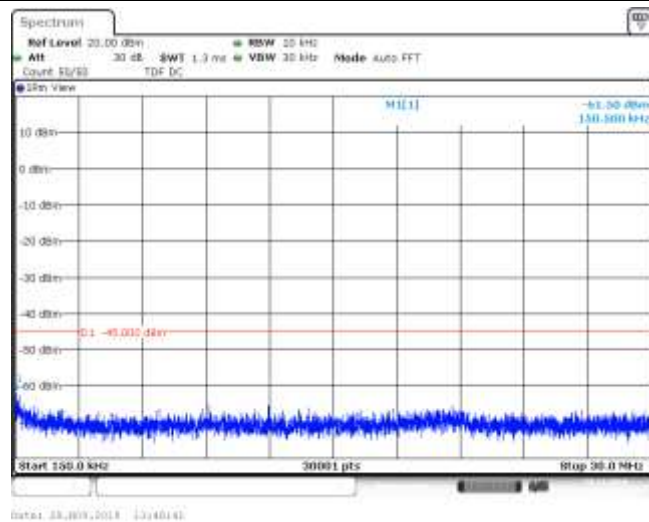
Band41_5MHz_QPSK_40265_1RB#0
