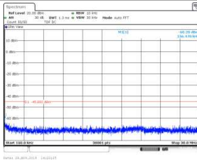
Band41_10MHz_16QAM_40690_1RB#0
