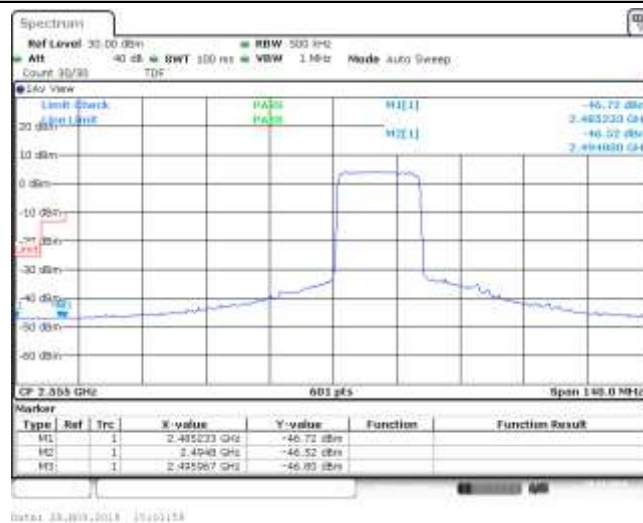
Band41_20MHz_16QAM_40340_100RB#0
