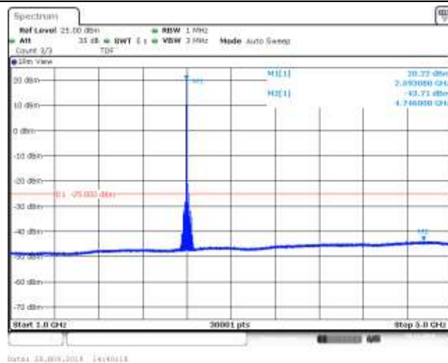
Band41_15MHz_16QAM_40690_1RB#0
