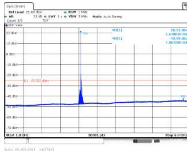
Band41_15MHz_16QAM_41165_1RB#0
