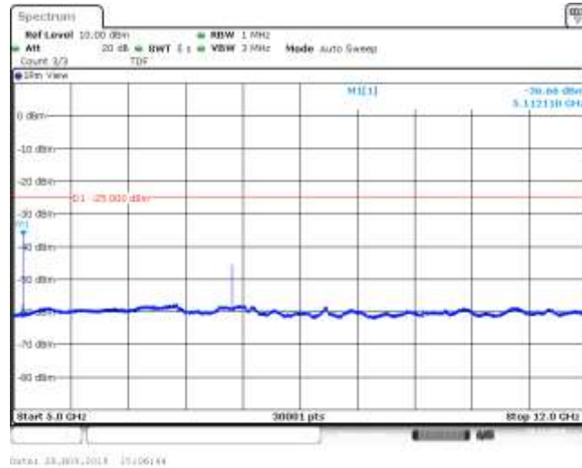
Band41_20MHz_QPSK_40340_1RB#0
