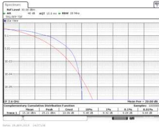
Band41_15MHz_16QAM_41165_1RB#0
