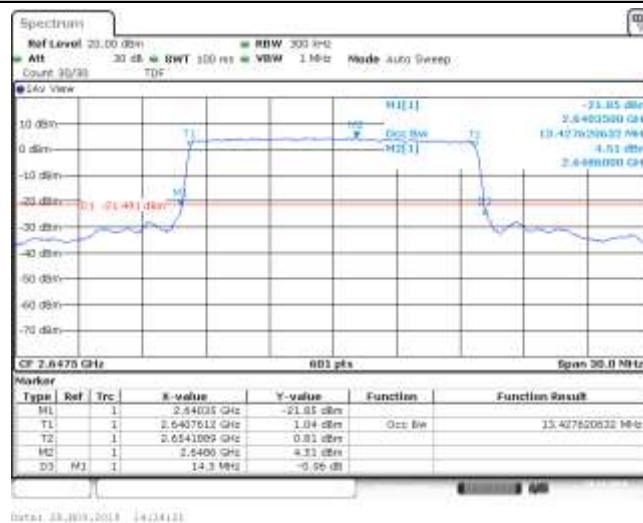
Band41_15MHz_QPSK_41165_75RB#0
