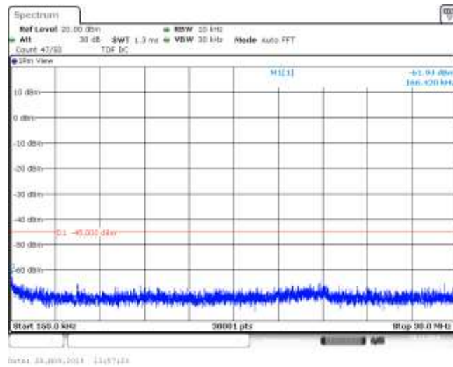
Band41_5MHz_16QAM_40690_1RB#0
