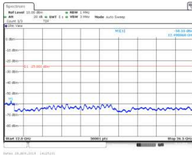
Band41_10MHz_16QAM_41190_1RB#0
