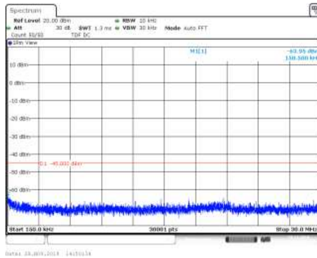
Band41_15MHz_QPSK_41165_1RB#0
