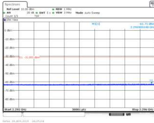
Band30_5MHz_16QAM_27710_1RB#0
