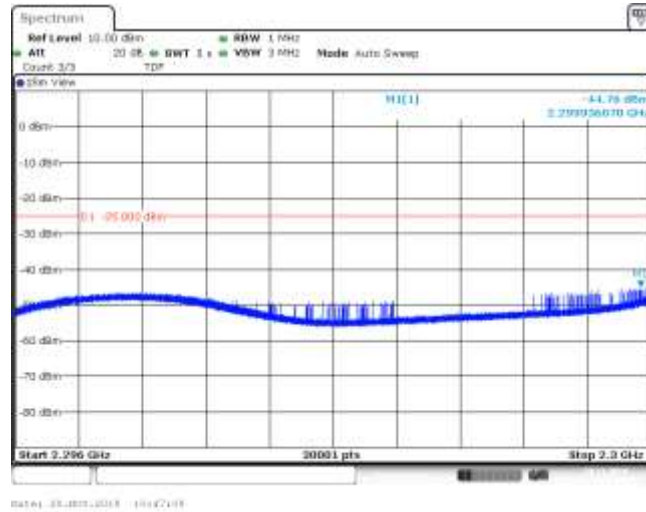
Band30_5MHz_16QAM_27685_1RB#0
