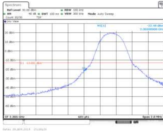
Band30_5MHz_16QAM_27685_1RB#12
