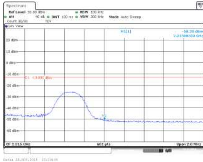
Band30_5MHz_16QAM_27735_1RB#12
