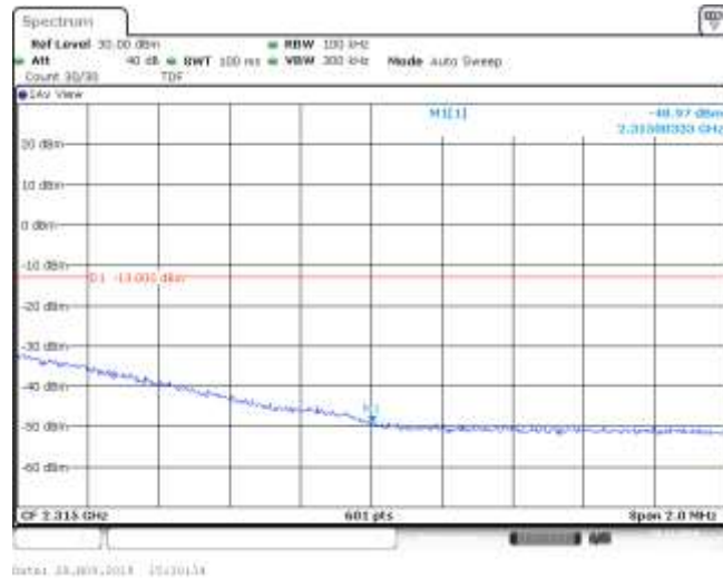
Band30_5MHz_16QAM_27735_1RB#24
