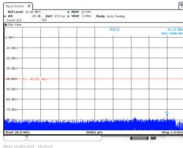
Band30_5MHz_QPSK_27685_1RB#0
