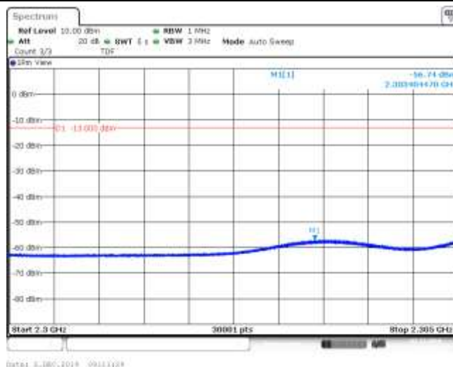
Band30_5MHz_QPSK_27710_1RB#0
