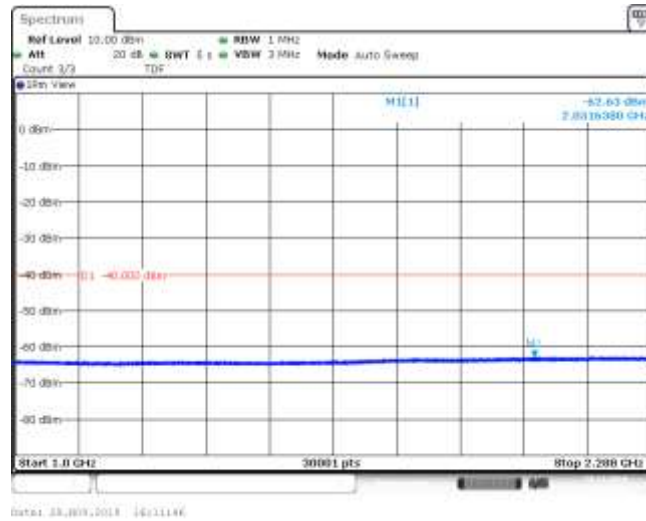
Band30_5MHz_16QAM_27685_1RB#0
