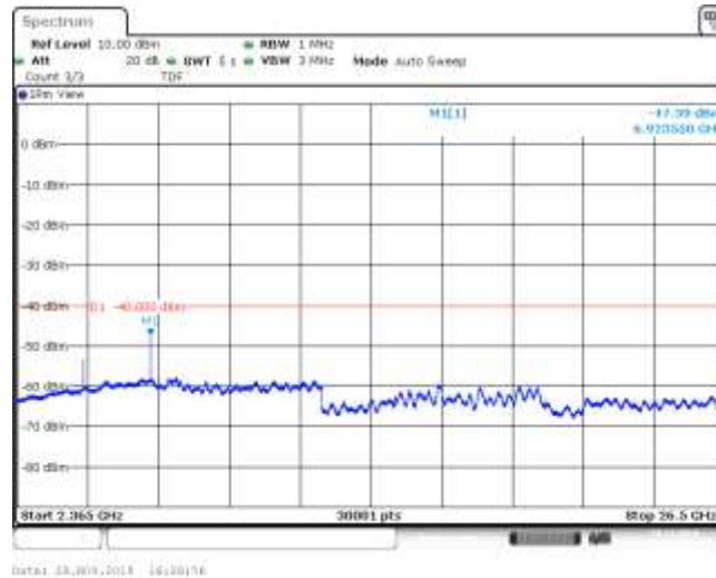
Band30_5MHz_16QAM_27735_1RB#0
