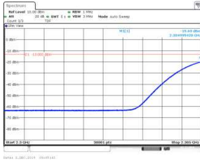
Band30_5MHz_QPSK_27685_1RB#0
