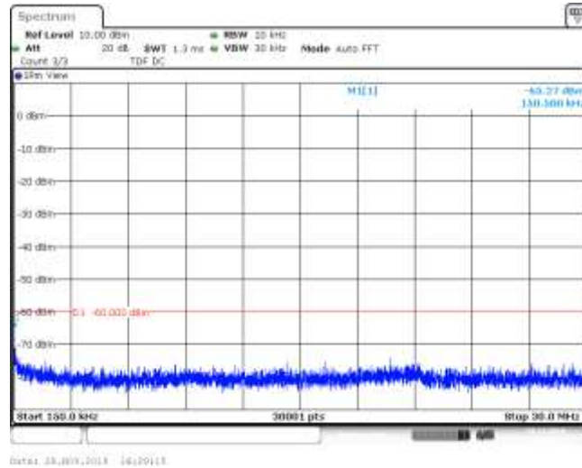
Band30_5MHz_QPSK_27735_1RB#0
