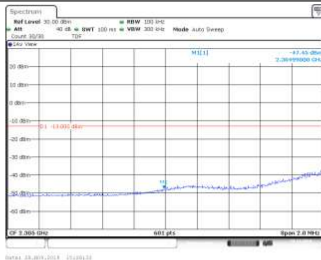
Band30_5MHz_QPSK_27685_1RB#24
