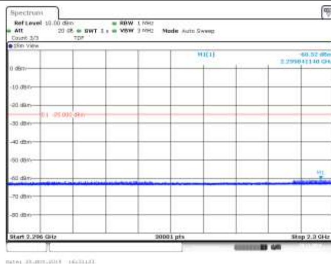
Band30_10MHz_16QAM_27710_1RB#0
