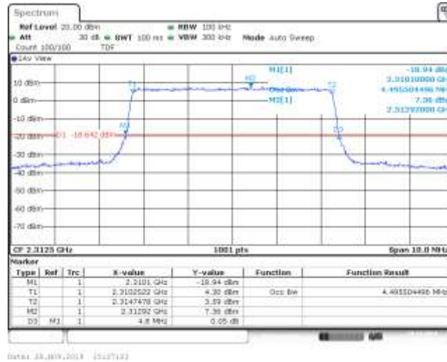
Band30_5MHz_16QAM_27685_25RB#0
