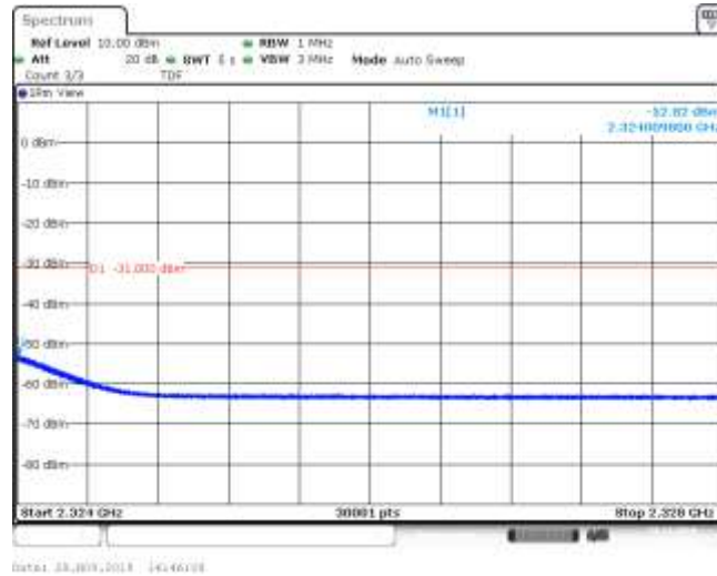
Band30_10MHz_QPSK_27710_1RB#0
