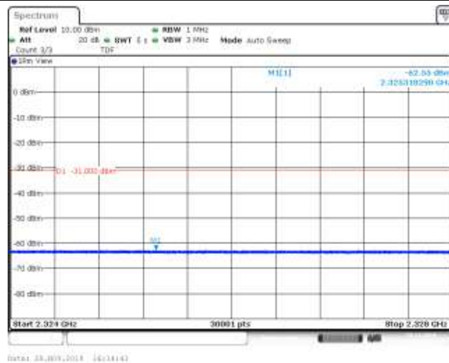
Band30_5MHz_16QAM_27685_1RB#0
