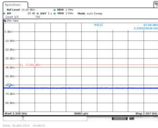
Band30_10MHz_QPSK_27710_1RB#0
