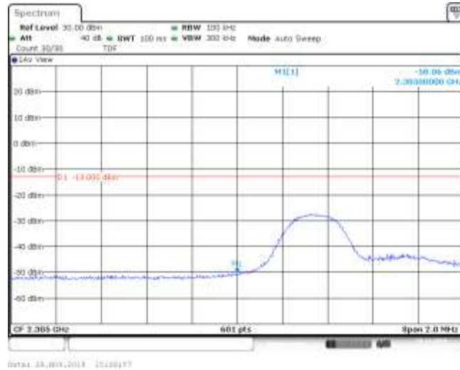
Band30_5MHz_QPSK_27685_25RB#0
