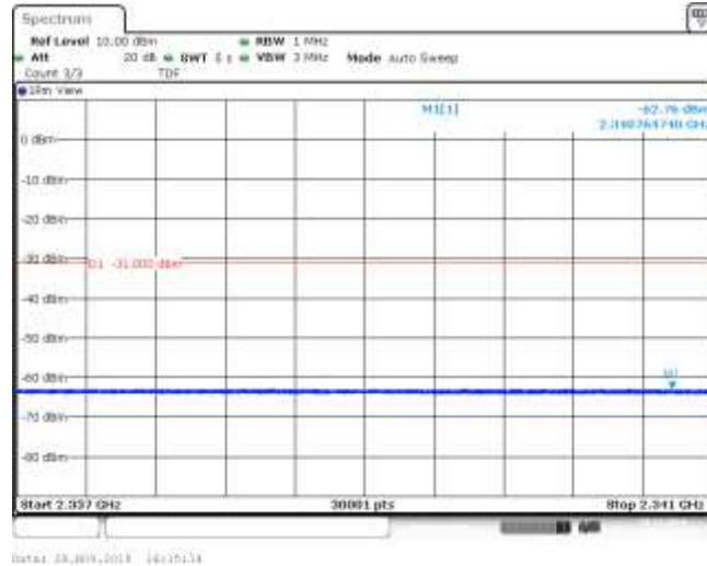
Band30_5MHz_16QAM_27685_1RB#0
