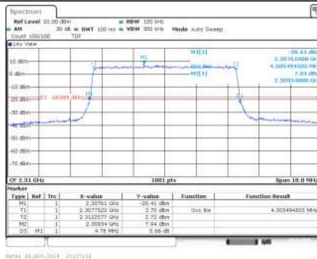
Band30_5MHz_16QAM_27710_25RB#0
