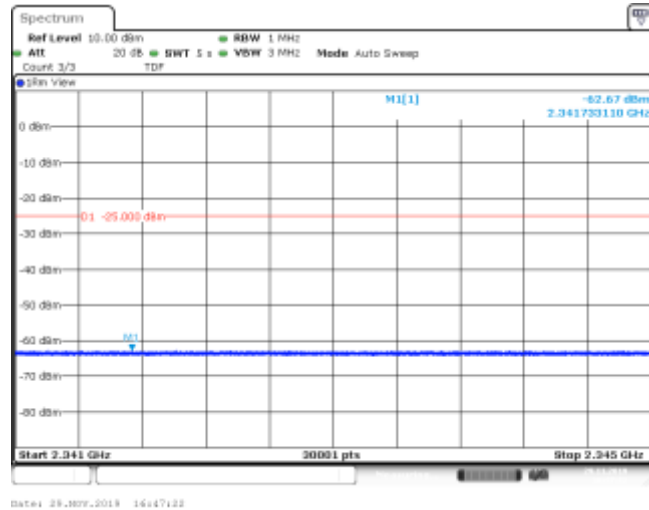
Band30_5MHz_QPSK_27710_1RB#0
