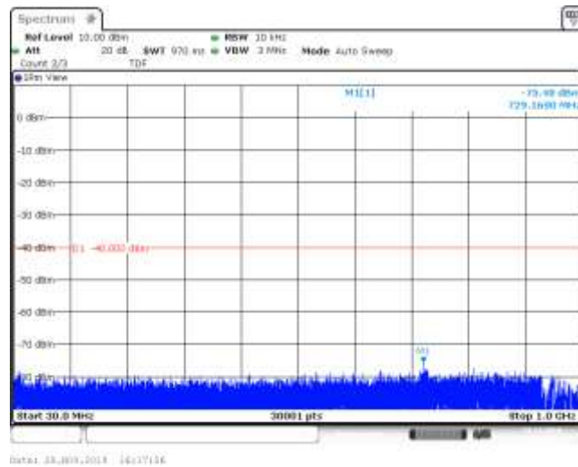
Band30_5MHz_QPSK_27710_1RB#0
