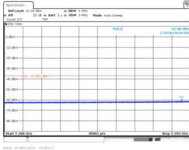
Band30_10MHz_16QAM_27710_1RB#0
