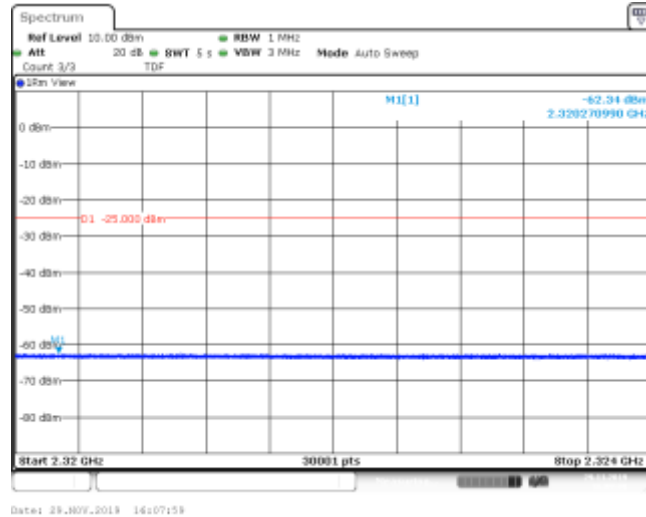
Band30_5MHz_QPSK_27685_1RB#0
