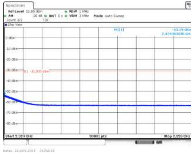
Band30_10MHz_16QAM_27710_1RB#0
