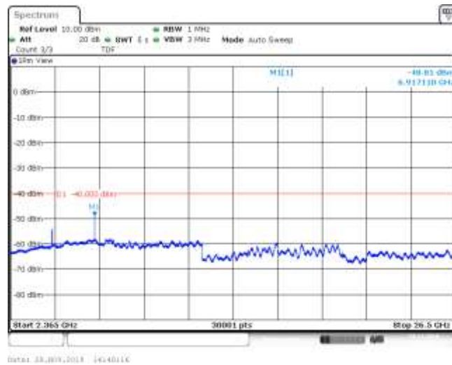
Band30_10MHz_16QAM_27710_1RB#0
