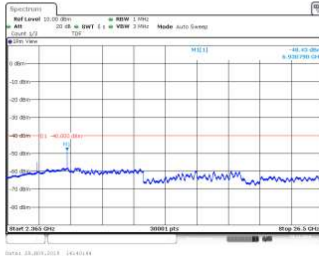
Band30_10MHz_QPSK_27710_1RB#0
