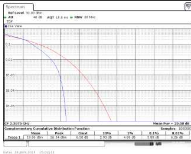
Band30_5MHz_16QAM_27710_1RB#0
