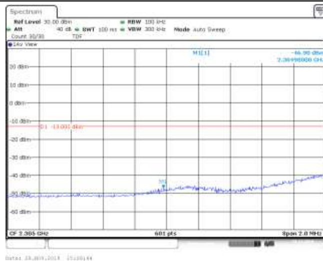
Band30_5MHz_16QAM_27685_1RB#12
