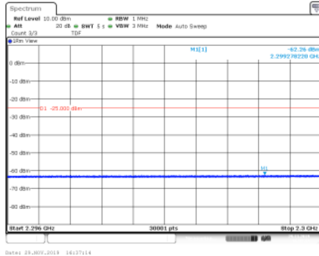
Band30_5MHz_16QAM_27735_1RB#0
