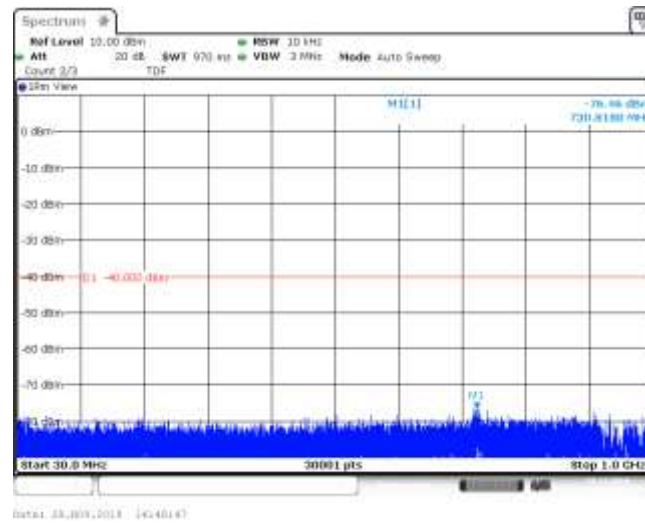
Band30_10MHz_16QAM_27710_1RB#0
