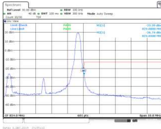
Band26_5MHz_QPSK_26765_25RB#0
