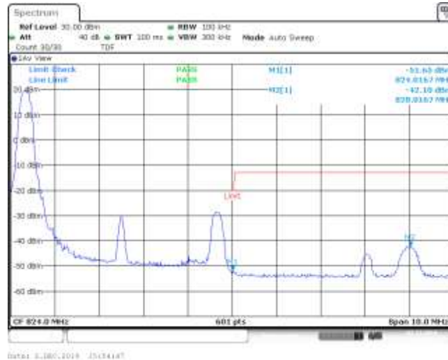
Band26_5MHz_QPSK_26765_1RB#24
