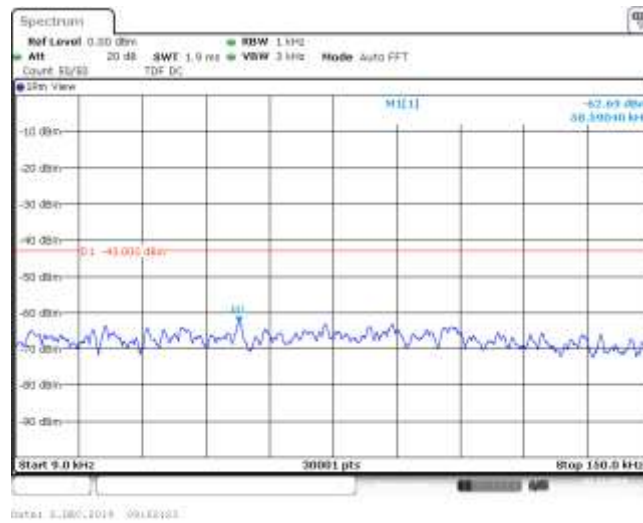
Band26_5MHz_16QAM_26715_1RB#0
