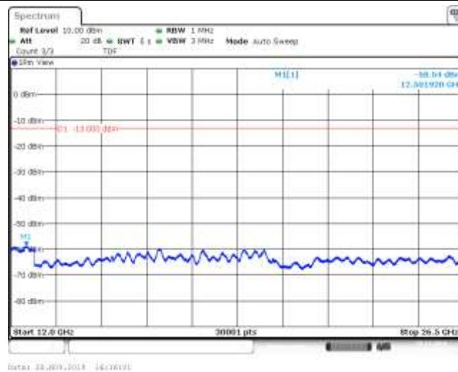
Band26_5MHz_QPSK_26715_1RB#0
