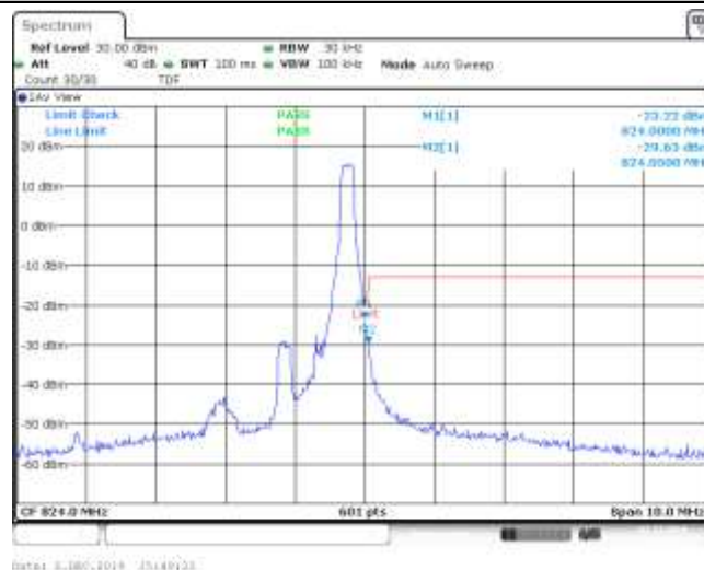
Band26_1.4MHz_QPSK_26783_1RB#5
