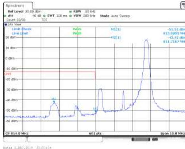
Band26_3MHz_QPSK_26705_15RB#0
