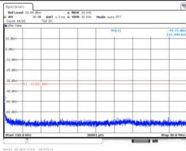
Band26_10MHz_QPSK_26740_1RB#0
