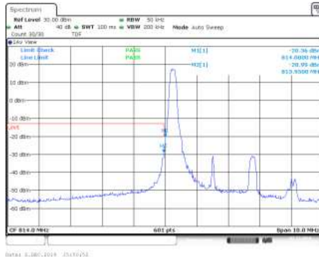
Band26_3MHz_16QAM_26705_1RB#14
