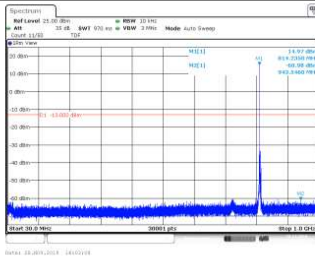
Band26_3MHz_16QAM_26705_1RB#0
