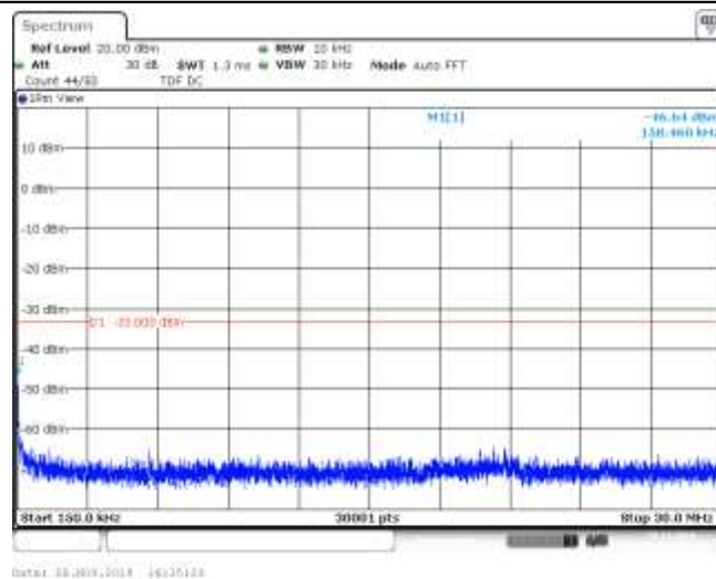
Band26_5MHz_QPSK_26740_1RB#0
