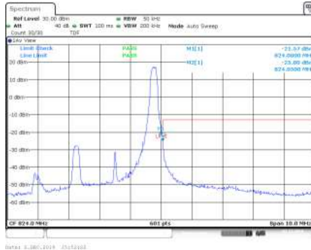
Band26_3MHz_16QAM_26775_15RB#0
