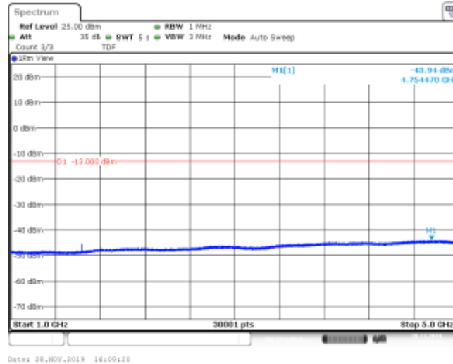
Band26_3MHz_16QAM_26740_1RB#0
