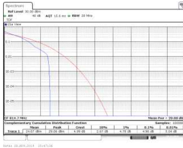
Band26_1.4MHz_QPSK_26697_6RB#0
