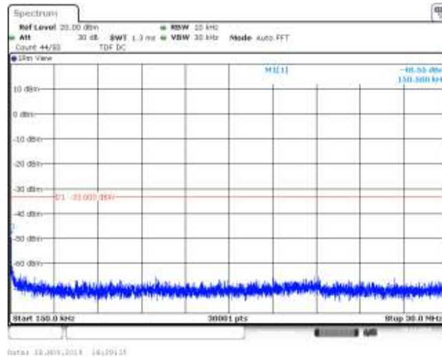
Band26_5MHz_QPSK_26715_1RB#0
