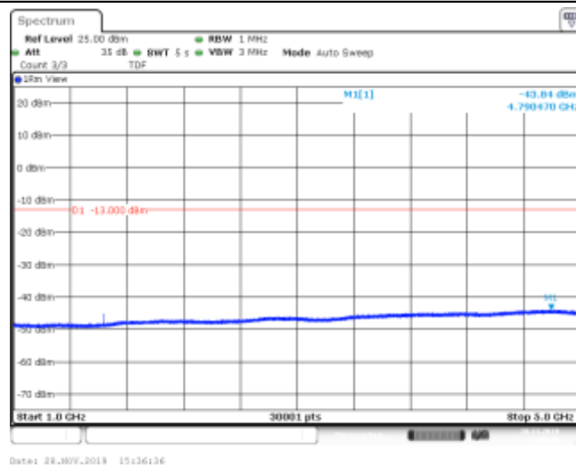
Band26_1.4MHz_QPSK_26740_1RB#0
