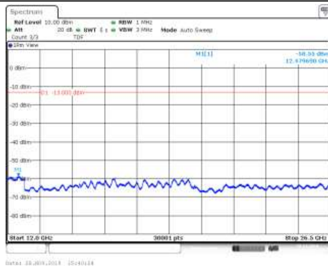
Band26_1.4MHz_16QAM_26740_1RB#0
