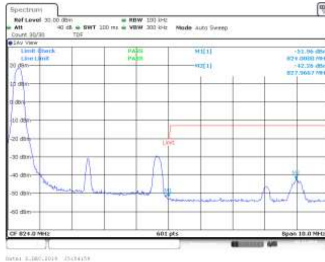
Band26_5MHz_16QAM_26765_1RB#24
