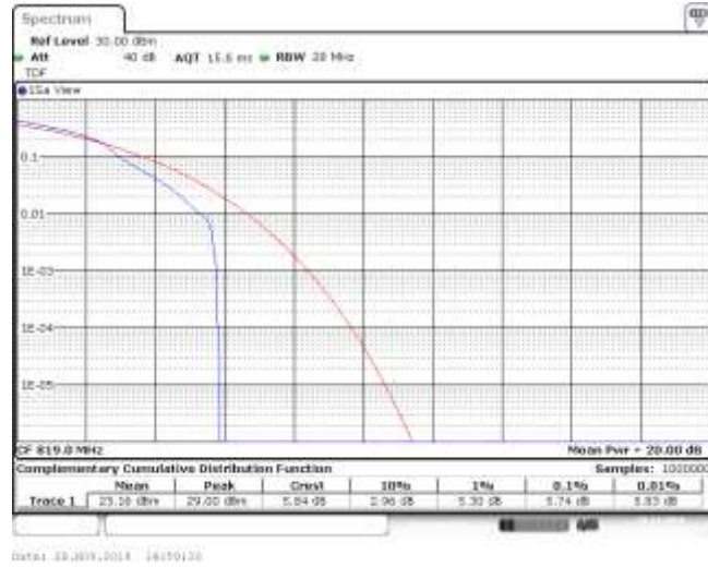
Band26_10MHz_16QAM_26740_50RB#0
