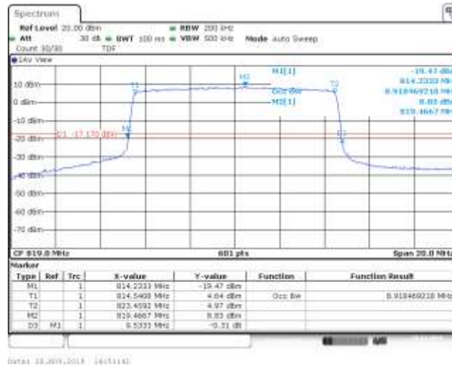
Band26_10MHz_16QAM_26740_50RB#0
