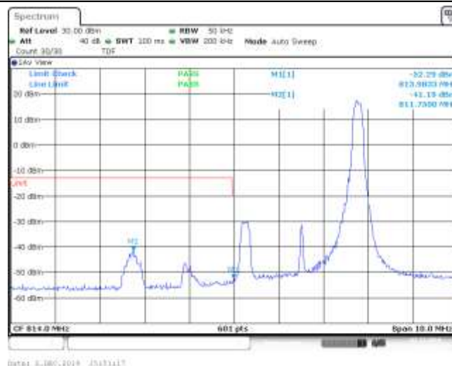
Band26_3MHz_16QAM_26705_1RB#14
