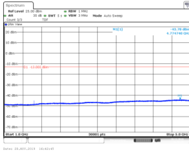
Band26_5MHz_QPSK_26765_1RB#0
