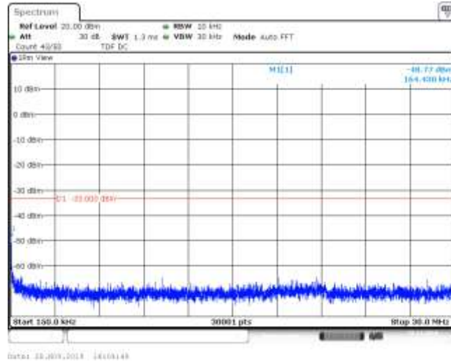
Band26_3MHz_QPSK_26740_1RB#0
