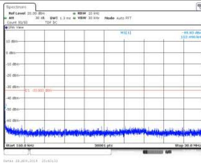
Band26_1.4MHz_16QAM_26783_1RB#0
