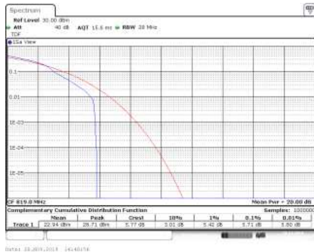
Band26_5MHz_16QAM_26740_25RB#0
