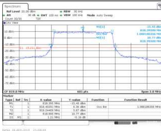
Band26_1.4MHz_16QAM_26740_6RB#0
