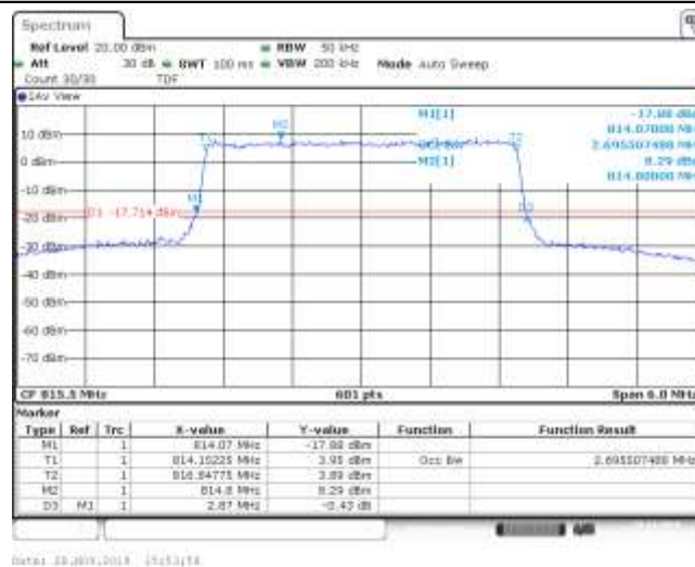
Band26_3MHz_16QAM_26705_15RB#0
