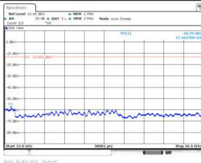
Band26_5MHz_16QAM_26765_1RB#0
