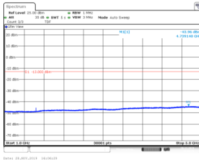
Band26_3MHz_QPSK_26740_1RB#0
