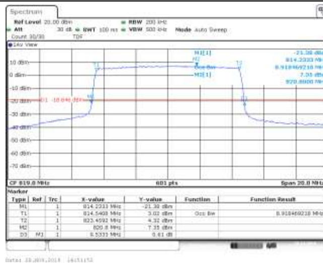
Band26_10MHz_16QAM_26740_50RB#0
