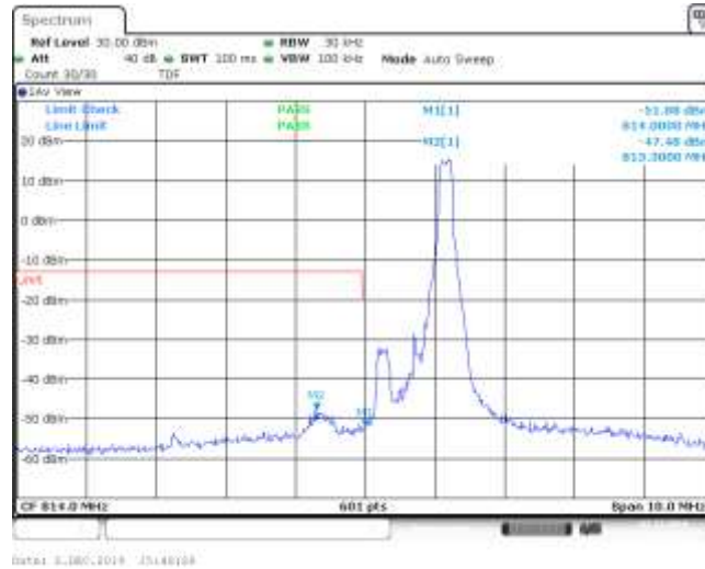
Band26_1.4MHz_16QAM_26697_6RB#0
