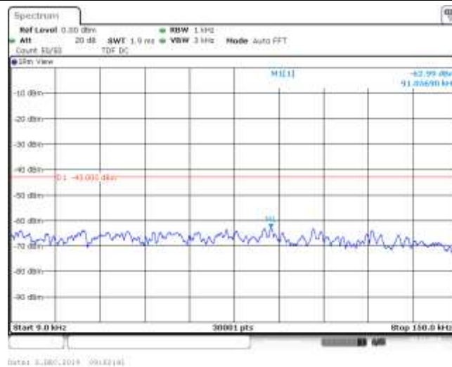
Band26_5MHz_16QAM_26740_1RB#0
