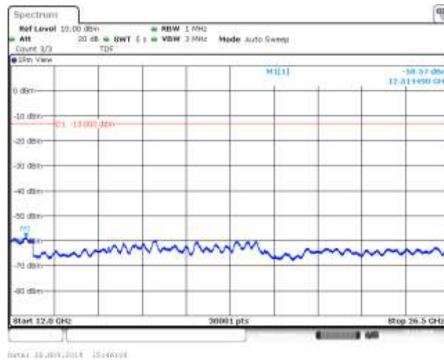
Band26_3MHz_QPSK_26705_1RB#0
