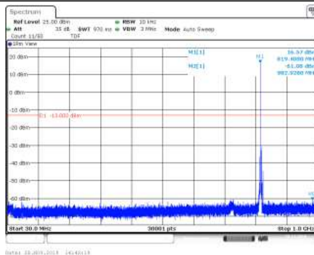
Band26_5MHz_QPSK_26765_1RB#0
