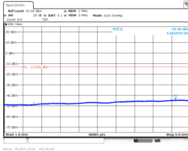
Band26_5MHz_16QAM_26715_1RB#0
