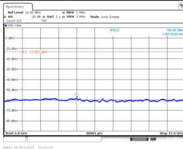
Band26_1.4MHz_QPSK_26697_1RB#0
