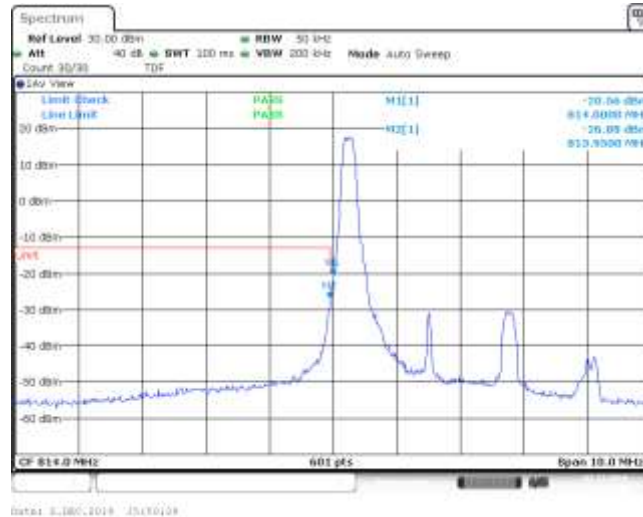
Band26_3MHz_QPSK_26705_1RB#14
