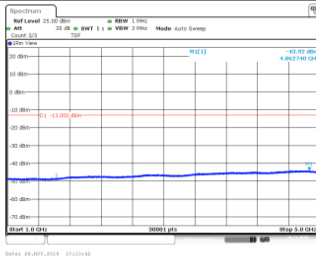
Band26_1.4MHz_16QAM_26697_1RB#0
