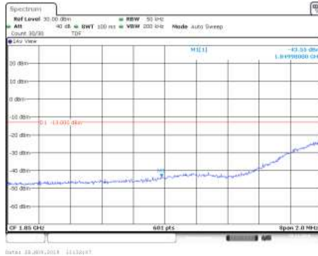
Band25_3MHz_QPSK_26055_1RB#14
