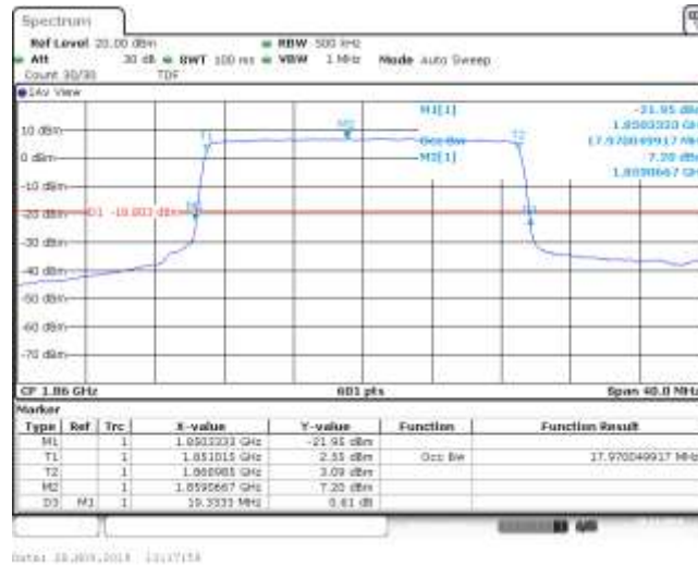
Band25_20MHz_QPSK_26365_100RB#0
