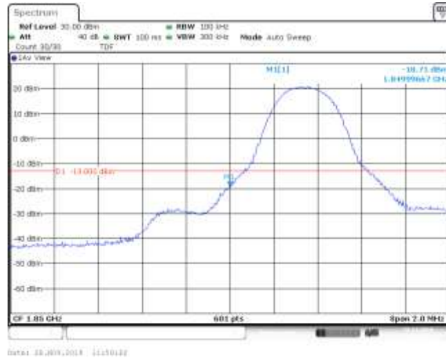
Band25_5MHz_QPSK_26065_1RB#12
