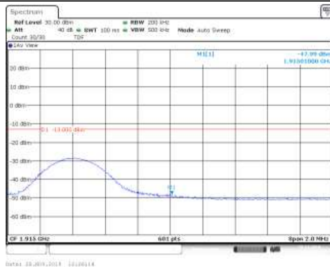
Band25_10MHz_QPSK_26640_1RB#24
