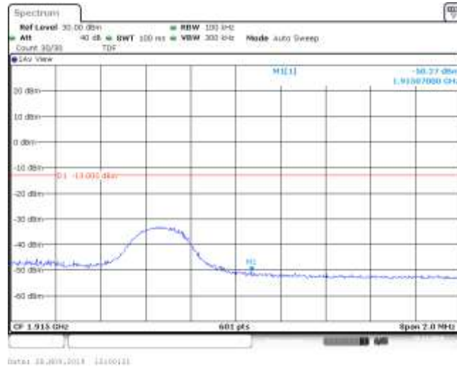
Band25_5MHz_16QAM_26665_1RB#12
