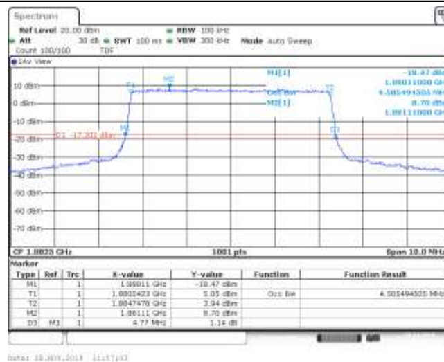
Band25_5MHz_QPSK_26665_25RB#0
