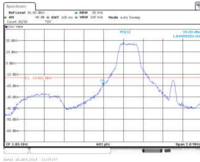
Band25_1.4MHz_QPSK_26047_1RB#2
