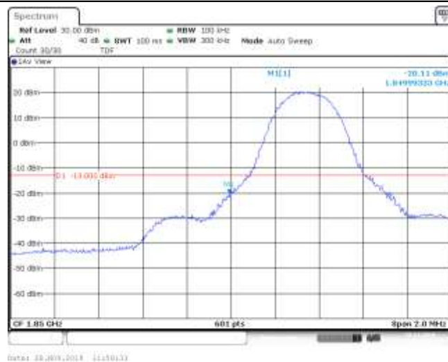
Band25_5MHz_16QAM_26065_1RB#12
