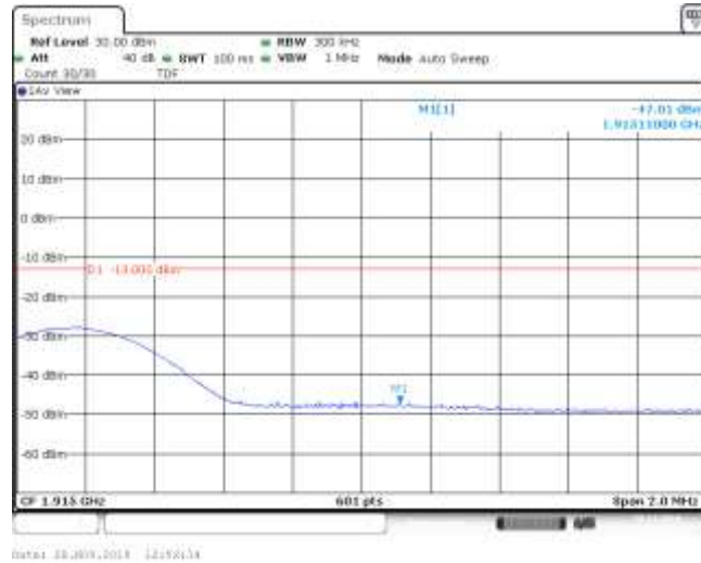
Band25_15MHz_QPSK_26615_1RB#38
