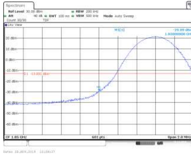
Band25_10MHz_16QAM_26090_1RB#24
