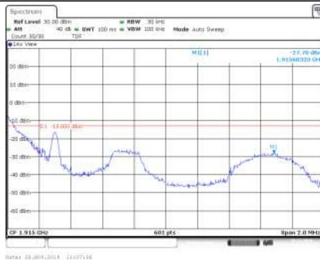
Band25_1.4MHz_QPSK_26683_1RB#2
