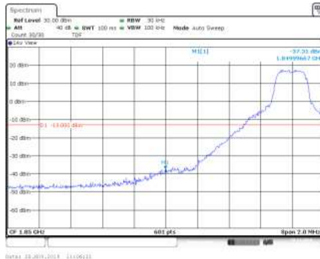
Band25_1.4MHz_QPSK_26047_1RB#5
