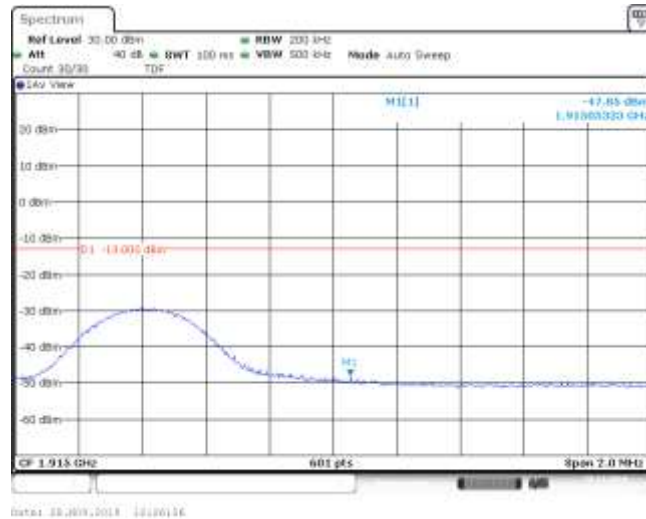
Band25_10MHz_16QAM_26640_1RB#24
