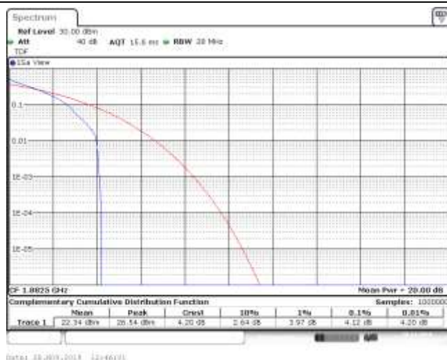
Band25_10MHz_QPSK_26365_50RB#0
