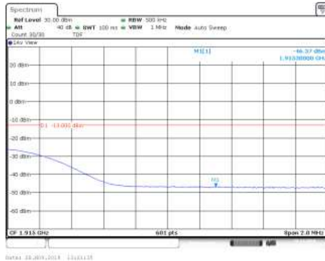
Band25_20MHz_QPSK_26590_1RB#49
