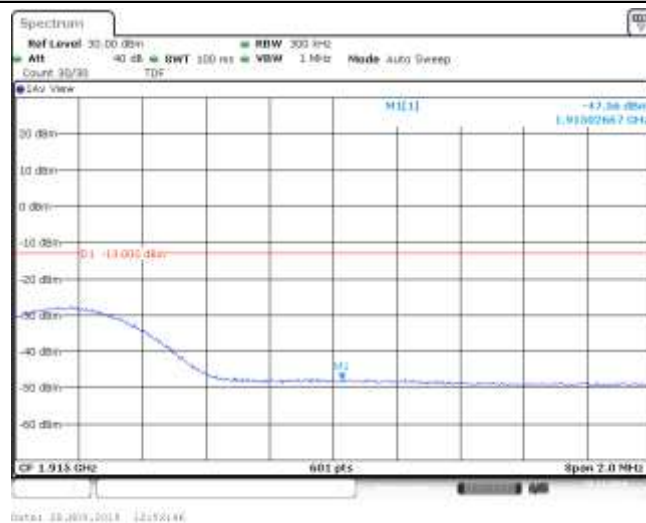
Band25_15MHz_16QAM_26615_1RB#38
