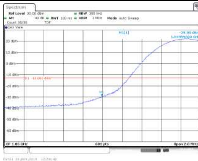
Band25_15MHz_QPSK_26115_1RB#38
