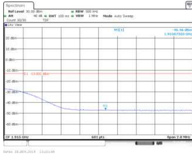
Band25_20MHz_16QAM_26590_1RB#49
