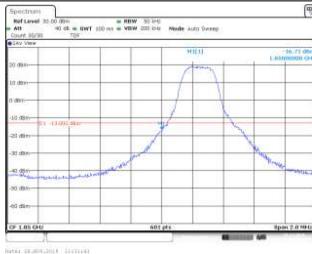
Band25_3MHz_QPSK_26055_1RB#8
