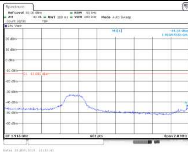
Band25_3MHz_16QAM_26675_1RB#8
