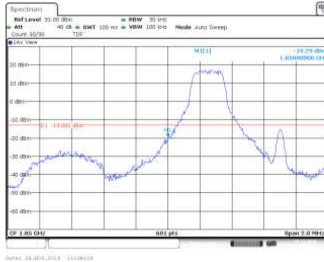
Band25_1.4MHz_16QAM_26047_1RB#2
