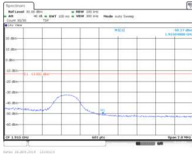
Band25_5MHz_QPSK_26665_1RB#12
