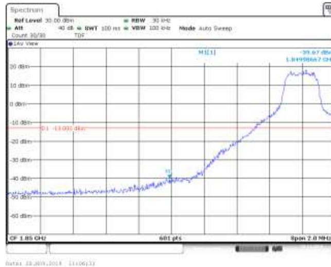
Band25_1.4MHz_16QAM_26047_1RB#5
