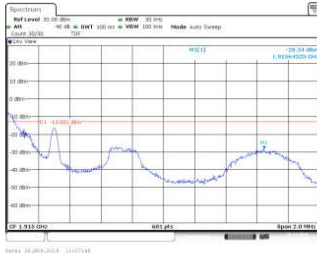
Band25_1.4MHz_16QAM_26683_1RB#2
