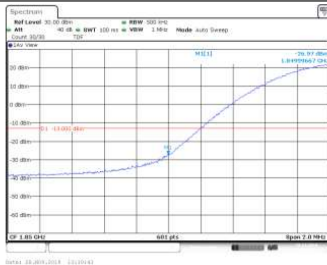
Band25_20MHz_16QAM_26140_1RB#49
