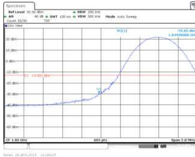
Band25_10MHz_QPSK_26090_1RB#24
