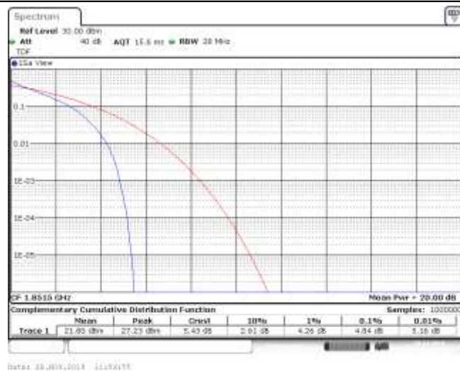
Band25_3MHz_QPSK_26365_1RB#0
