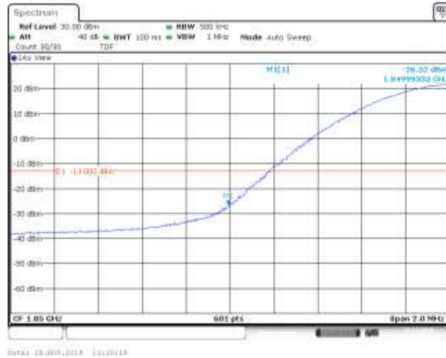
Band25_20MHz_QPSK_26140_1RB#49
