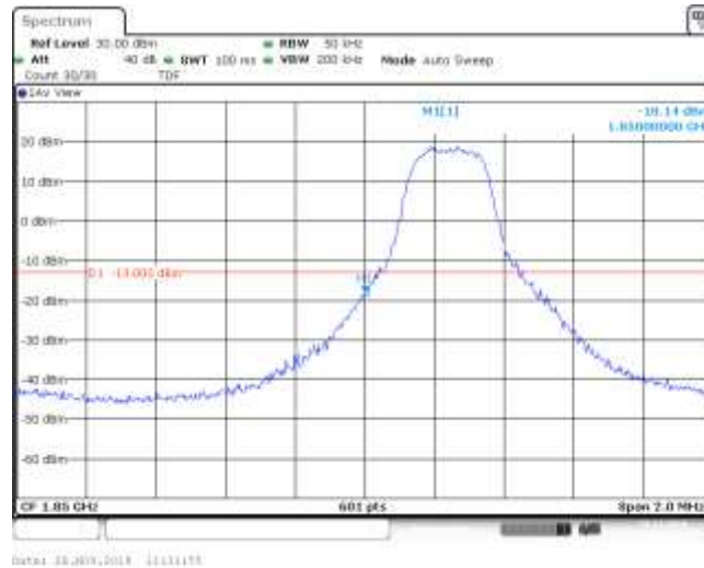
Band25_3MHz_16QAM_26055_1RB#8
