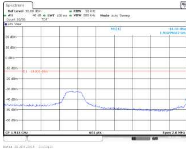
Band25_3MHz_QPSK_26675_1RB#8
