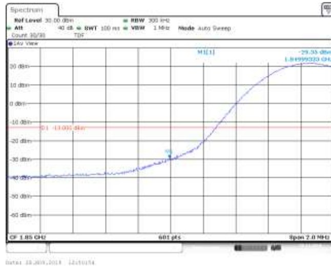
Band25_15MHz_16QAM_26115_1RB#38
