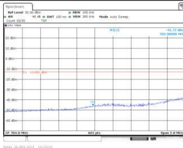
Band17_5MHz_16QAM_23755_1RB#12
