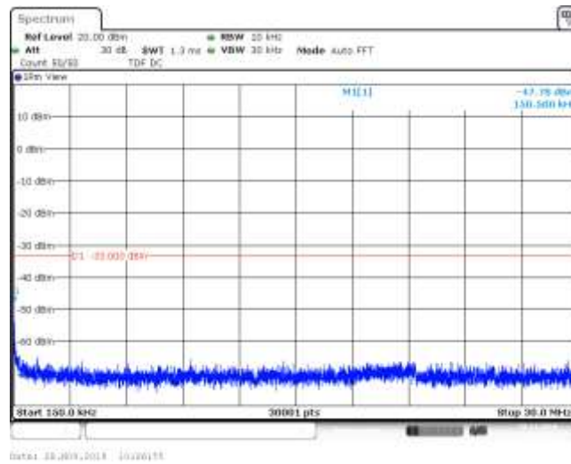
Band17_5MHz_16QAM_23790_1RB#0
