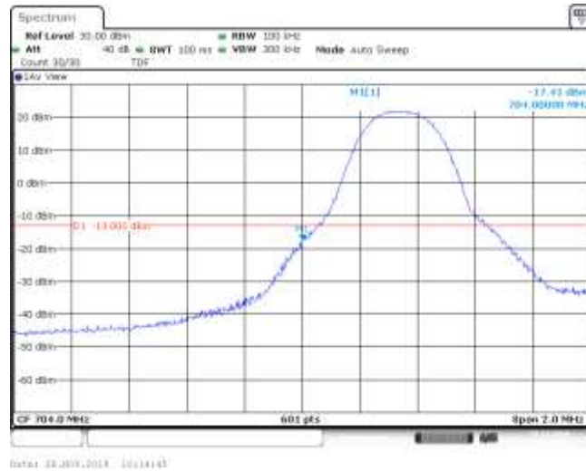
Band17_5MHz_QPSK_23755_1RB#12
