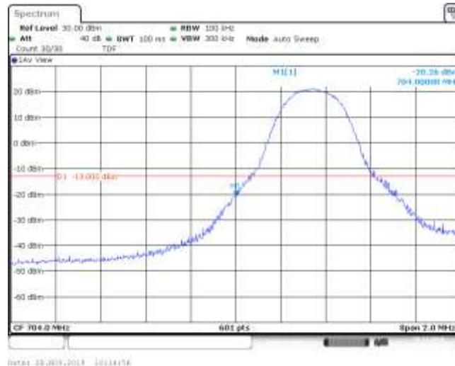
Band17_5MHz_16QAM_23755_1RB#12
