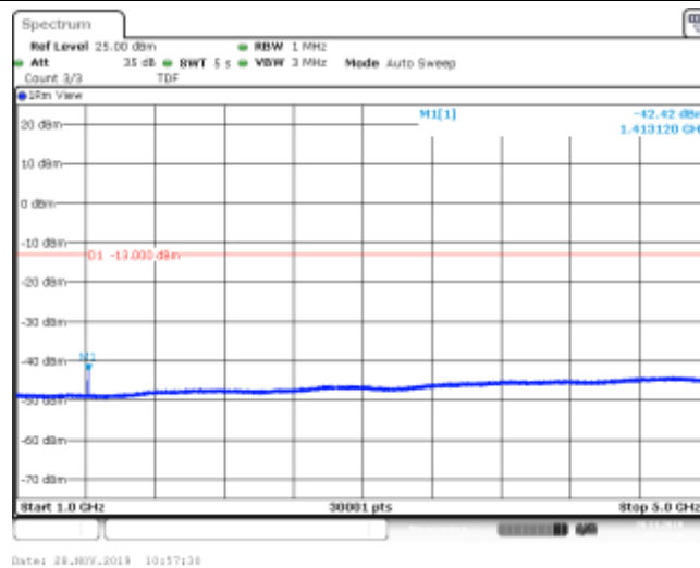
Band17_10MHz_QPSK_23800_1RB#0
