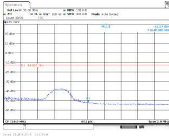
Band17_5MHz_16QAM_23825_1RB#12
