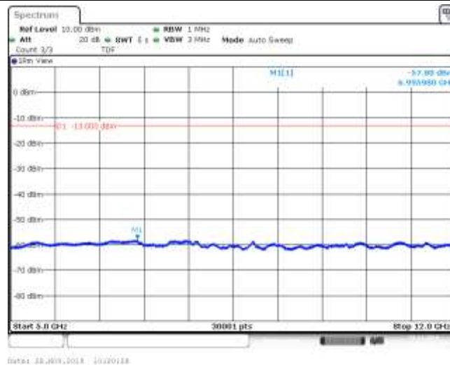
Band17_5MHz_QPSK_23755_1RB#0
