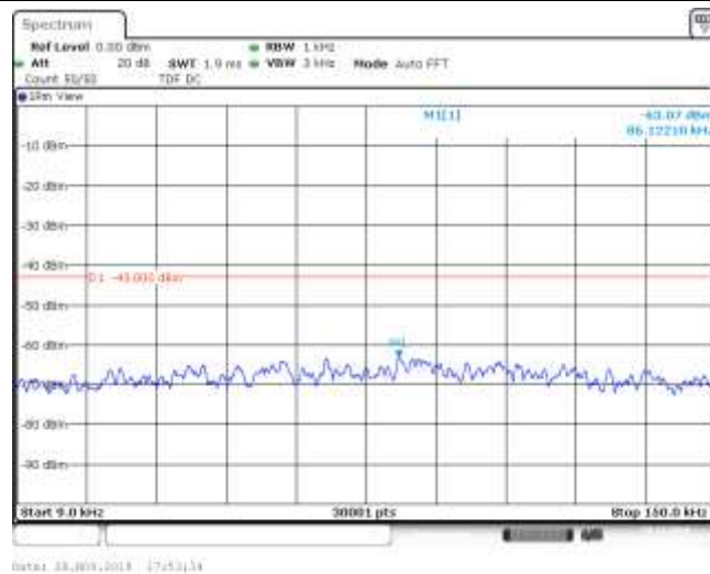
Band17_10MHz_QPSK_23780_1RB#0
