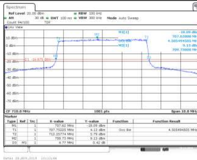
Band17_5MHz_16QAM_23790_25RB#0
