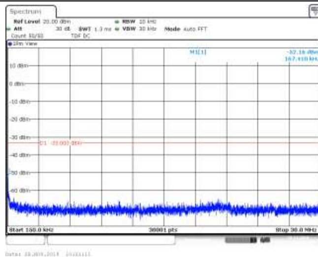
Band17_5MHz_16QAM_23755_1RB#0
