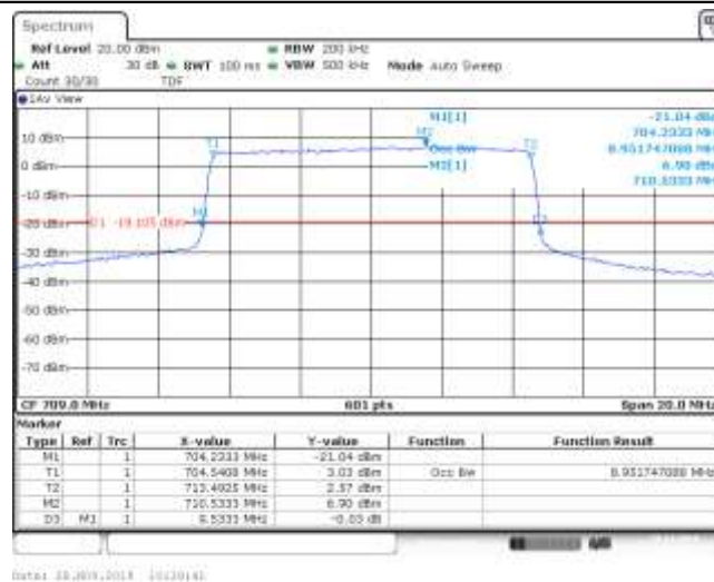
Band17_10MHz_16QAM_23780_50RB#0
