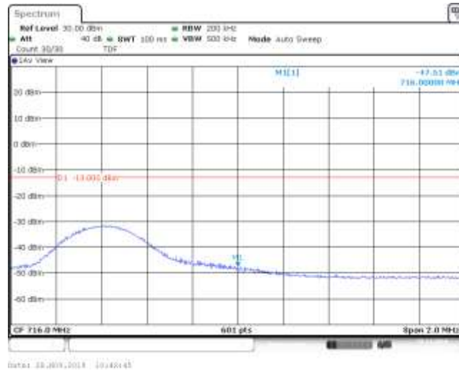
Band17_10MHz_16QAM_23800_1RB#24
