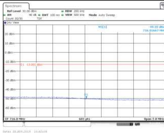
Band17_10MHz_16QAM_23800_1RB#24
