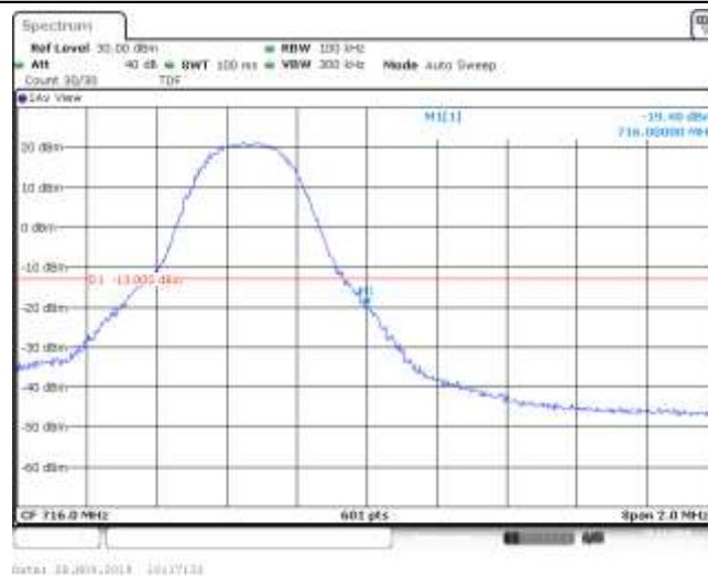
Band17_5MHz_16QAM_23825_1RB#24
