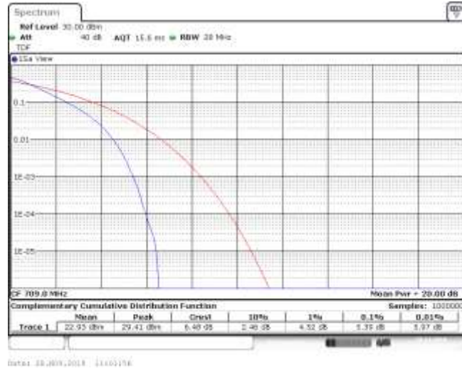
Band17_10MHz_QPSK_23790_1RB#0
