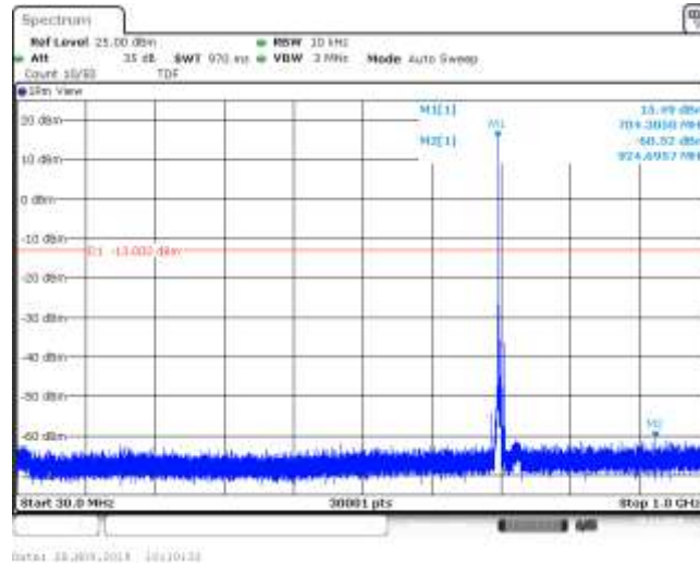
Band17_5MHz_QPSK_23755_1RB#0
