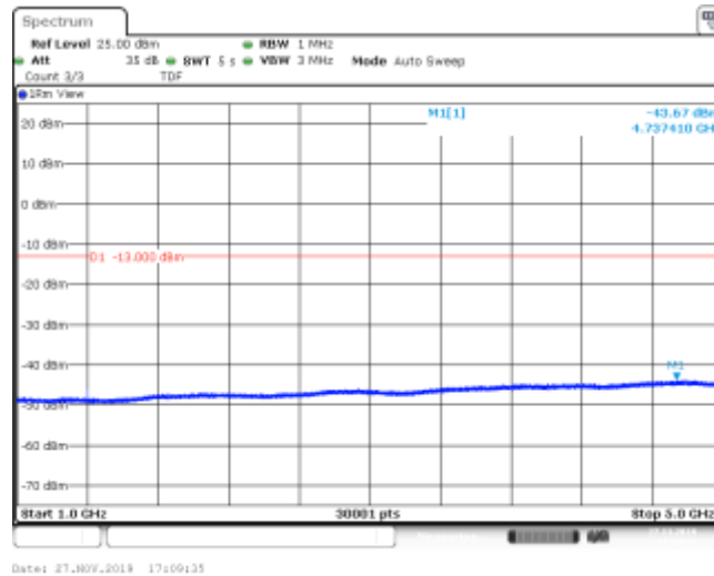
Band12_1.4MHz_QPSK_23017_1RB#0
