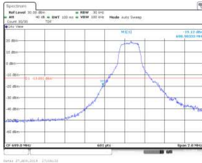
Band12_1.4MHz_16QAM_23017_1RB#2
