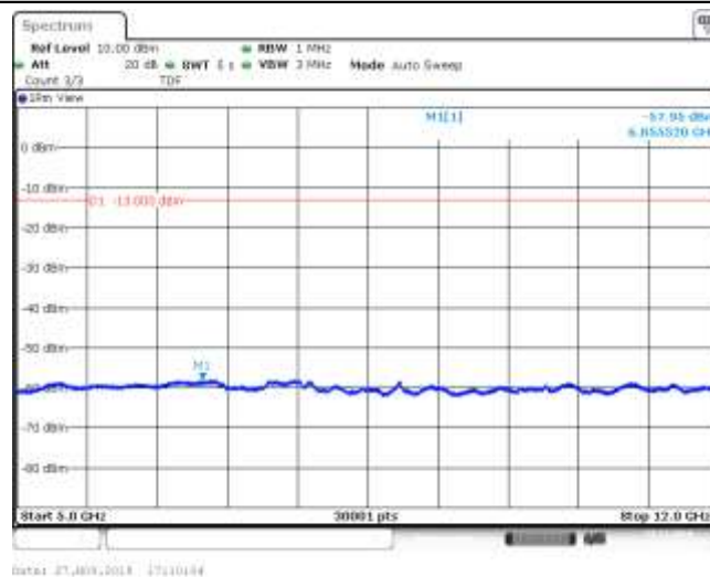
Band12_1.4MHz_QPSK_23017_1RB#0
