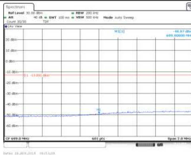
Band12_10MHz_QPSK_23060_1RB#24
