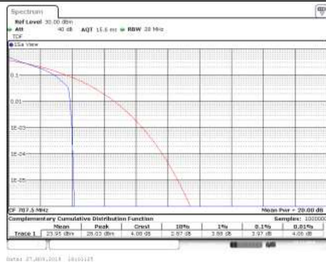
Band12_3MHz_QPSK_23095_1RB#0
