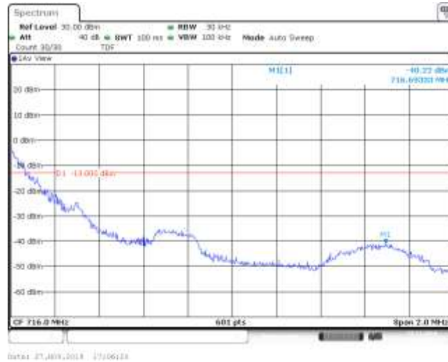
Band12_1.4MHz_16QAM_23173_1RB#2
