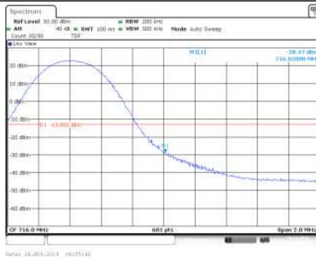
Band12_10MHz_QPSK_23130_1RB#49
