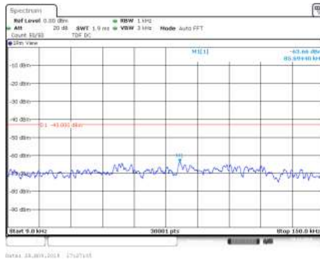
Band12_10MHz_QPSK_23130_1RB#0
