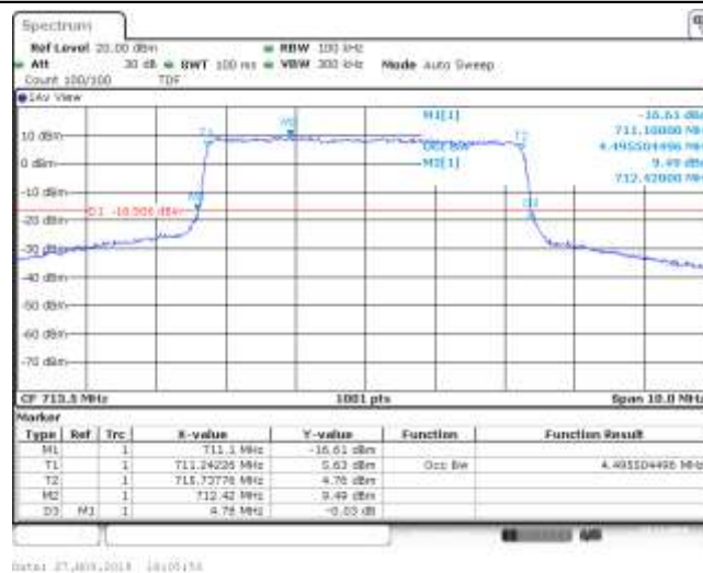
Band12_5MHz_QPSK_23155_25RB#0
