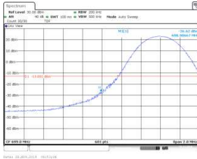
Band12_10MHz_QPSK_23060_1RB#24
