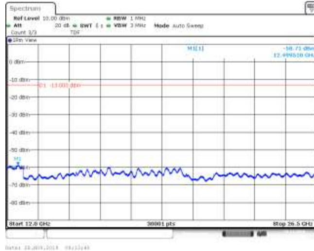
Band12_10MHz_16QAM_23130_1RB#0
