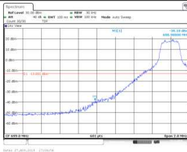
Band12_1.4MHz_16QAM_23017_1RB#2
