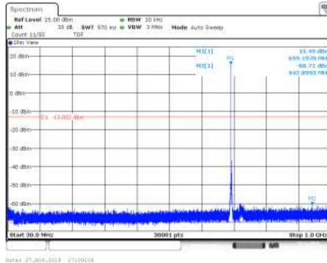
Band12_1.4MHz_QPSK_23017_1RB#0
