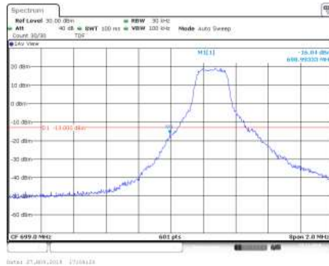
Band12_1.4MHz_QPSK_23017_1RB#2
