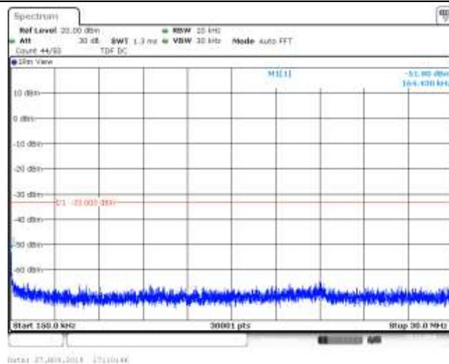
Band12_1.4MHz_16QAM_23017_1RB#0
