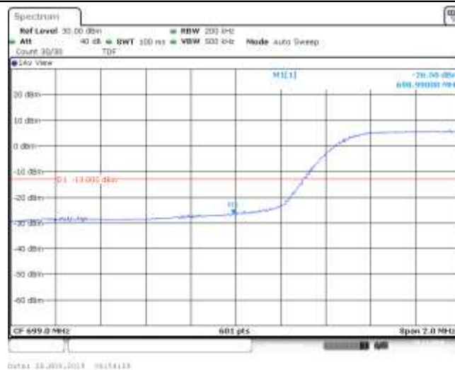
Band12_10MHz_16QAM_23060_50RB#0
