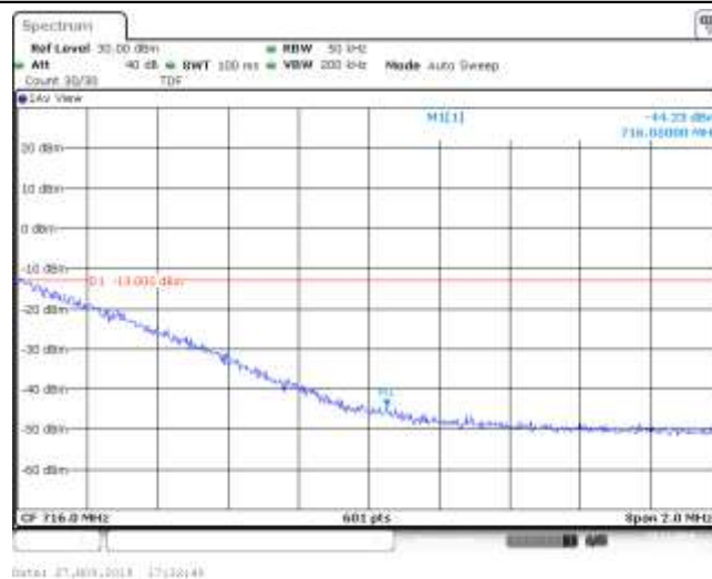
Band12_3MHz_16QAM_23165_1RB#8
