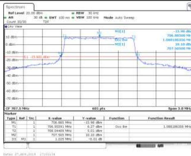
Band12_1.4MHz_16QAM_23095_6RB#0
