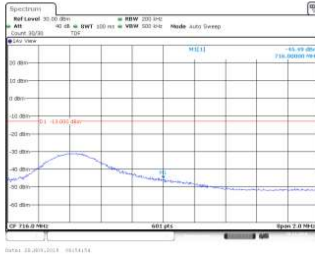
Band12_10MHz_QPSK_23130_1RB#24
