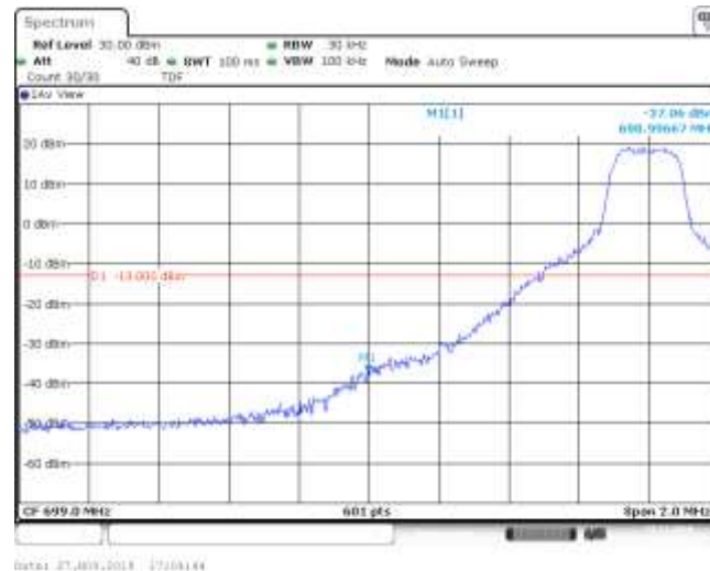
Band12_1.4MHz_QPSK_23017_1RB#5
