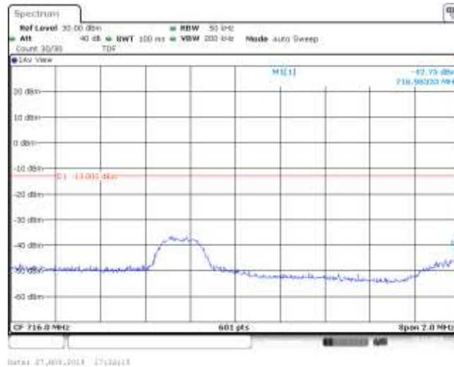
Band12_3MHz_16QAM_23165_1RB#8
