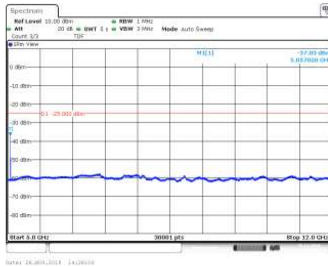
Band7_15MHz_16QAM_21100_1RB#0
