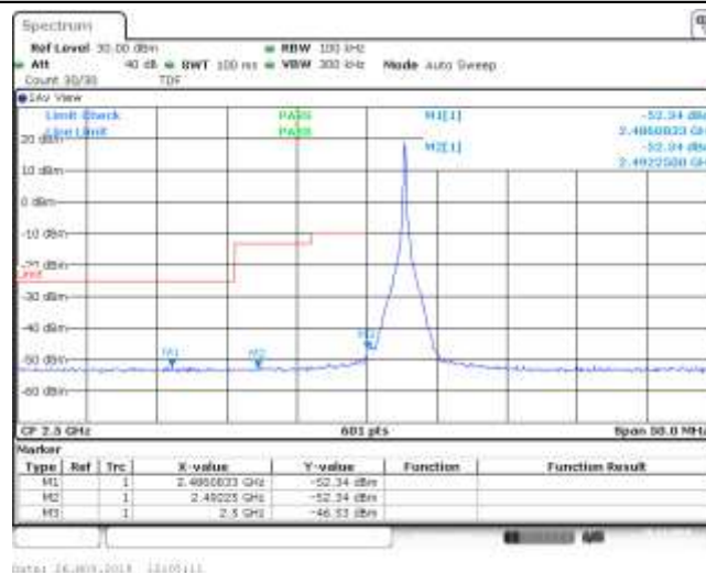
Band7_5MHz_16QAM_20775_1RB#12
