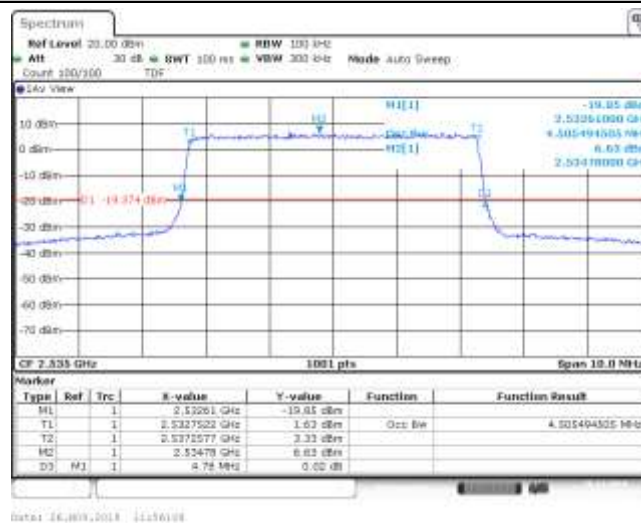
Band7_5MHz_16QAM_21100_25RB#0
