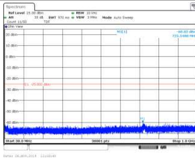
Band7_5MHz_16QAM_21100_1RB#0
