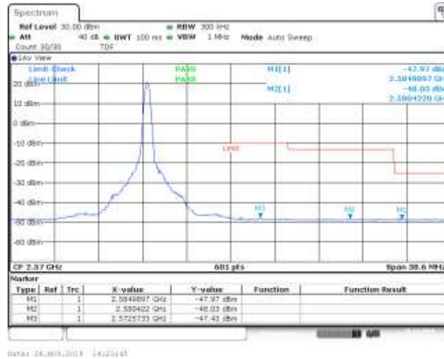
Band7_15MHz_QPSK_21375_1RB#74
