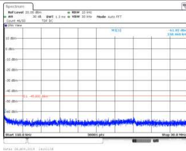
Band7_10MHz_16QAM_21100_1RB#0
