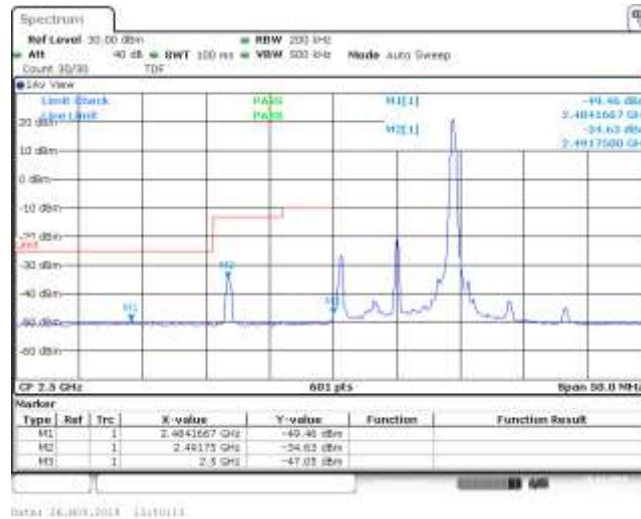
Band7_10MHz_QPSK_20800_50RB#0
