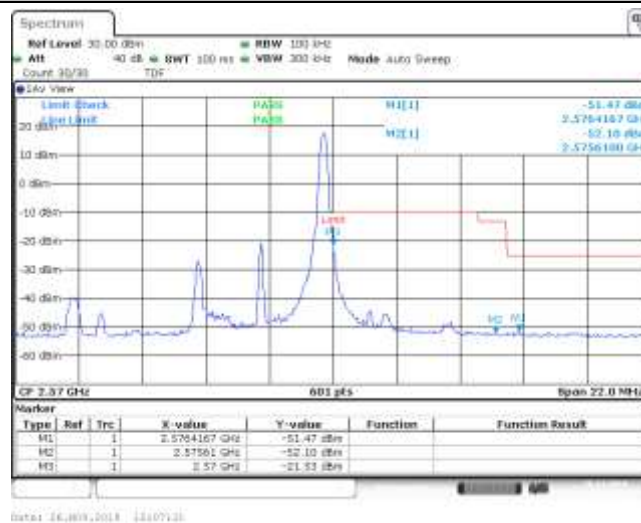
Band7_5MHz_16QAM_21425_1RB#24
