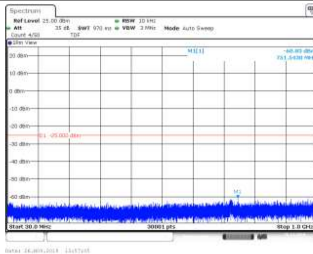
Band7_10MHz_16QAM_20800_1RB#0
