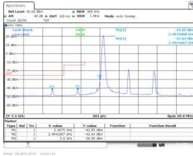
Band7_15MHz_QPSK_20825_1RB#38
