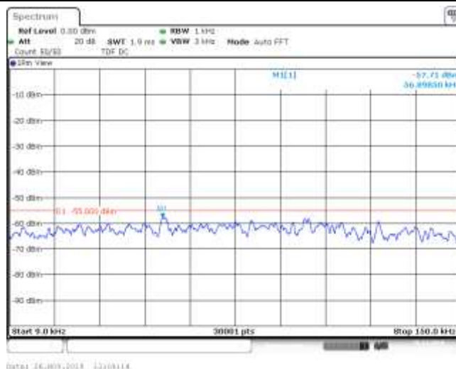
Band7_5MHz_QPSK_21425_1RB#0
