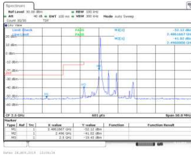
Band7_5MHz_QPSK_20775_1RB#12
