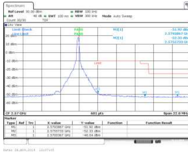
Band7_5MHz_16QAM_21425_1RB#24
