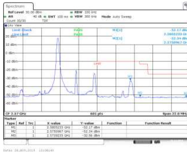
Band7_5MHz_16QAM_21425_1RB#12
