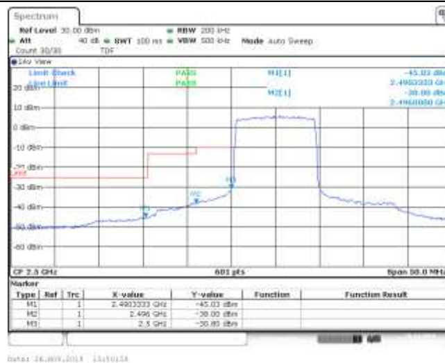
Band7_10MHz_QPSK_20800_50RB#0
