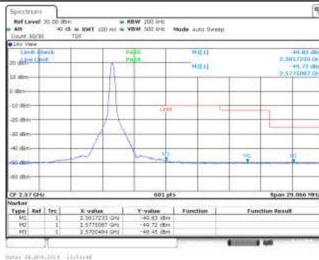
Band7_10MHz_16QAM_21400_1RB#24
