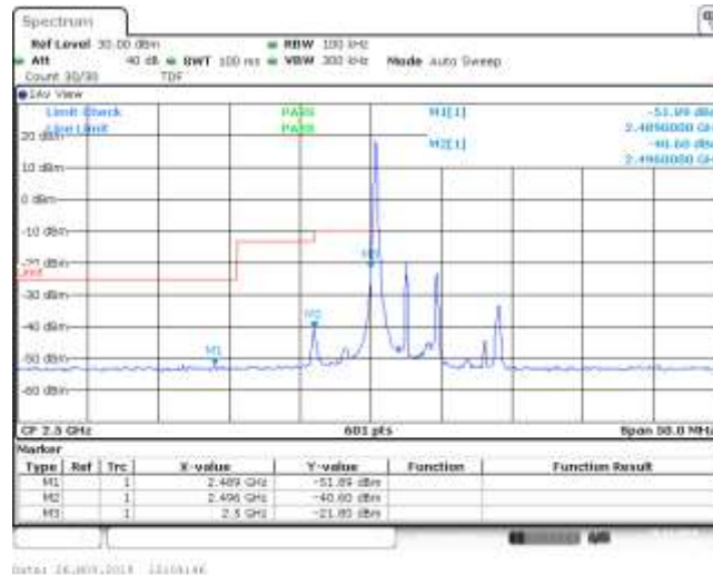
Band7_5MHz_16QAM_20775_1RB#12
