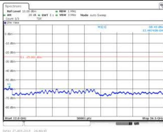
Band7_20MHz_16QAM_21100_1RB#0
