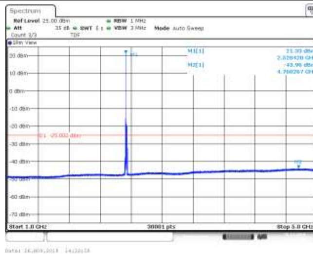
Band7_15MHz_QPSK_21100_1RB#0
