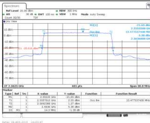
Band7_15MHz_QPSK_21375_75RB#0
