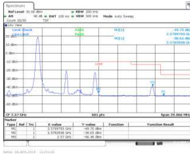
Band7_10MHz_16QAM_21400_1RB#24
