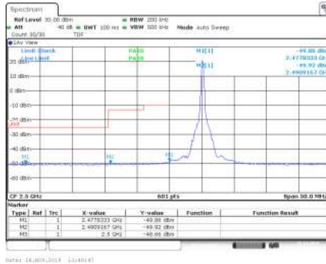
Band7_10MHz_QPSK_20800_1RB#49
