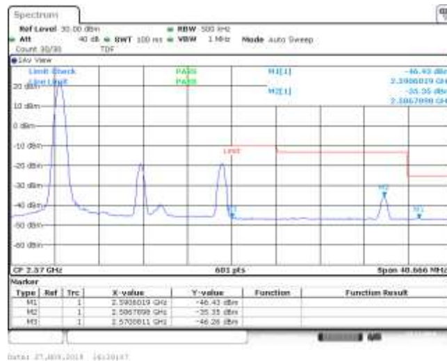
Band7_20MHz_QPSK_21350_1RB#49
