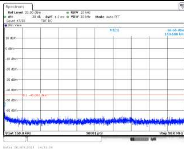
Band7_15MHz_QPSK_21100_1RB#0
