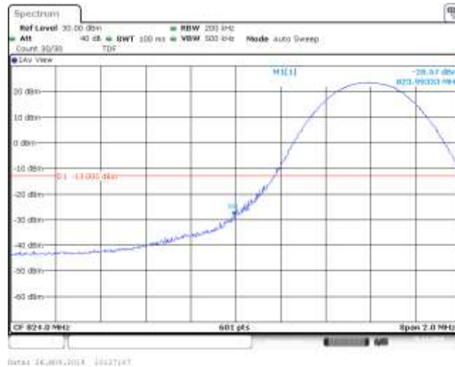
Band5_10MHz_QPSK_20450_1RB#24
