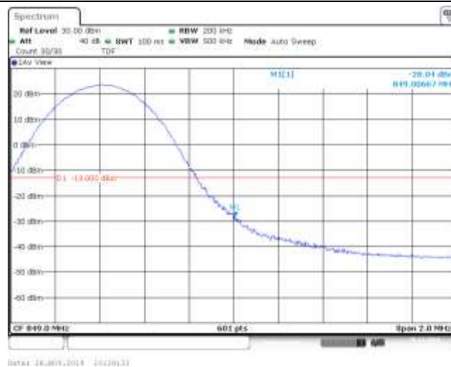
Band5_10MHz_QPSK_20600_1RB#49
