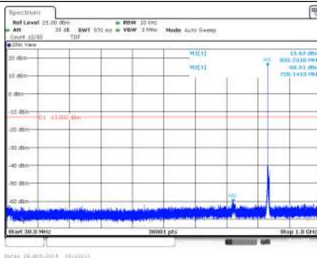
Band5 3MHz 16QAM 20525 1RB#0
