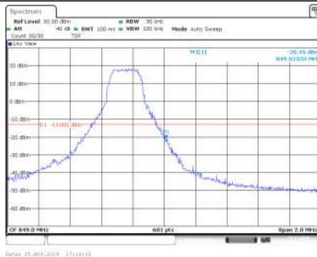
Band5_1.4MHz_16QAM_20643_1RB#5
