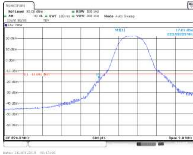
Band5_5MHz_QPSK_20425_1RB#12
