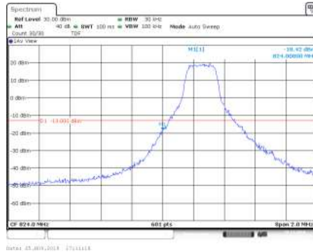
Band5_1.4MHz_QPSK_20407_1RB#2
