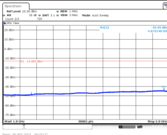
Band5_3MHz_16QAM_20525_1RB#0
