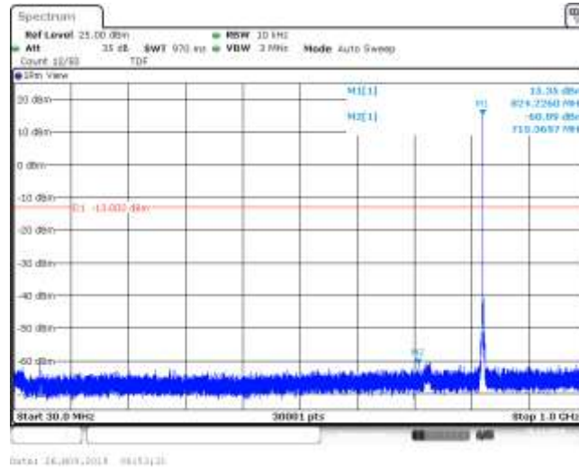
Band5_1.4MHz_QPSK_20407_1RB#0
