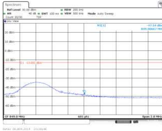
Band5_10MHz_QPSK_20600_1RB#24
