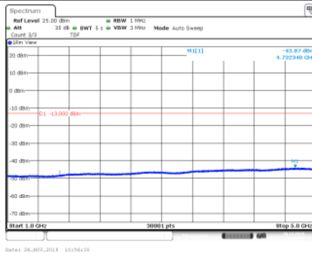
Band5_10MHz_16QAM_20600_1RB#0
