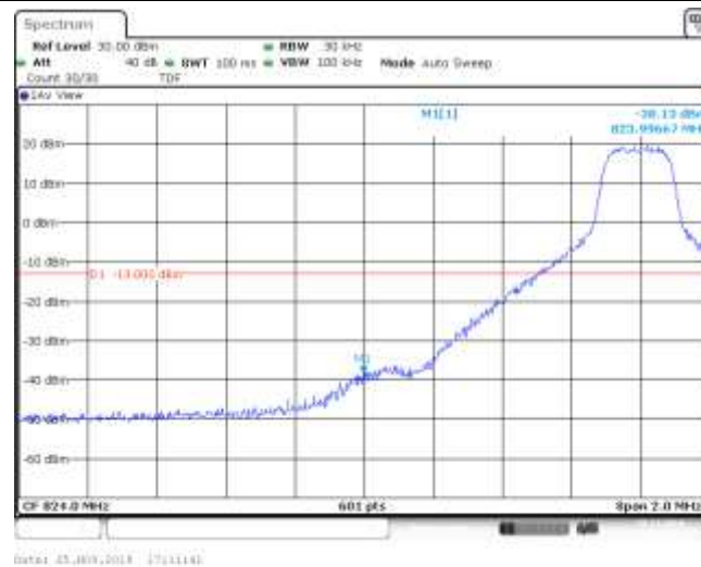
Band5_1.4MHz_QPSK_20407_1RB#5
