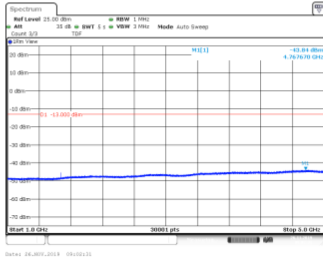
Band5_1.4MHz_16QAM_20525_1RB#0
