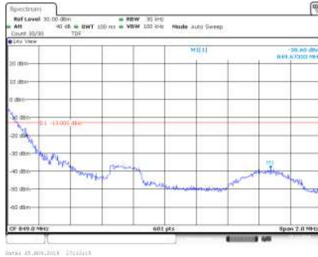
Band5_1.4MHz_16QAM_20643_1RB#2
