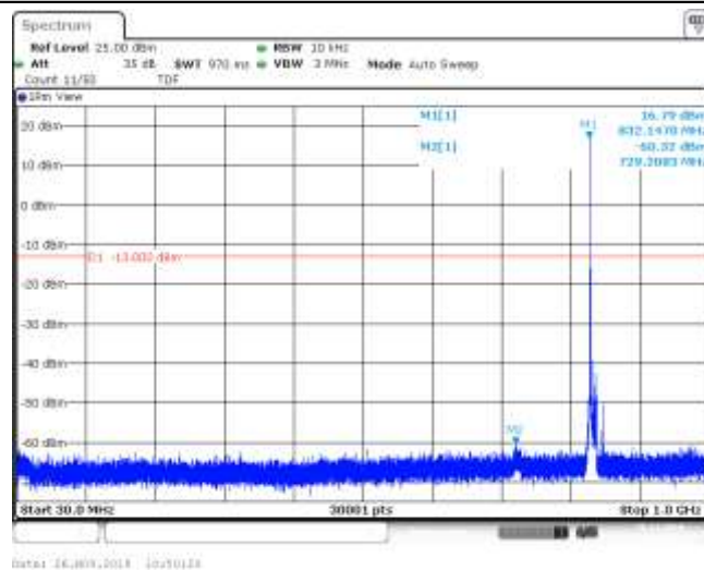
Band5_10MHz_16QAM_20525_1RB#0
