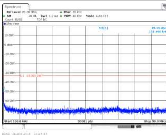
Band5_10MHz_QPSK_20525_1RB#0
