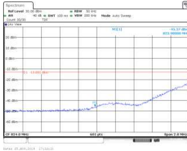
Band5_3MHz_QPSK_20415_1RB#14
