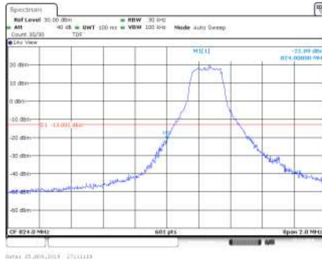
Band5_1.4MHz_16QAM_20407_1RB#2
