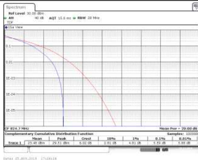
Band5_1.4MHz_QPSK_20525_1RB#0
