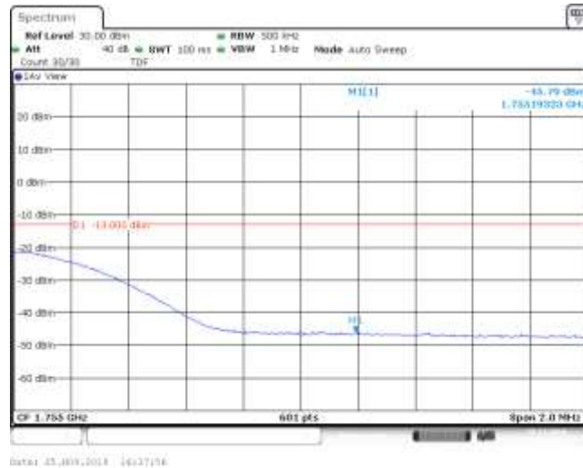
Band4_20MHz_QPSK_20300_1RB#49
