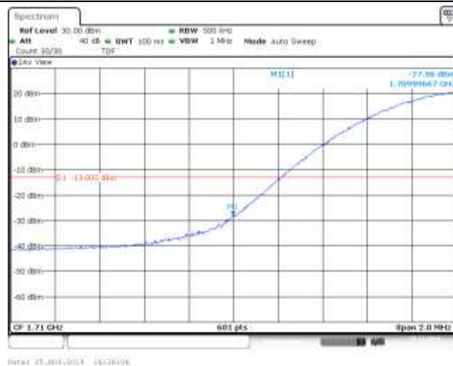
Band4_20MHz_16QAM_20050_1RB#49
