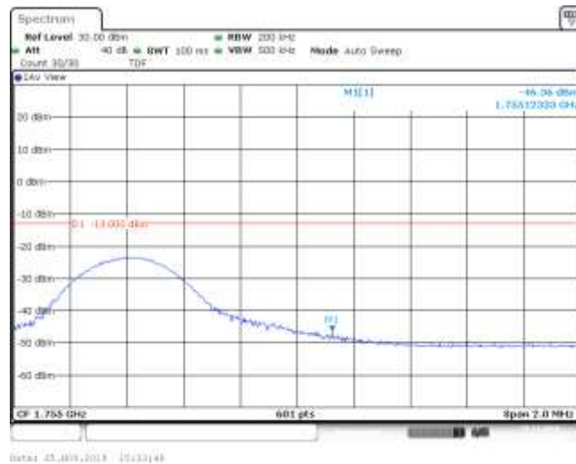
Band4_10MHz_16QAM_20350_1RB#24
