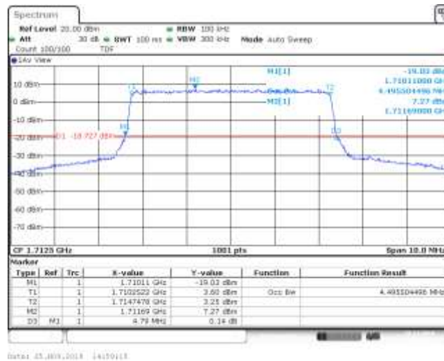
Band4_5MHz_16QAM_20175_25RB#0
