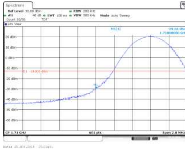
Band4_10MHz_16QAM_20000_1RB#24
