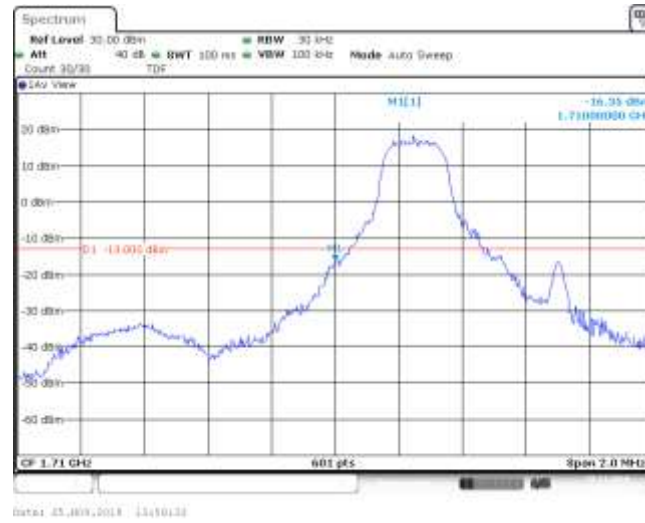
Band4_1.4MHz_QPSK_19957_1RB#2
