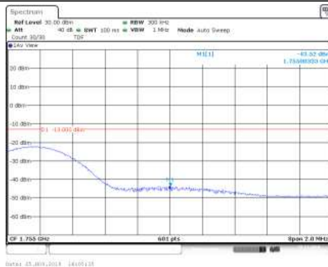
Band4_15MHz_16QAM_20325_1RB#38
