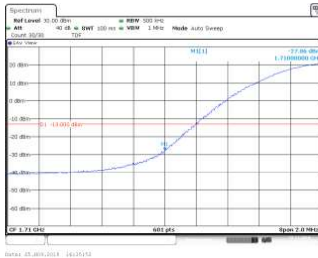
Band4_20MHz_QPSK_20050_1RB#49
