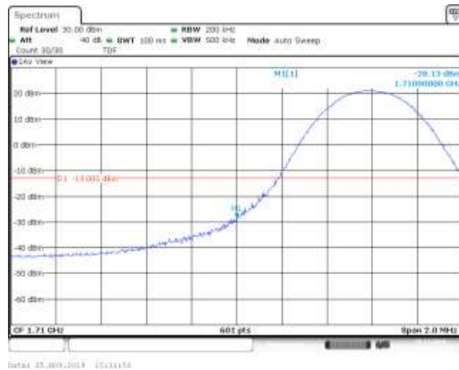
Band4_10MHz_QPSK_20000_1RB#24
