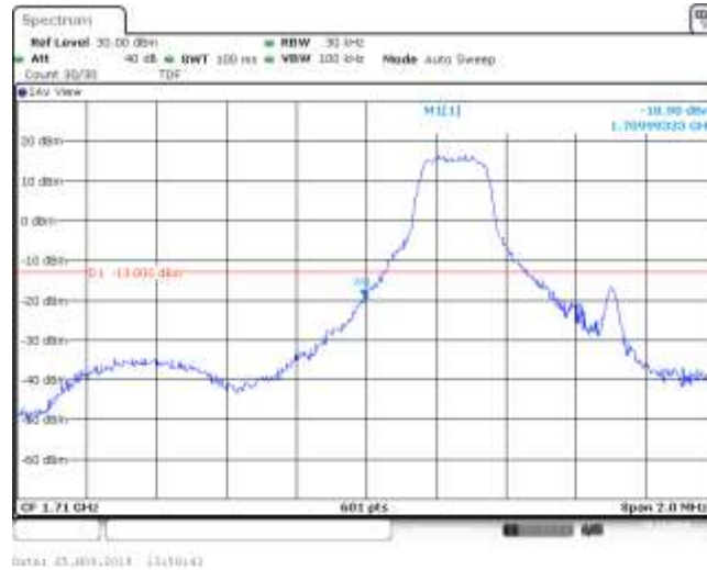
Band4_1.4MHz_16QAM_19957_1RB#2
