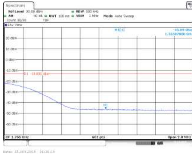
Band4_20MHz_16QAM_20300_1RB#49
