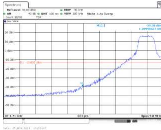
Band4_1.4MHz_16QAM_19957_1RB#5
