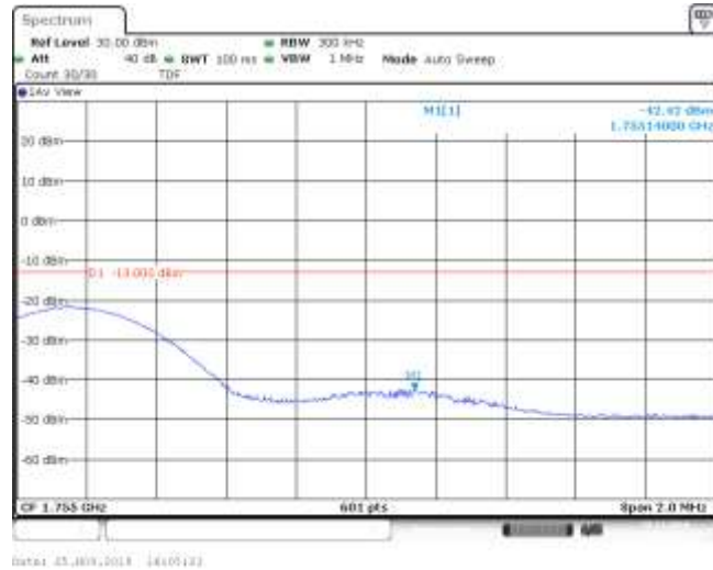
Band4_15MHz_QPSK_20325_1RB#38
