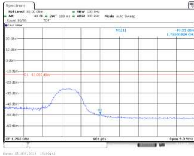
Band4_5MHz_16QAM_20375_1RB#12
