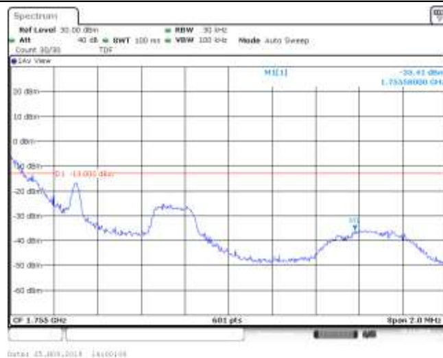
Band4_1.4MHz_QPSK_20393_1RB#2
