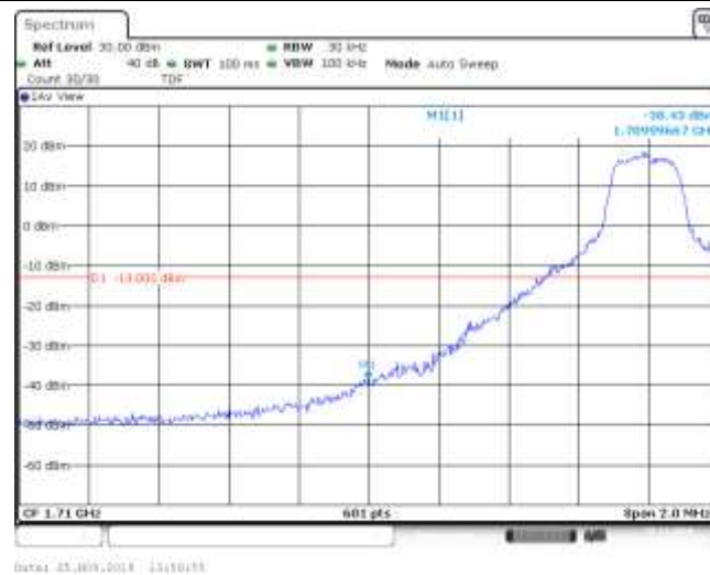
Band4_1.4MHz_QPSK_19957_1RB#5
