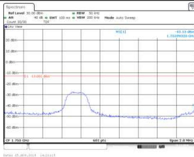
Band4_3MHz_16QAM_20385_1RB#8
