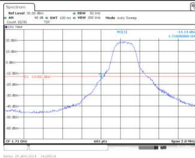
Band4_3MHz_QPSK_19965_1RB#8
