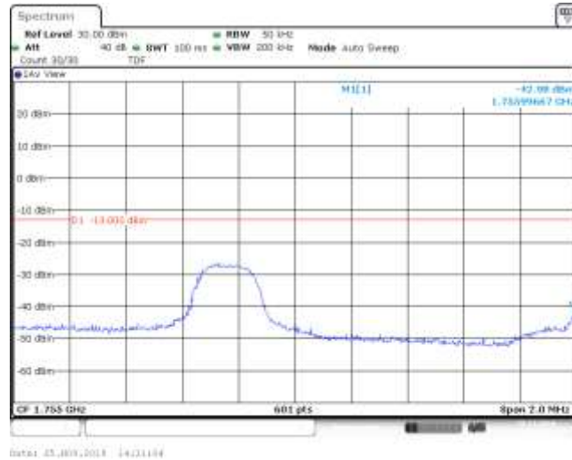
Band4_3MHz_QPSK_20385_1RB#8
