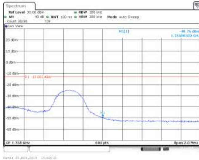
Band4_5MHz_QPSK_20375_1RB#12
