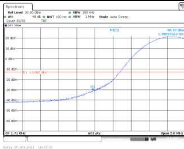
Band4_15MHz_QPSK_20025_1RB#38
