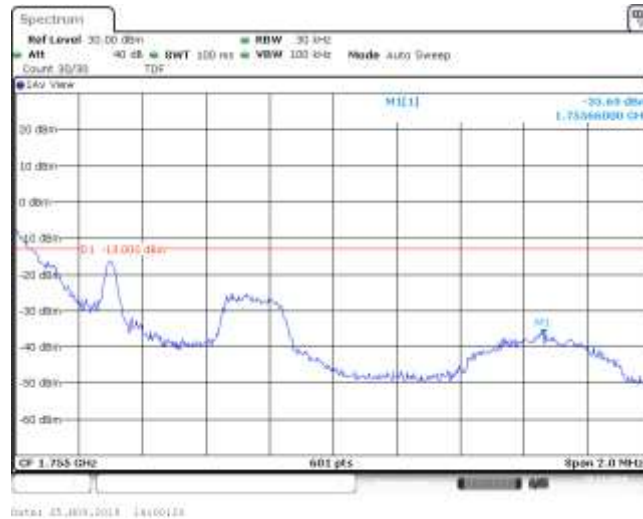
Band4_1.4MHz_16QAM_20393_1RB#2
