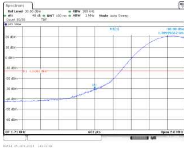
Band4_15MHz_16QAM_20025_1RB#38
