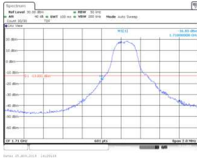
Band4_3MHz_16QAM_19965_1RB#8
