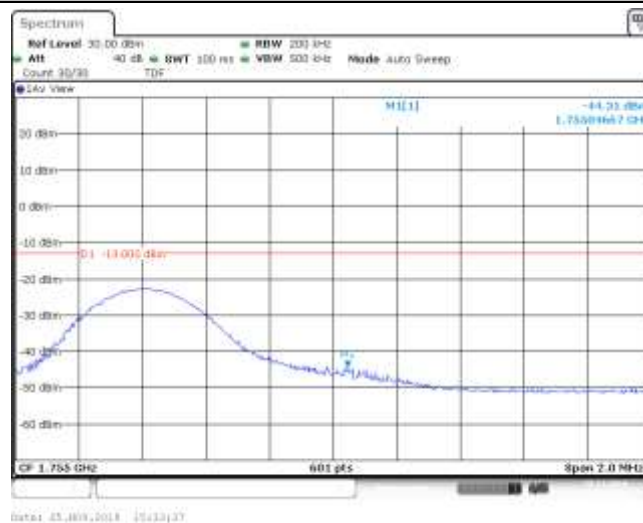
Band4_10MHz_QPSK_20350_1RB#24
