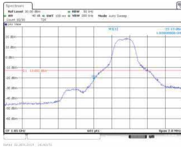
Band2_5MHz_16QAM_18625_1RB#24
