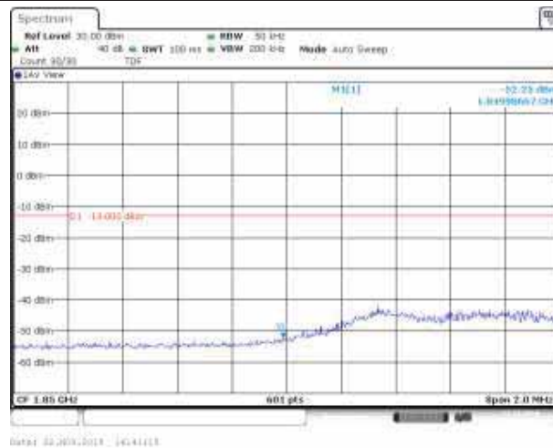
Band2_5MHz_16QAM_18625_25RB#0
