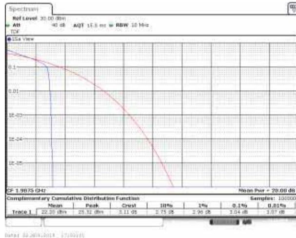
Band2_5MHz_QPSK_19175_25RB#0
