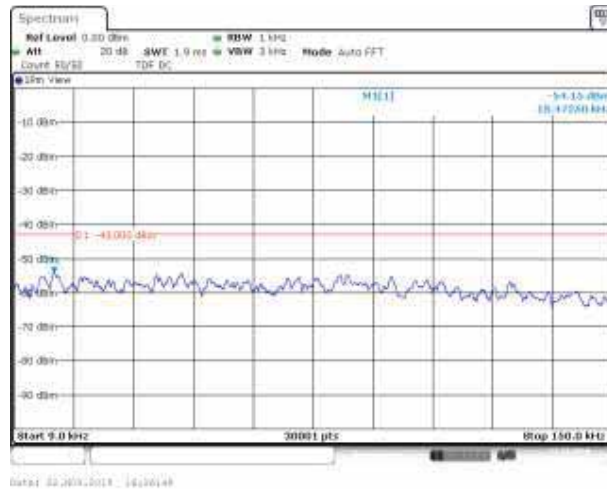
Band2_3MHz_16QAM_19185_1RB#0
