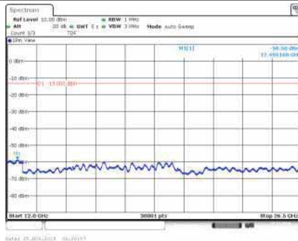
Band2_20MHz_QPSK_19100_1RB#0
