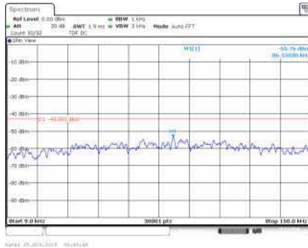
Band2_15MHz_QPSK_19125_1RB#0
