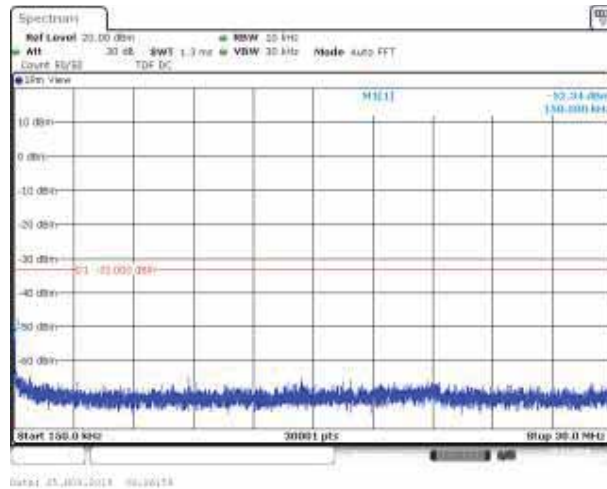
Band2_20MHz_16QAM_19100_1RB#0
