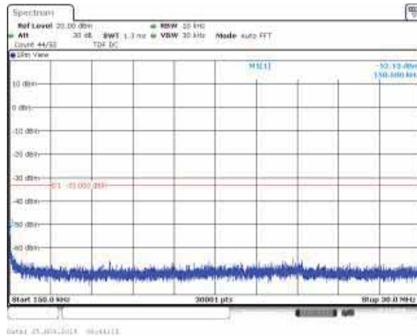
Band2_15MHz_QPSK_18900_1RB#0
