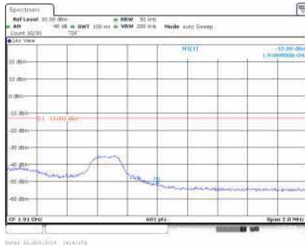
Band2_5MHz_QPSK_19175_1RB#24
