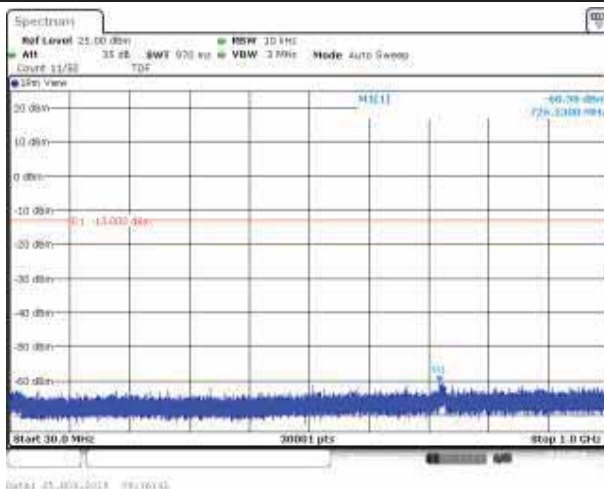
Band2_20MHz_16QAM_18700_1RB#0
