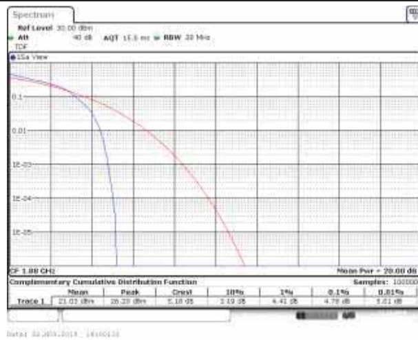
Band2_1.4MHz_16QAM_18900_6RB#0
