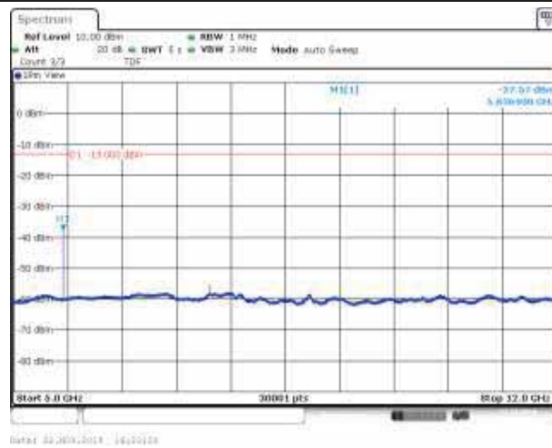
Band2_3MHz_16QAM_18900_1RB#0
