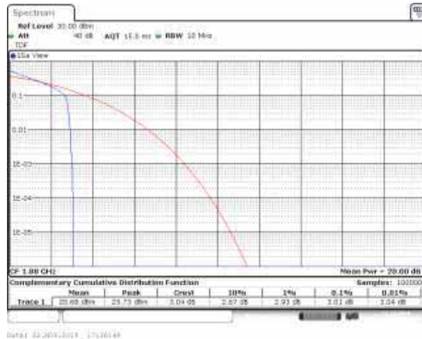
Band2_10MHz_QPSK_18900_50RB#0
