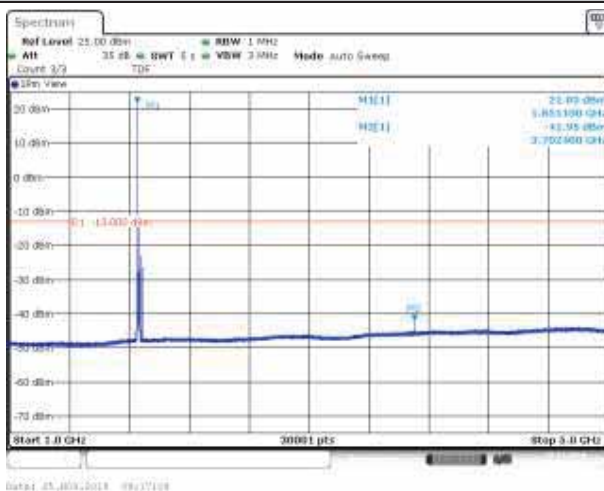
Band2_20MHz_16QAM_18700_1RB#0
