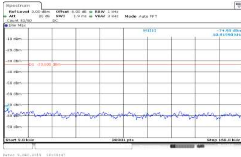
Band V-4233-HSUPA_Sub3-0.009~0.15
