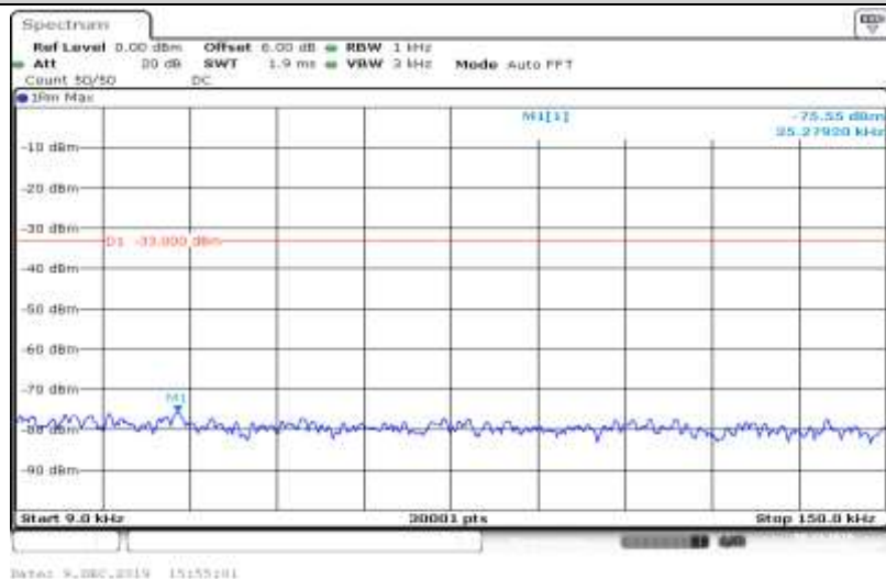
Band V-4182-HSUPA_Sub5-0.009~0.15
