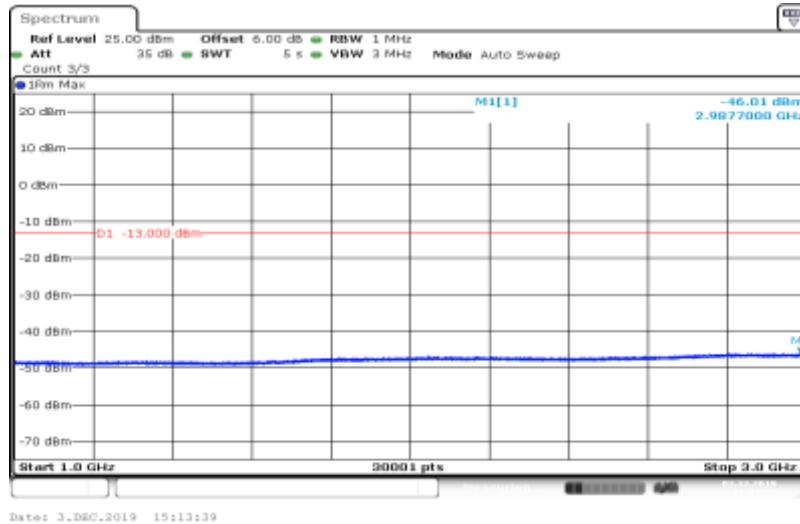
Band V-4132-HSDPA_Sub2-1000~3000
