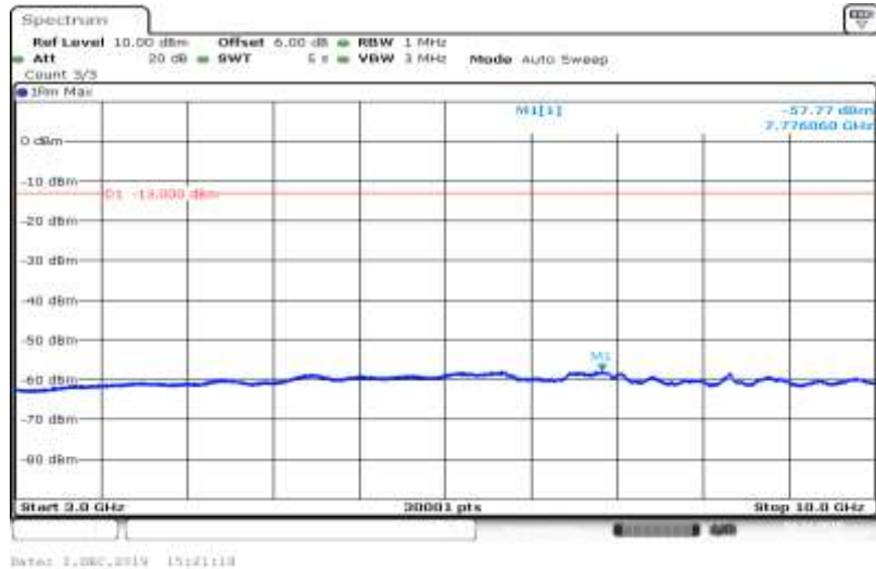
Band V-4132-HSDPA_Sub4-3000~10000
