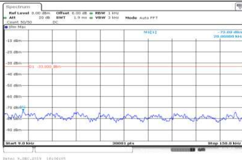
Band V-4182-HSUPA_Sub2-0.009~0.15
