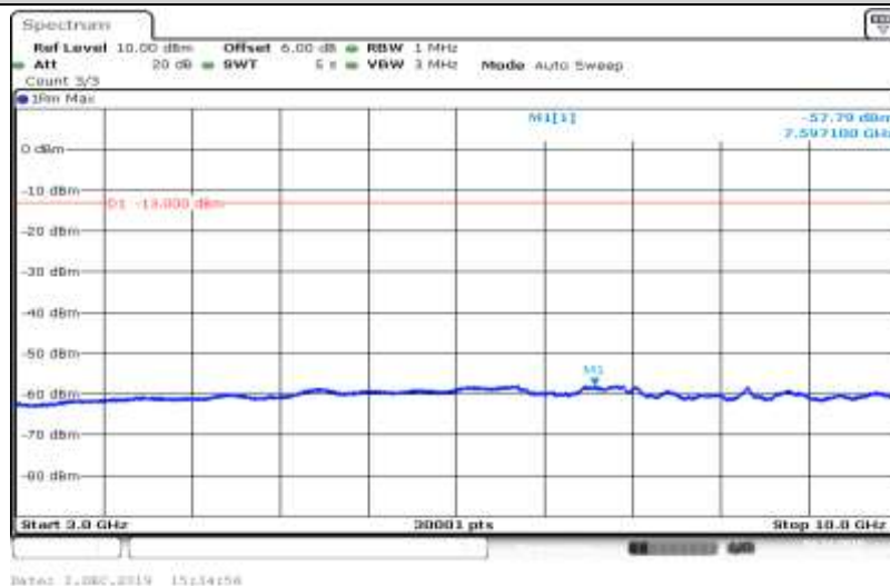
Band V-4182-HSDPA_Sub2-3000~10000
