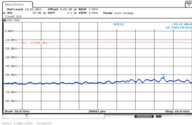
Band V-4233-HSDPA_Sub2-10000~18000
