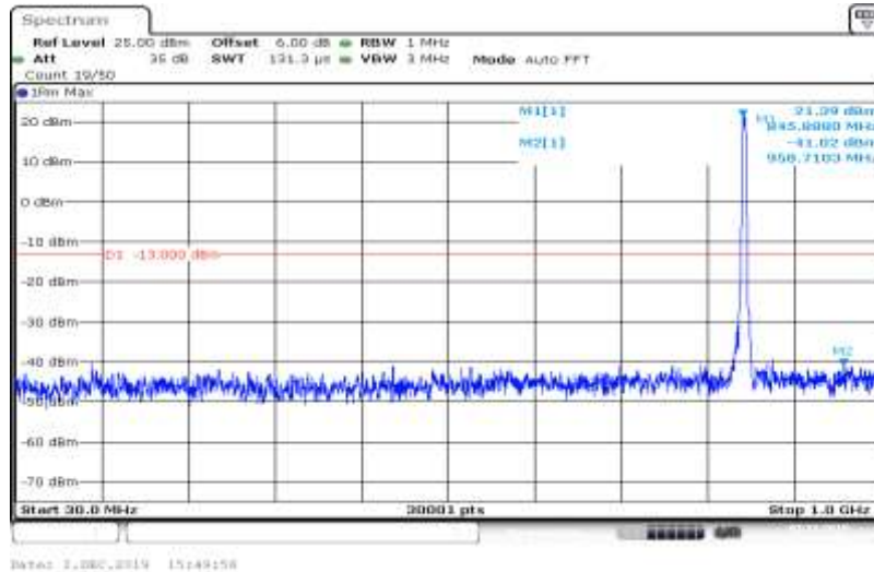
Band V-4233-HSDPA_Sub2-30~1000
