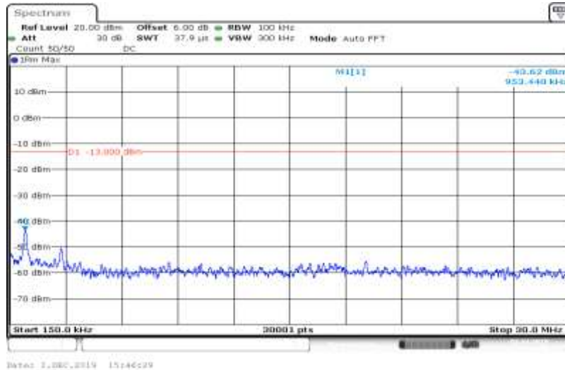
Band V-4233-HSDPA_Sub4-0.15~30
