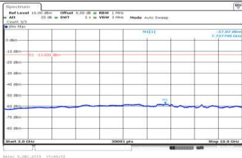
Band V-4132-HSUPA_Sub3-3000~10000
