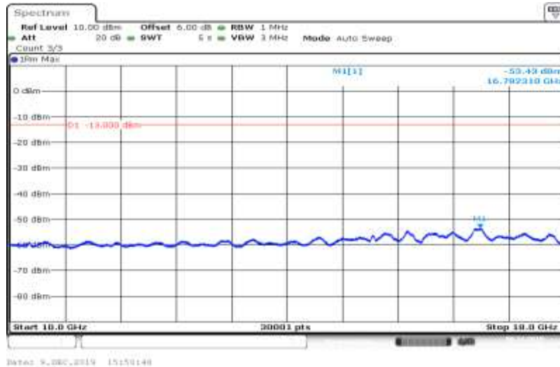
Band V-4132-HSUPA_Sub2-10000~18000
