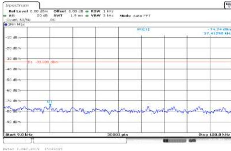
Band V-4182-HSDPA_Sub4-0.009~0.15
