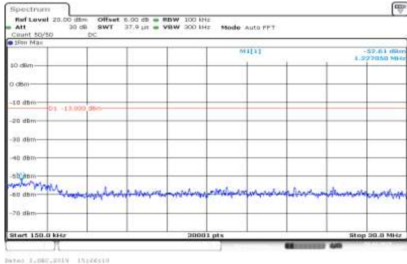
Band V-4182-HSDPA_Sub3-0.15~30
