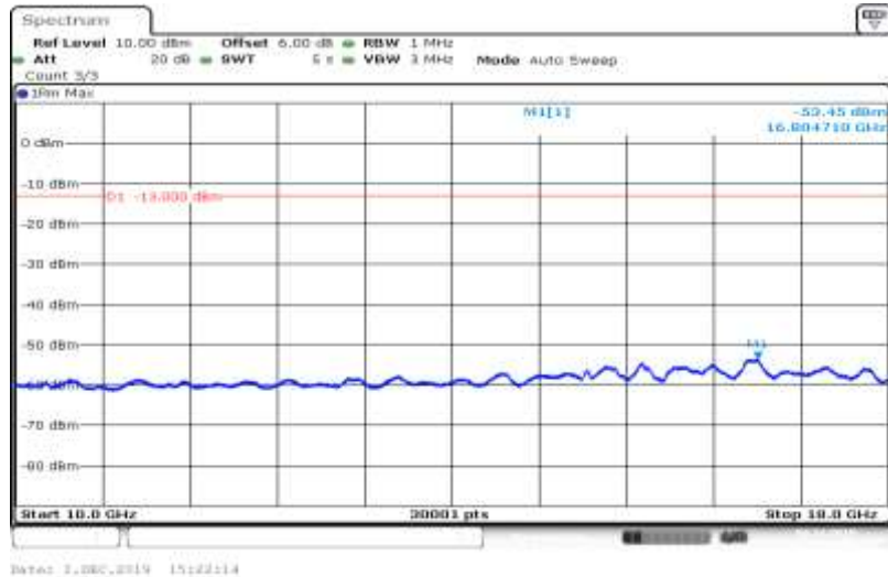
Band V-4132-HSDPA_Sub3-10000~18000
