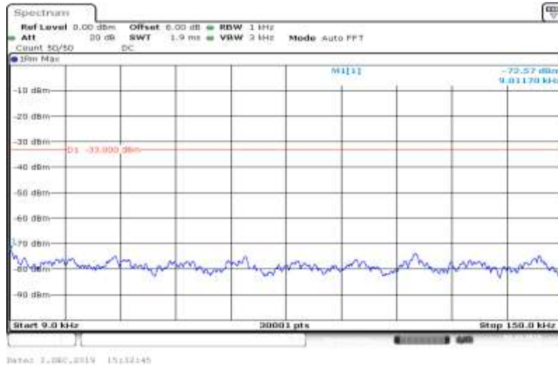
Band V-4182-HSDPA_Sub2-0.009~0.15
