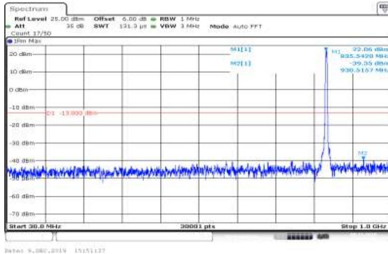
Band V-4182-HSUPA_Sub2-30~1000
