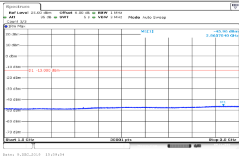
Band V-4182-HSUPA_Sub5-1000~3000
