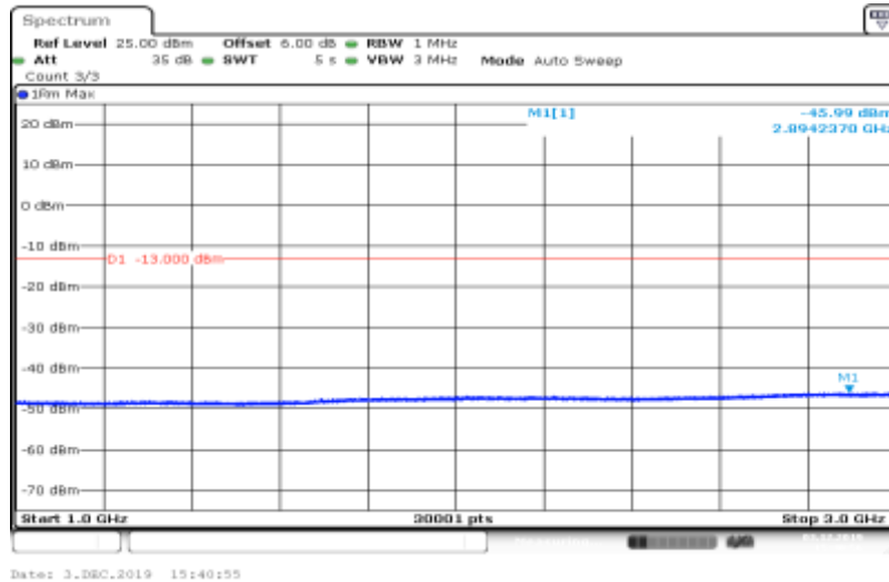
Band V-4233-HSDPA_Sub4-1000~3000
