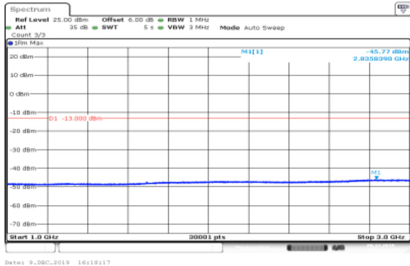
Band V-4233-HSUPA_Sub3-1000~3000
