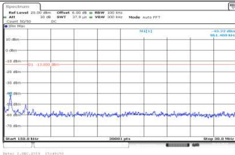
Band V-4233-HSDPA_Sub2-0.15~30
