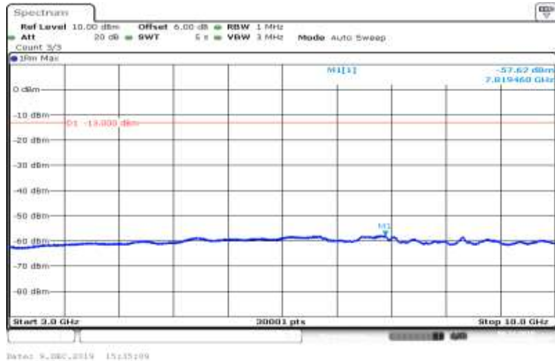
Band V-4132-HSUPA_Sub4-3000~10000
