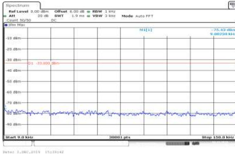
Band V-4233-HSDPA_Sub4-0.009~0.15
