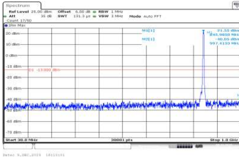
Band V-4233-HSUPA_Sub2-30~1000
