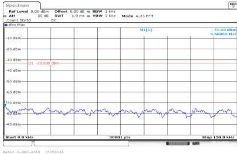
Band V-4182-HSUPA_Sub4-0.009~0.15
