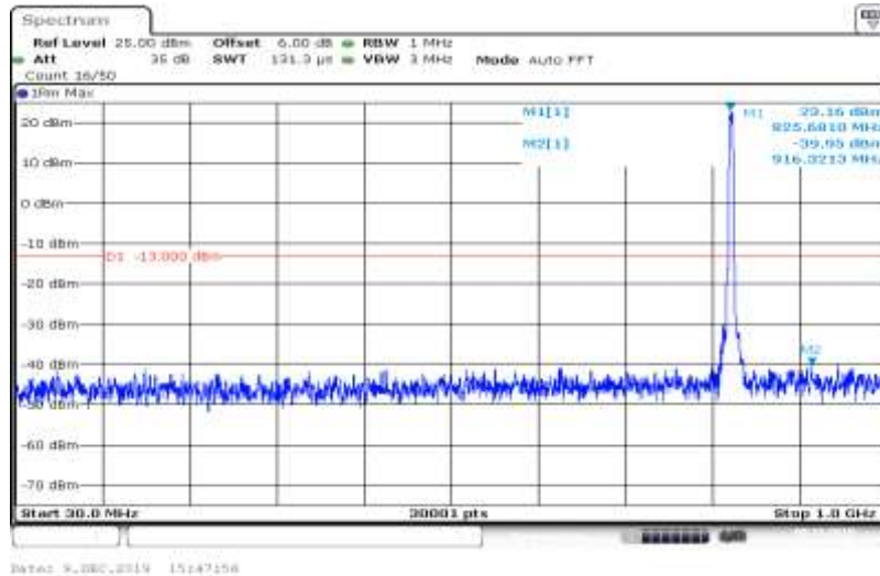
Band V-4132-HSUPA_Sub3-30~1000
