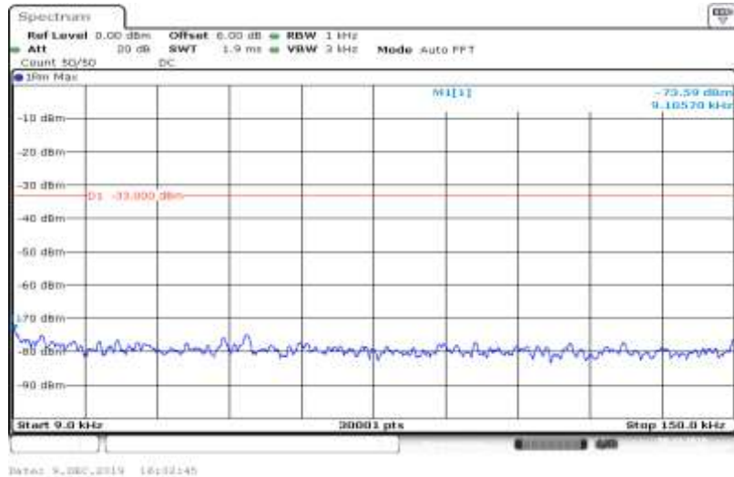
Band V-4182-HSUPA_Sub3-0.009~0.15
