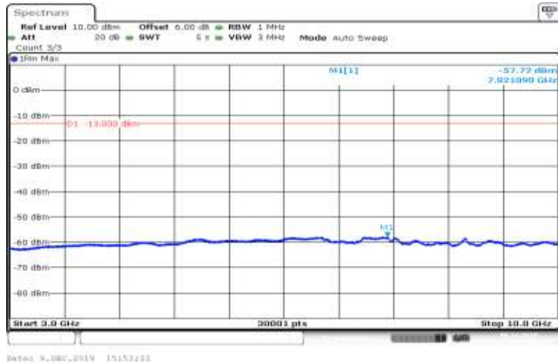
Band V-4182-HSUPA_Sub4-3000~10000
