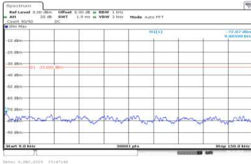
Band V-4132-HSUPA_Sub4-0.009~0.15
