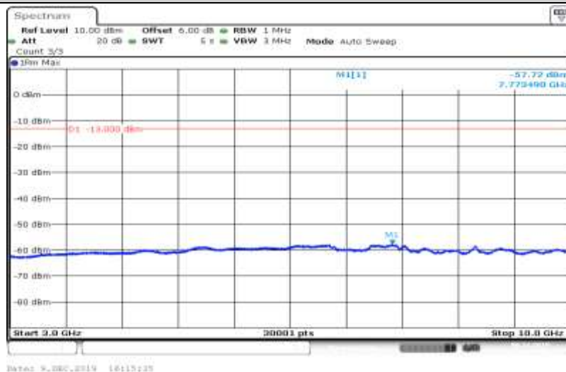
Band V-4233-HSUPA_Sub3-3000~10000
