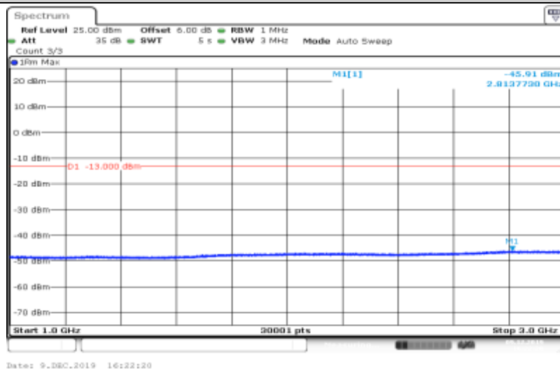
Band V-4233-HSUPA_Sub2-1000~3000
