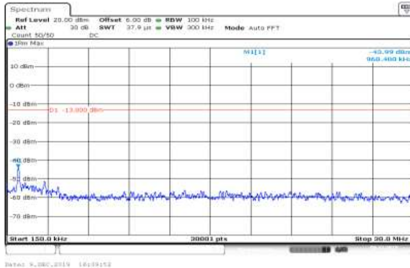
Band V-4233-HSUPA_Sub5-0.15~30
