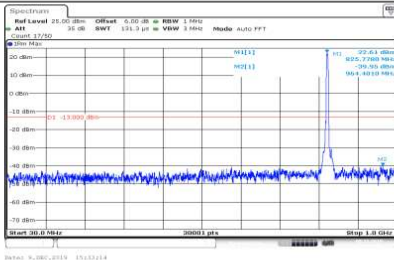
Band V-4132-HSUPA_Sub4-30~1000
