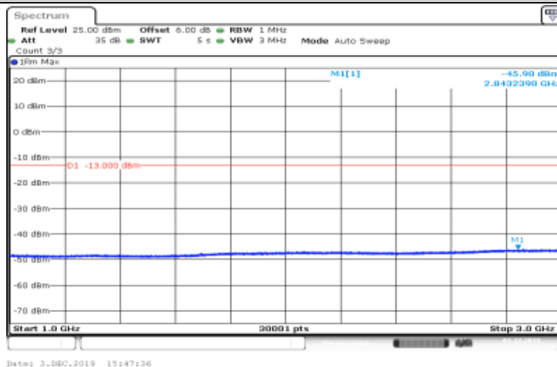
Band V-4233-HSDPA_Sub3-1000~3000
