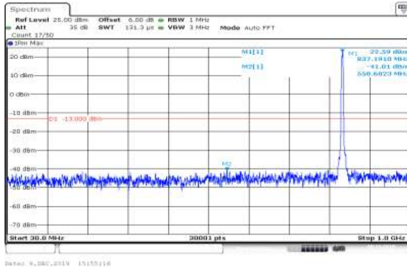
Band V-4182-HSUPA_Sub3-30~1000
