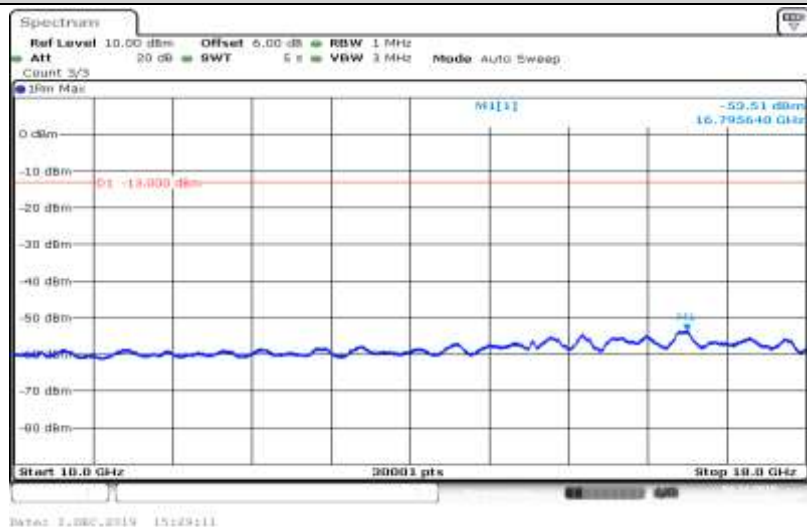
Band V-4182-HSDPA_Sub4-10000~18000
