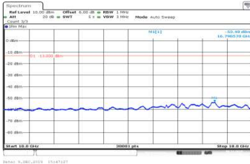
Band V-4132-HSUPA_Sub3-10000~18000
