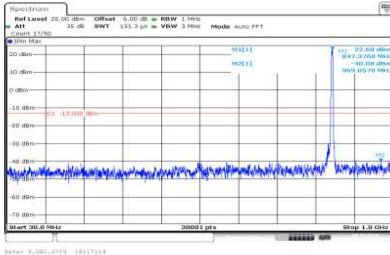
Band V-4233-HSUPA_Sub1-1000~3000
