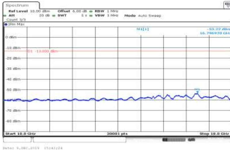
Band V-4132-HSUPA_Sub5-10000~18000
