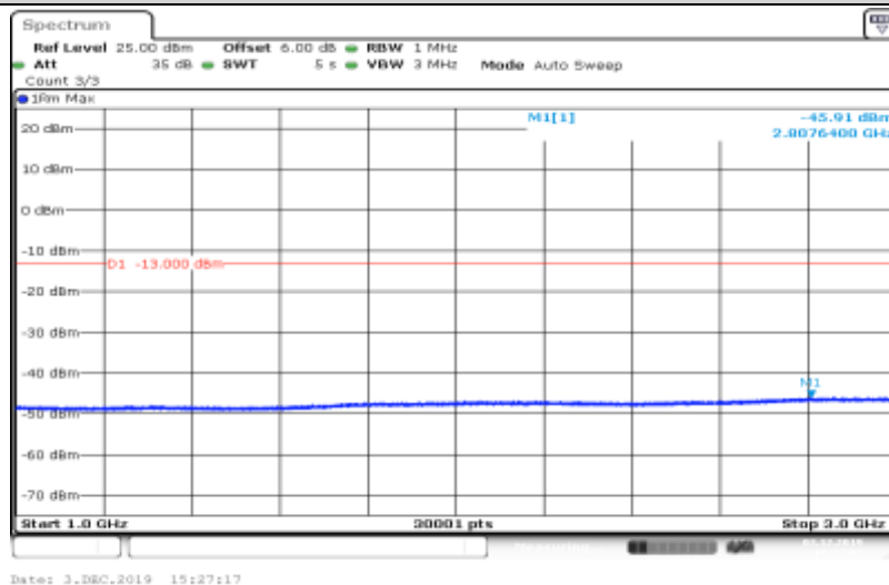
Band V-4182-HSDPA_Sub3-1000~3000
