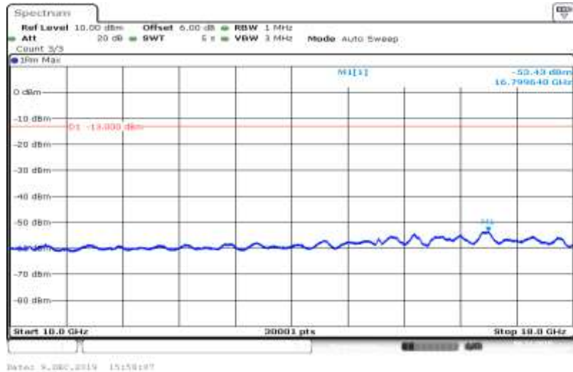
Band V-4182-HSUPA_Sub3-10000~18000
