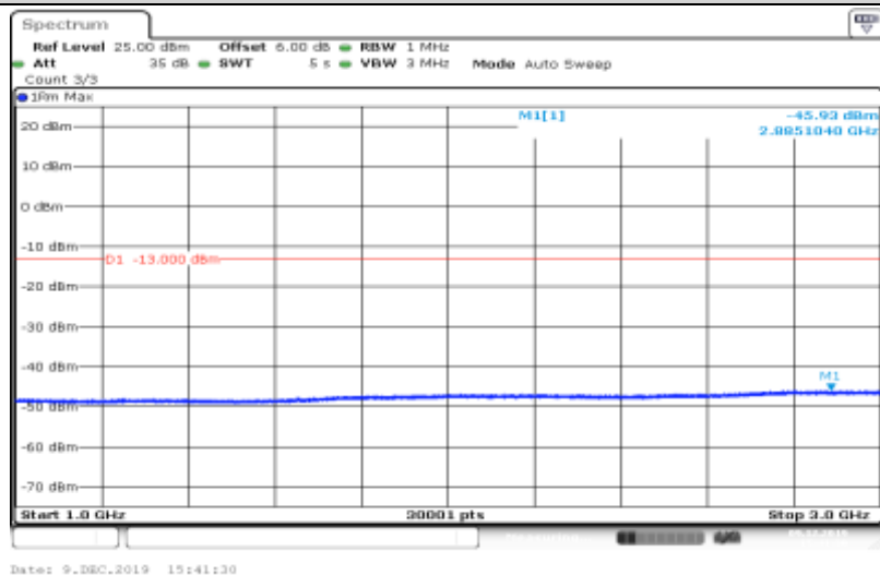
Band V-4132-HSUPA_Sub5-1000~3000
