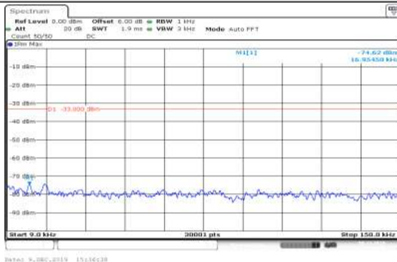
Band V-4132-HSUPA_Sub5-0.009~0.15
