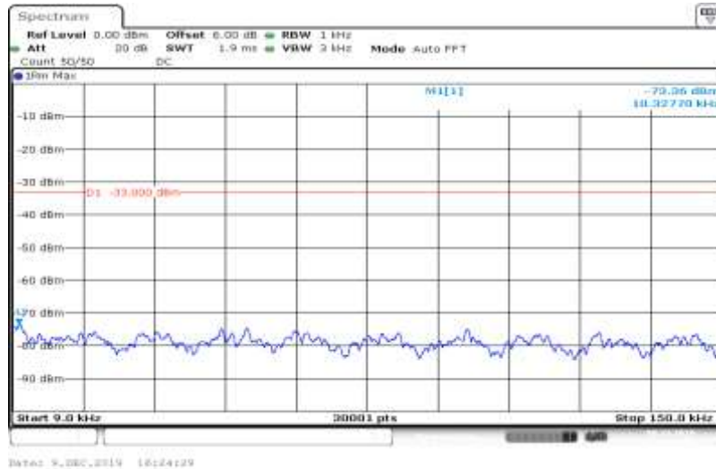
Band V-4233-HSUPA_Sub4-0.009~0.15
