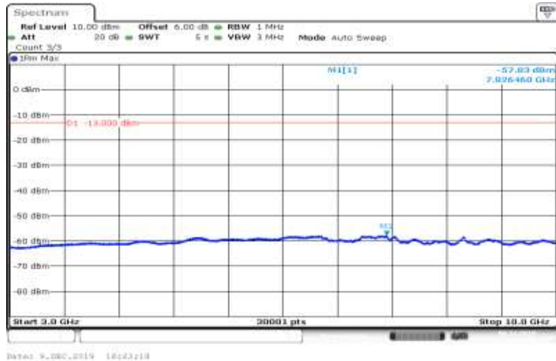
Band V-4233-HSUPA_Sub4-3000~10000
