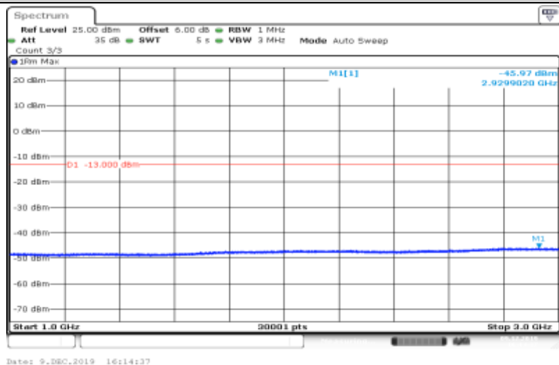
Band V-4233-HSUPA_Sub5-1000~3000
