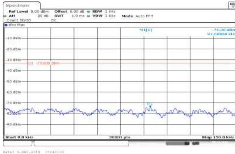
Band V-4132-HSUPA_Sub3-0.009~0.15
