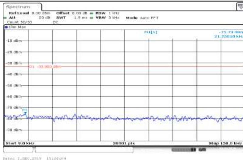
Band V-4182-HSDPA_Sub3-0.009~0.15
