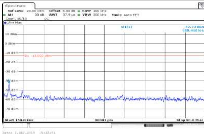
Band V-4182-HSDPA_Sub2-0.15~30
