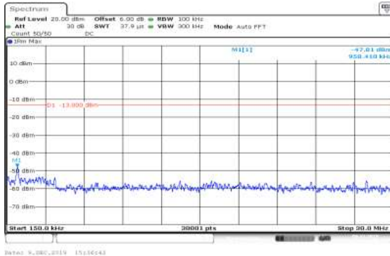
Band V-4132-HSUPA_Sub2-0.15~30
