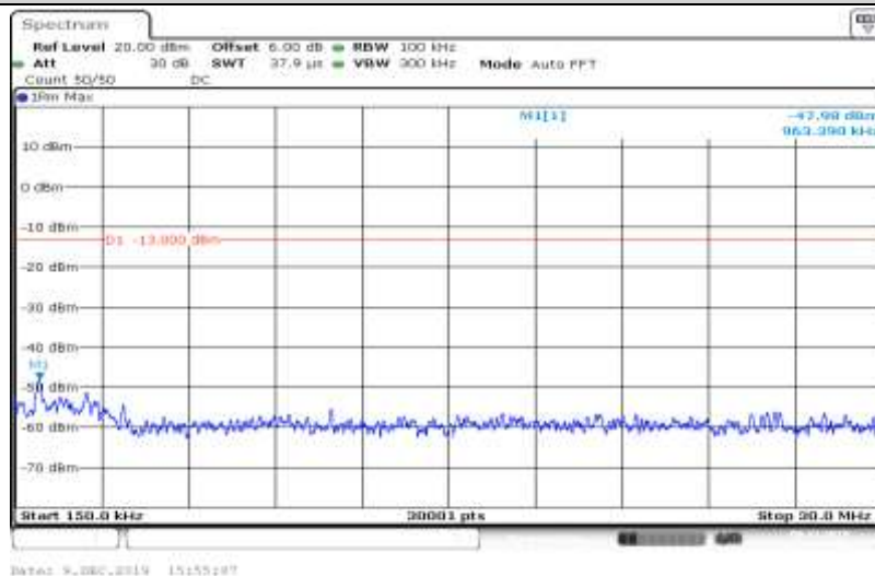
Band V-4182-HSUPA_Sub3-0.15~30
