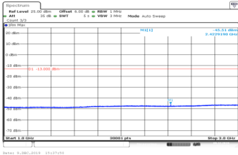
Band V-4132-HSUPA_Sub4-1000~3000
