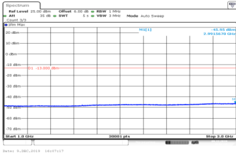
Band V-4182-HSUPA_Sub4-1000~3000
