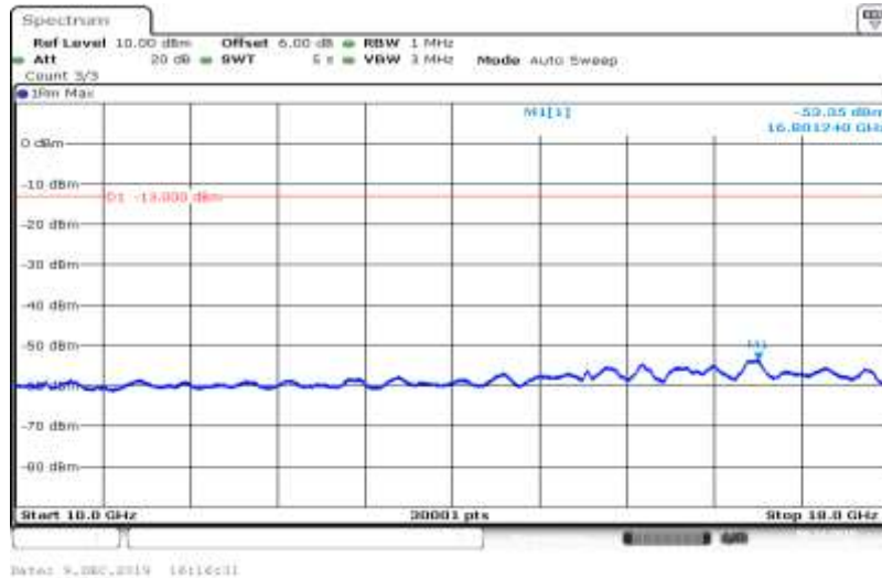
Band V-4233-HSUPA_Sub3-10000~18000
