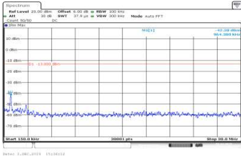
Band V-4182-HSDPA_Sub4-0.15~30
