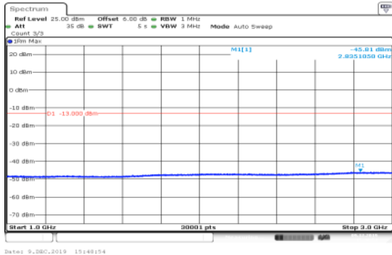
Band V-4132-HSUPA_Sub3-1000~3000
