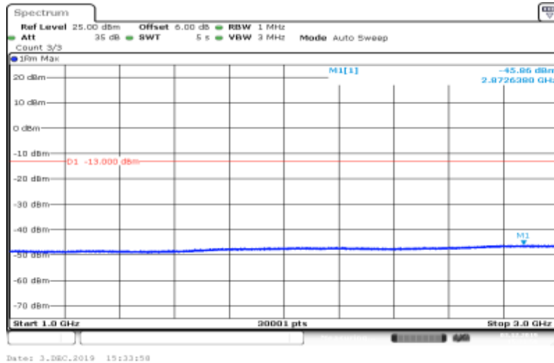
Band V-4182-HSDPA_Sub2-1000~3000
