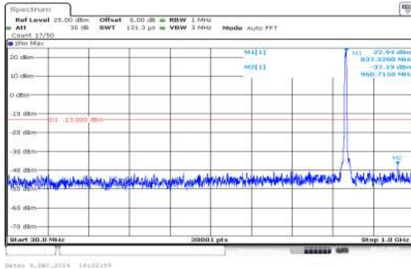
Band V-4182-HSUPA_Sub5-30~1000
