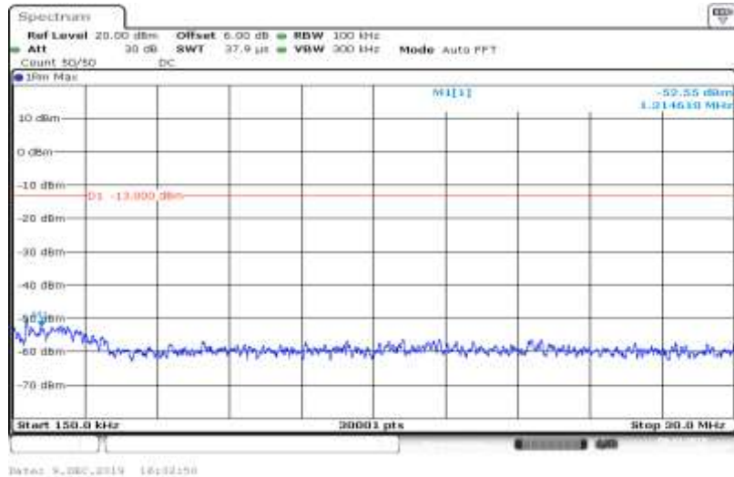
Band V-4182-HSUPA_Sub4-0.15~30
