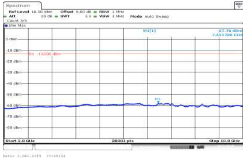
Band V-4233-HSDPA_Sub3-3000~10000
