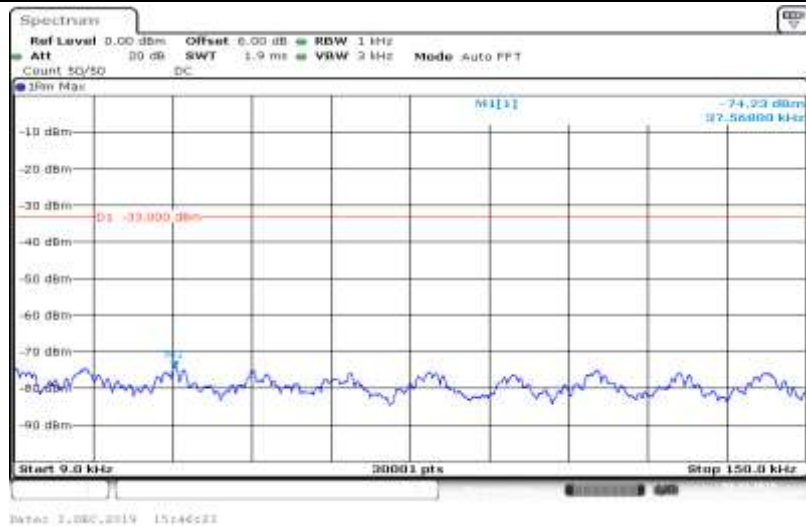
Band V-4233-HSDPA_Sub2-0.009~0.15
