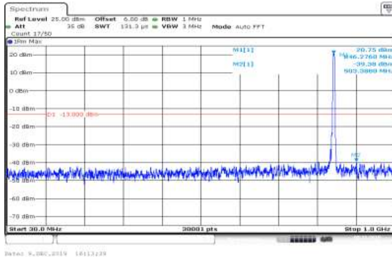
Band V-4233-HSUPA_Sub5-30~1000
