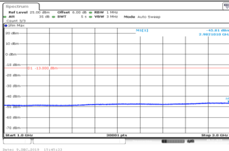
Band V-4132-HSUPA_Sub2-1000~3000
