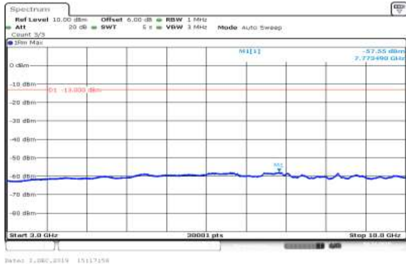
Band V-4132-HSDPA_Sub3-3000~10000
