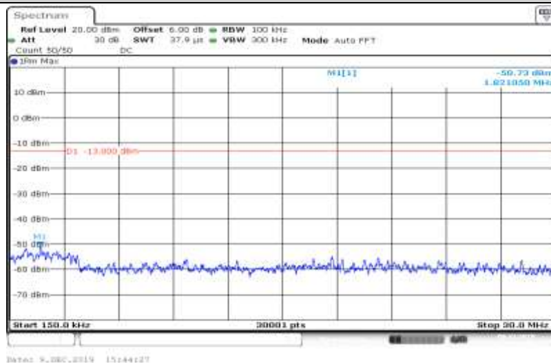
Band V-4132-HSUPA_Sub3-0.15~30
