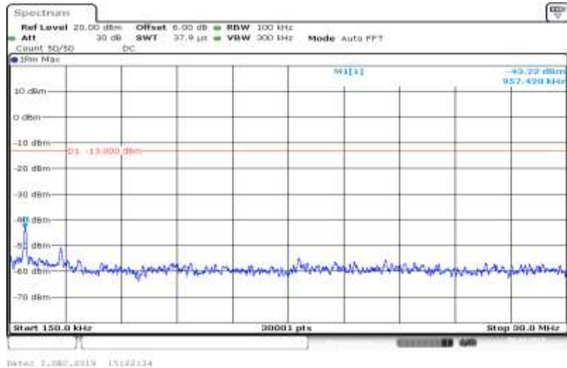
Band V-4132-HSDPA_Sub3-0.15~30
