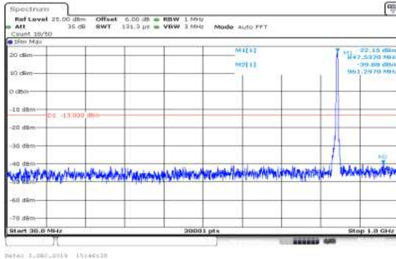
Band V-4233-HSDPA_Sub3-30~1000
