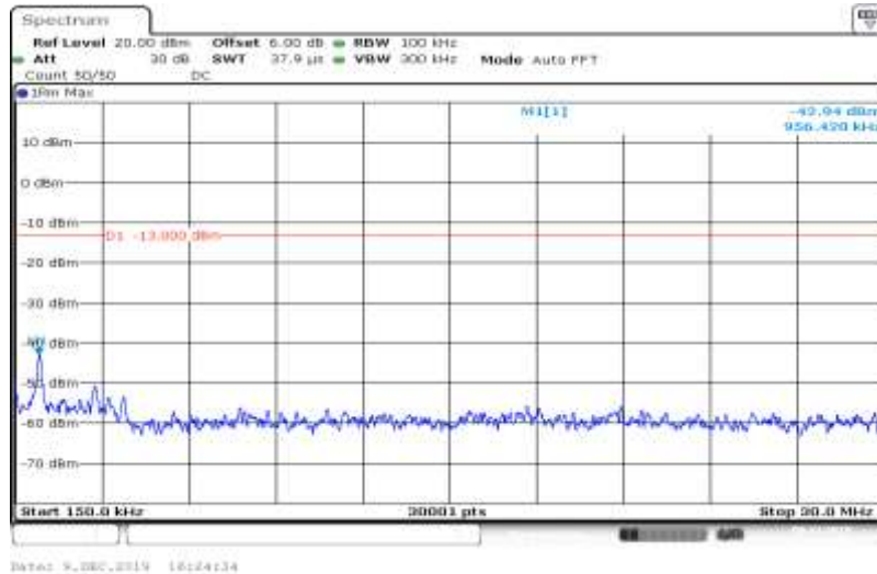
Band V-4233-HSUPA_Sub4-0.15~30
