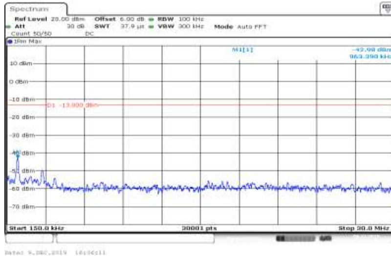
Band V-4182-HSUPA_Sub2-0.15~30
