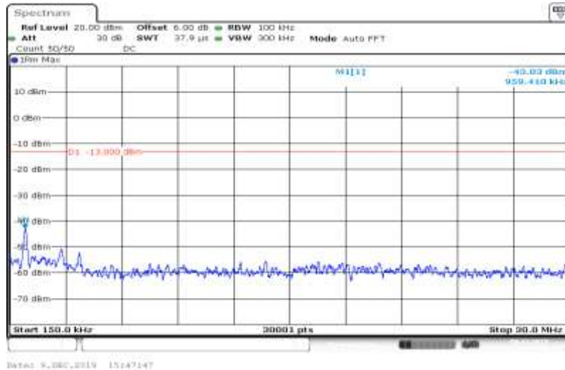
Band V-4132-HSUPA_Sub5-0.15~30
