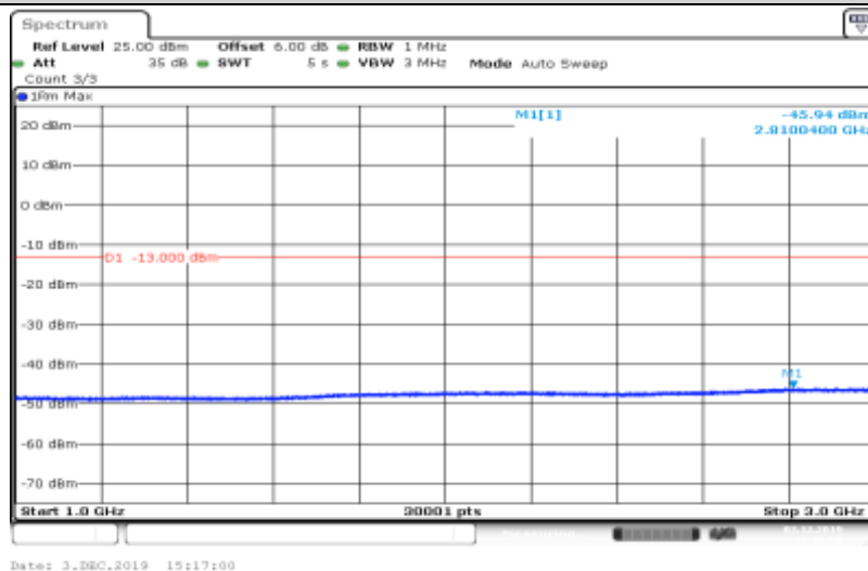
Band V-4132-HSDPA_Sub3-1000~3000
