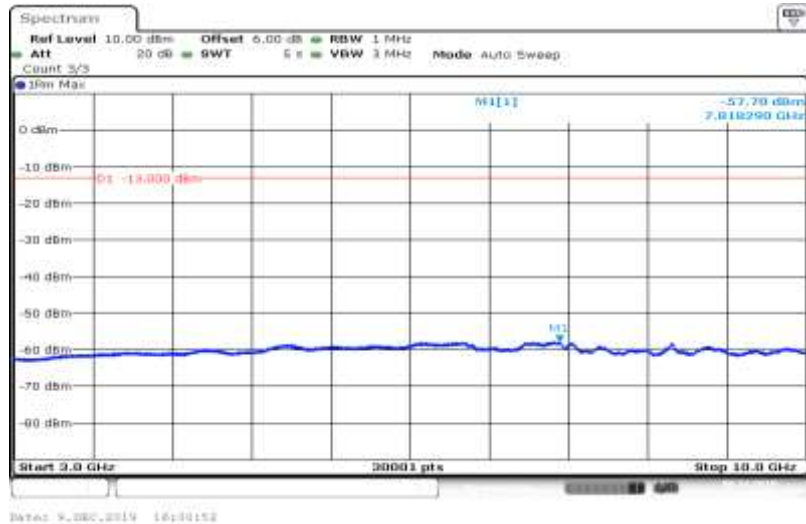
Band V-4182-HSUPA_Sub2-3000~10000
