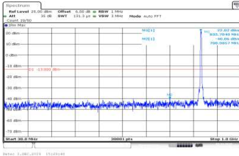
Band V-4182-HSDPA_Sub3-30~1000
