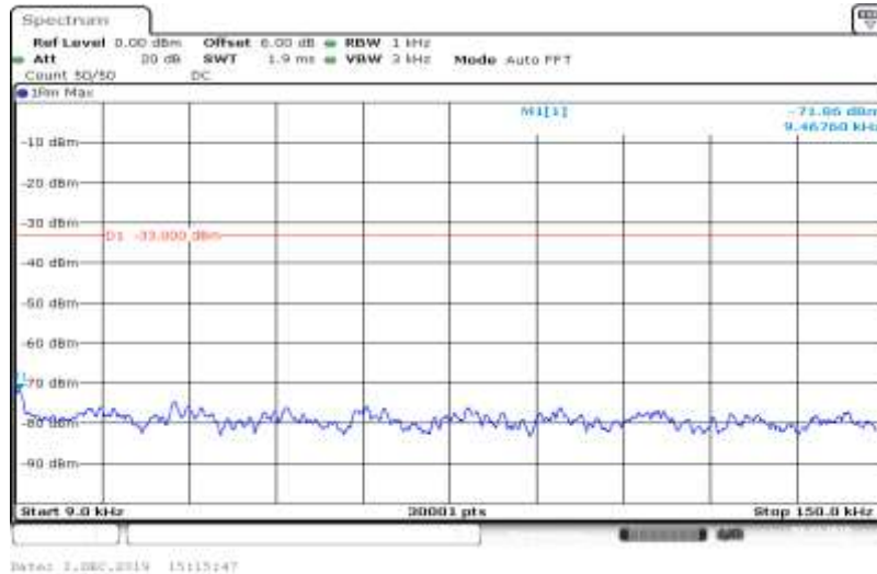
Band V-4132-HSDPA_Sub4-0.009~0.15
