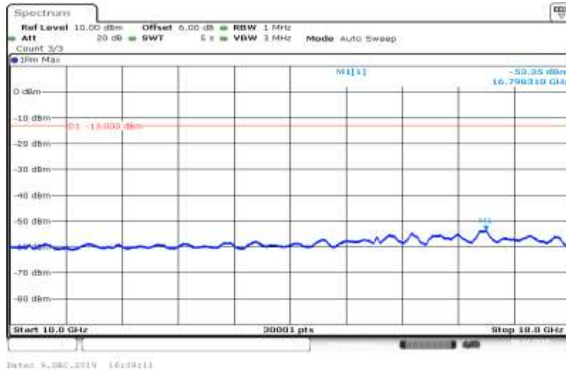
Band V-4182-HSUPA_Sub5-10000~18000
