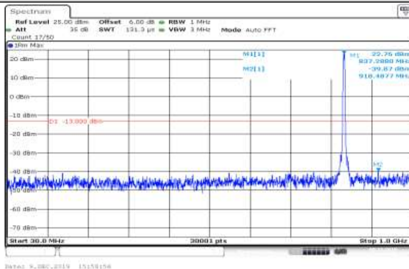
Band V-4182-HSUPA_Sub4-30~1000
