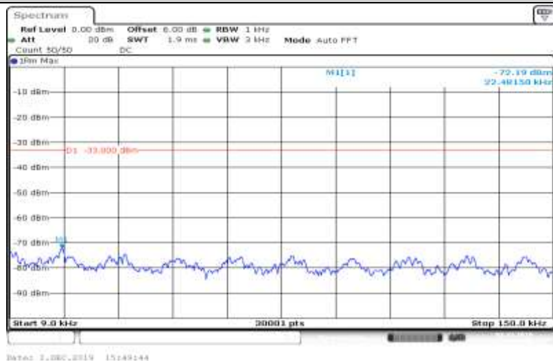
Band V-4233-HSDPA_Sub3-0.009~0.15
