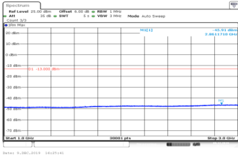
Band V-4233-HSUPA_Sub4-1000~3000
