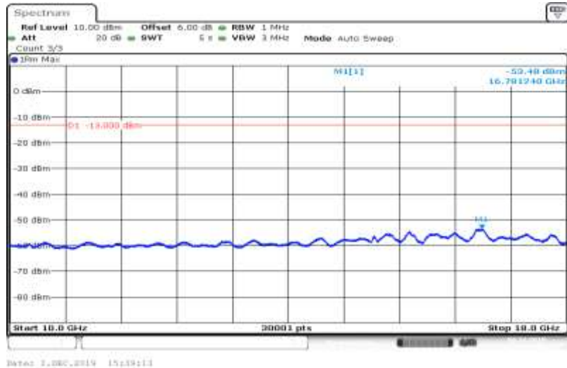
Band V-4182-HSDPA_Sub3-10000~18000
