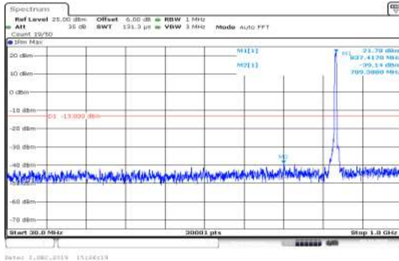
Band V-4182-HSDPA_Sub2-30~1000
