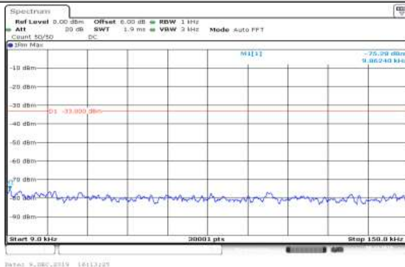
Band V-4233-HSUPA_Sub2-0.009~0.15
