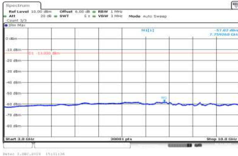
Band V-4182-HSDPA_Sub4-3000~10000
