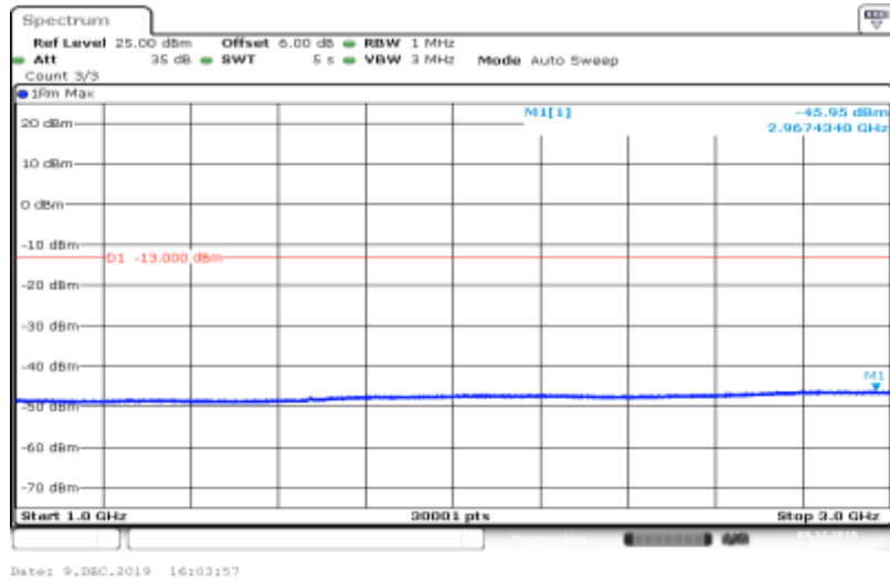
Band V-4182-HSUPA_Sub3-1000~3000
