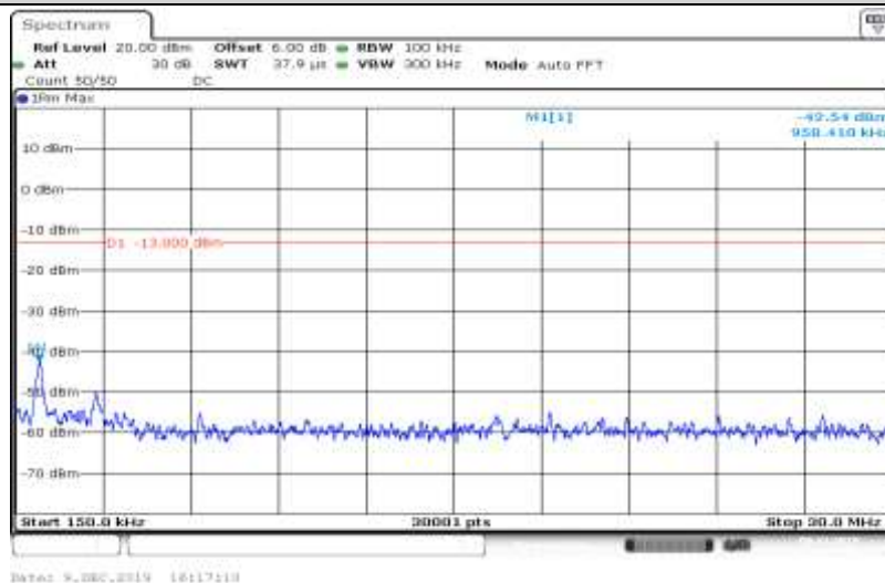
Band V-4233-HSUPA_Sub3-0.15~30
