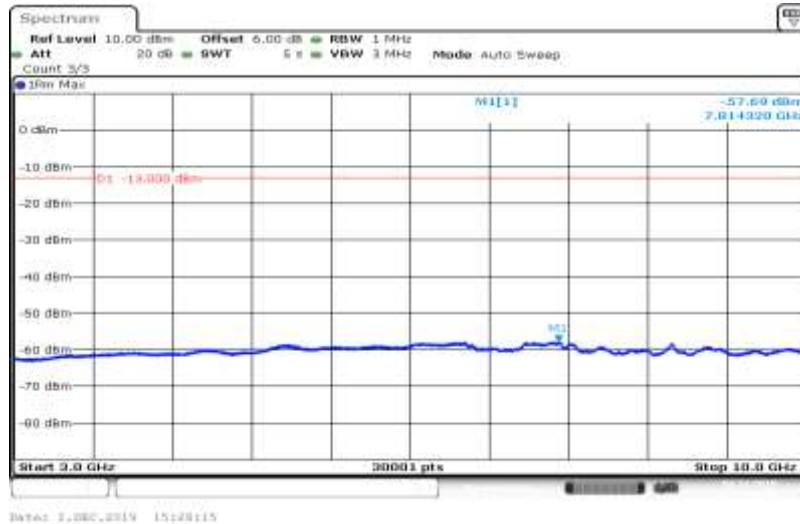
Band V-4182-HSDPA_Sub3-3000~10000
