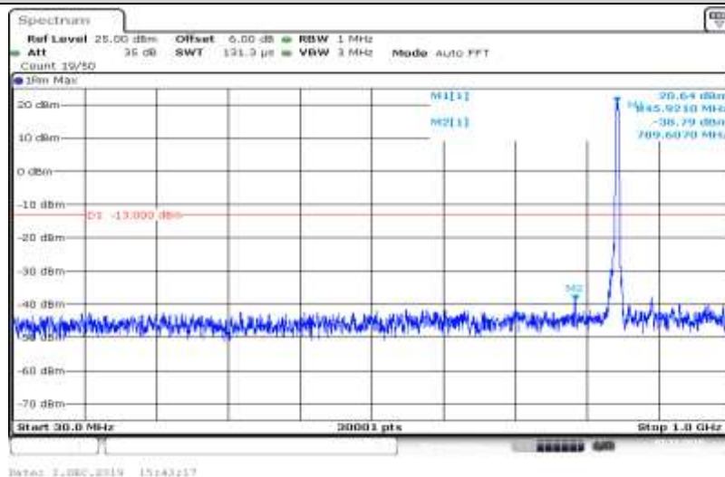
Band V-4233-HSDPA_Sub4-30~1000
