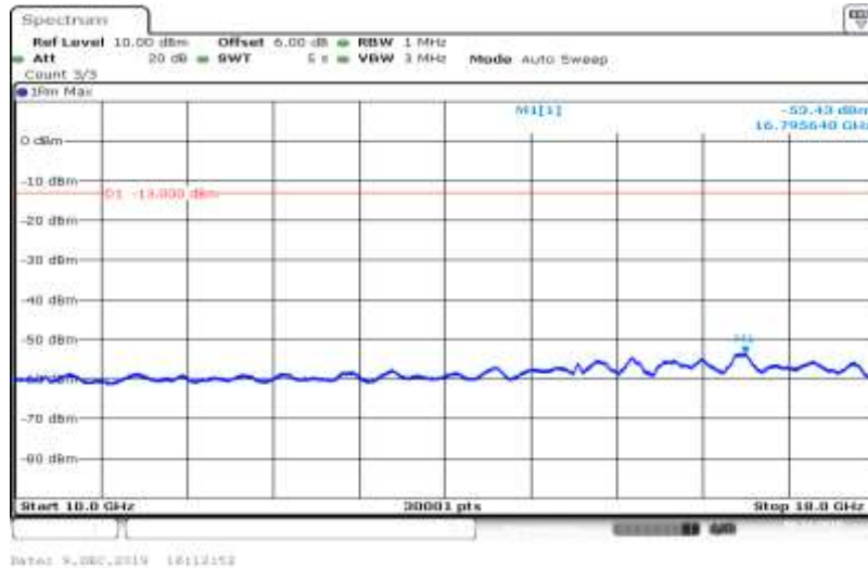
Band V-4233-HSUPA_Sub2-10000~18000
