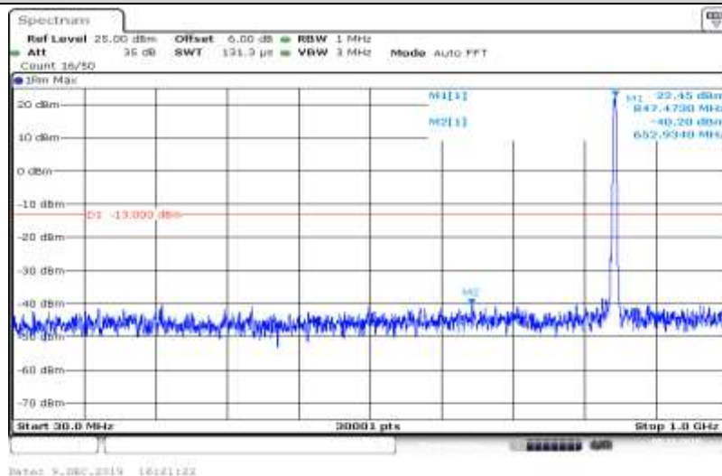
Band V-4233-HSUPA_Sub4-30~1000
