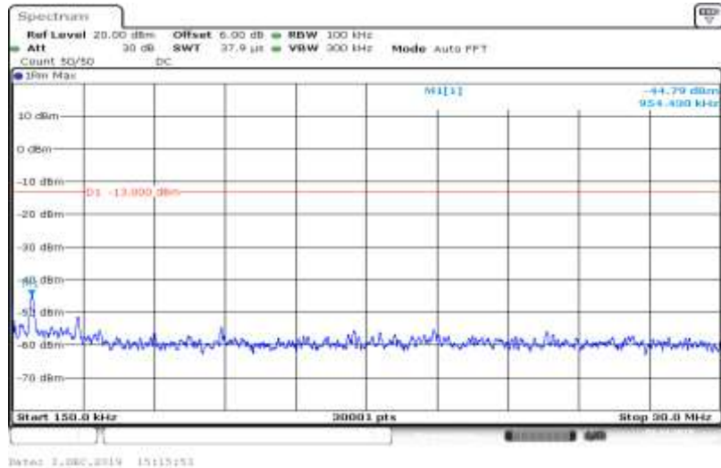
Band V-4132-HSDPA_Sub4-0.15~30
