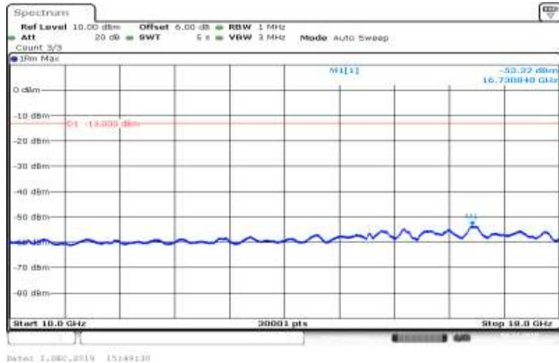
Band V-4233-HSDPA_Sub3-10000~18000
