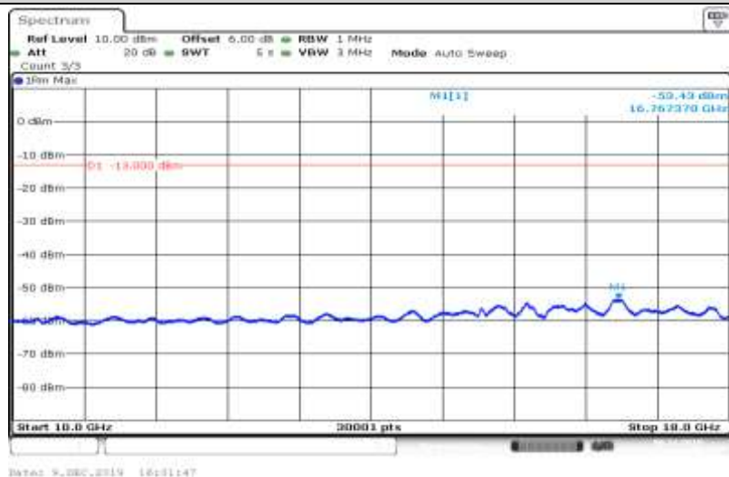
Band V-4182-HSUPA_Sub4-10000~18000
