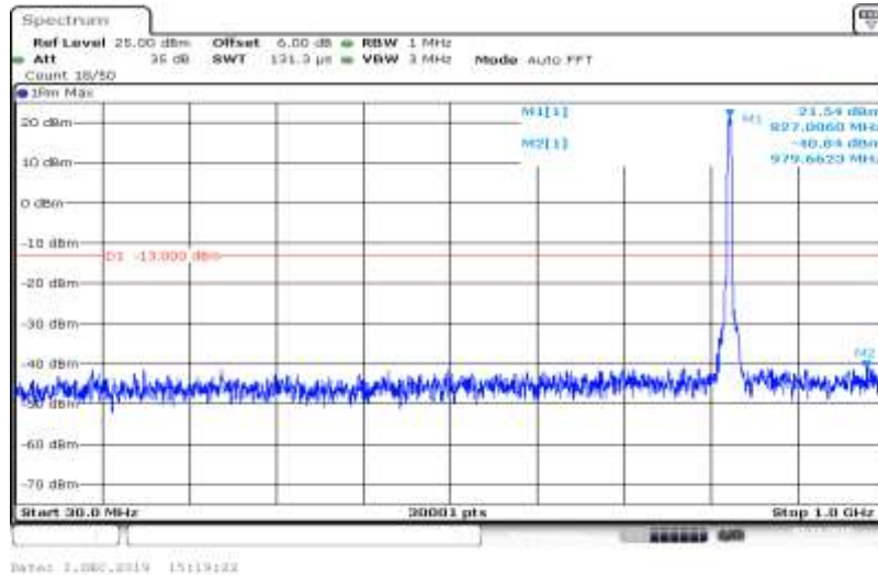
Band V-4132-HSDPA_Sub3-30~1000
