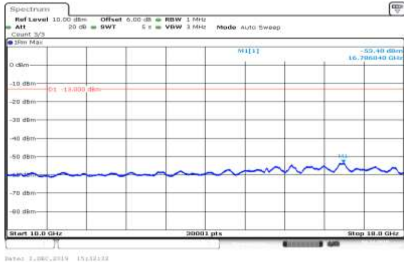
Band V-4182-HSDPA_Sub2-10000~18000
