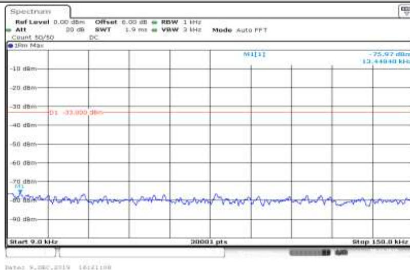
Band V-4233-HSUPA_Sub5-0.009~0.15
