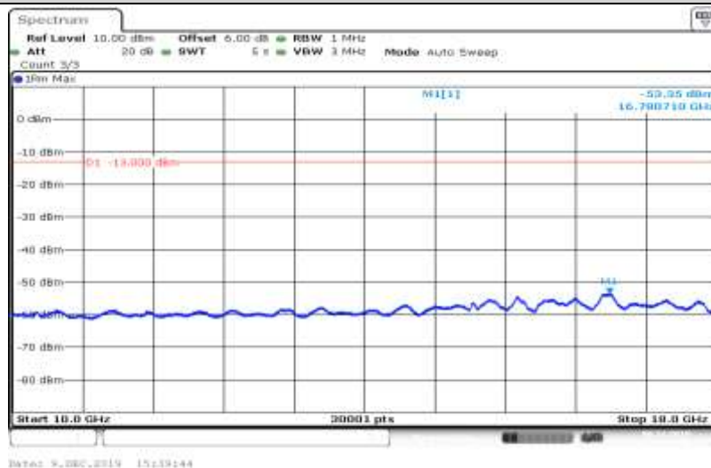
Band V-4132-HSUPA_Sub4-10000~18000
