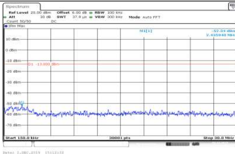
Band V-4132-HSDPA_Sub2-0.15~30
