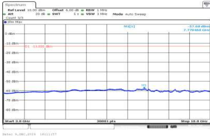
Band V-4233-HSUPA_Sub5-3000~10000
