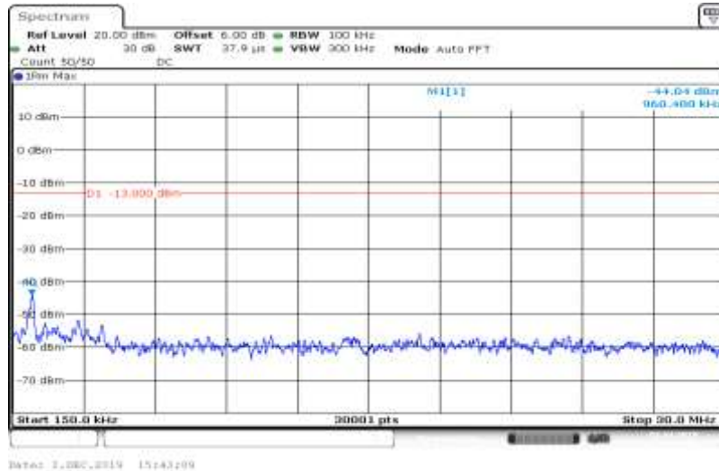
Band V-4233-HSDPA_Sub3-0.15~30
