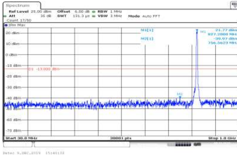
Band V-4132-HSUPA_Sub5-30~1000
