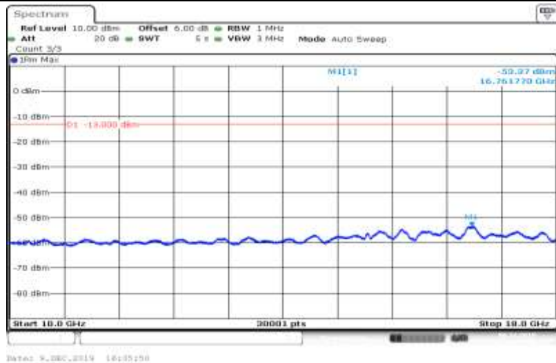
Band V-4182-HSUPA_Sub2-10000~18000
