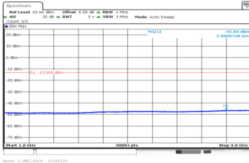
Band V-4132-HSDPA_Sub4-1000~3000
