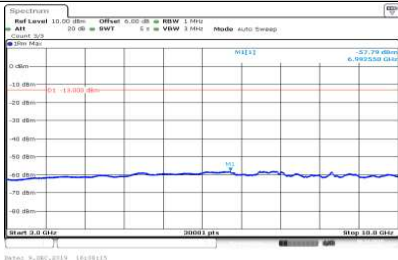
Band V-4182-HSUPA_Sub3-3000~10000
