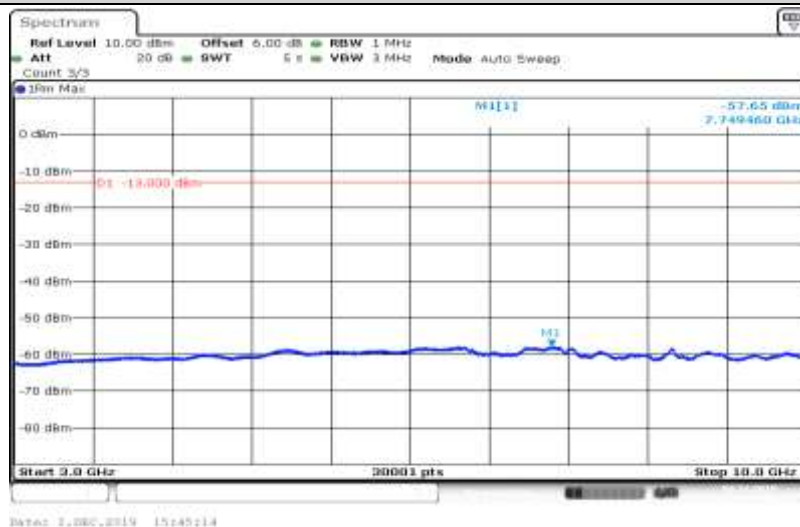
Band V-4233-HSDPA_Sub2-3000~10000
