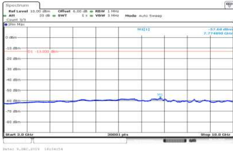
Band V-4182-HSUPA_Sub5-3000~10000
