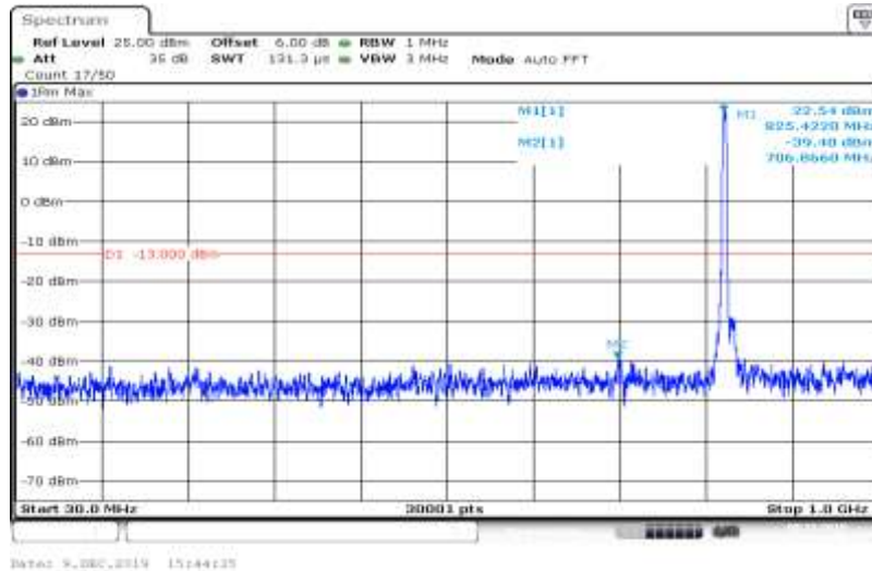
Band V-4132-HSUPA_Sub2-30~1000
