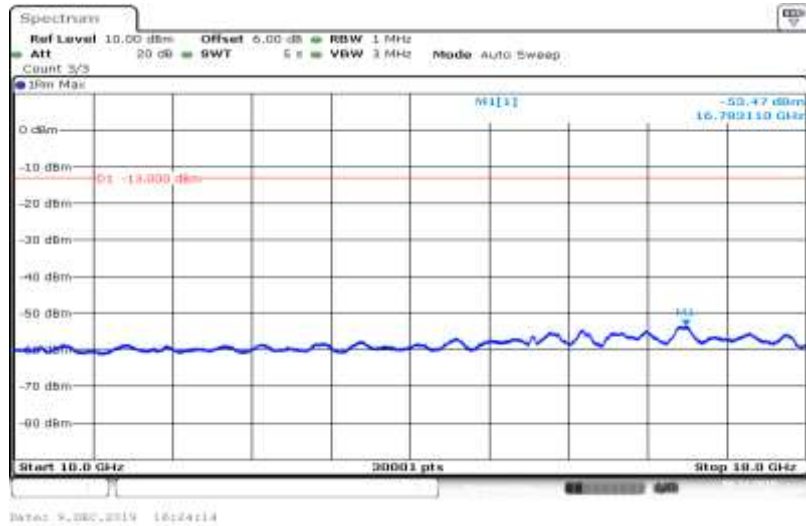
Band V-4233-HSUPA_Sub5-10000~18000
