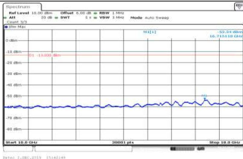
Band V-4233-HSDPA_Sub4-10000~18000
