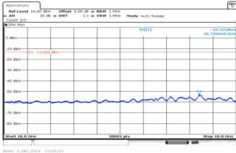
Band V-4132-HSDPA_Sub2-10000~18000
