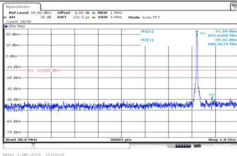
Band V-4132-HSDPA_Sub4-30~1000
