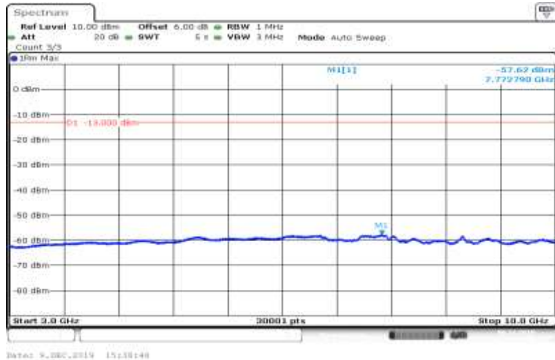
Band V-4132-HSUPA_Sub5-3000~10000
