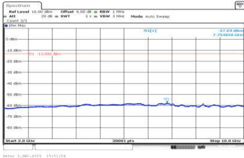
Band V-4233-HSDPA_Sub4-3000~10000
