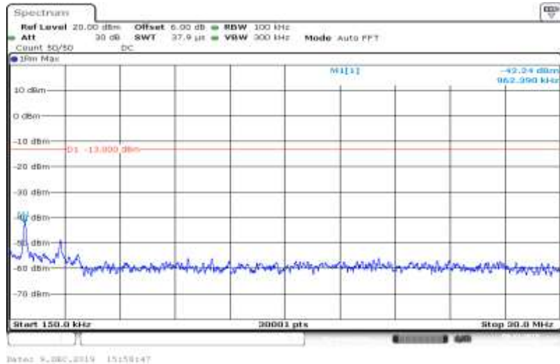
Band V-4182-HSUPA_Sub5-0.15~30
