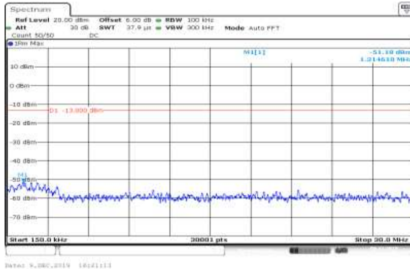
Band V-4233-HSUPA_Sub2-0.15~30
