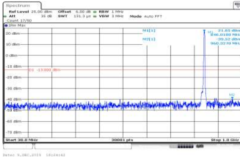
Band V-4233-HSUPA_Sub3-30~1000
