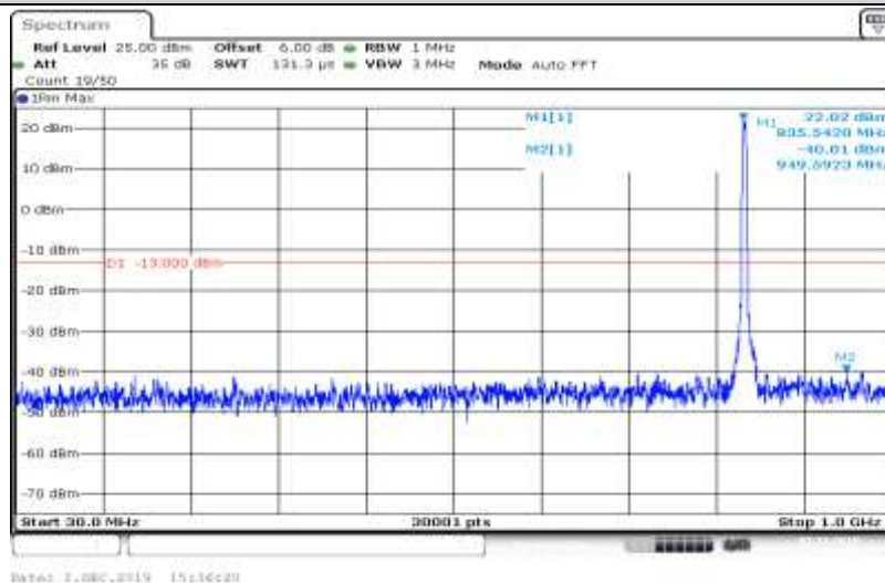
Band V-4182-HSDPA_Sub4-30~1000
