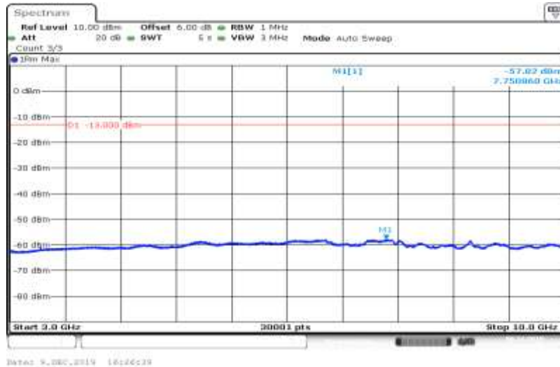
Band V-4233-HSUPA_Sub2-3000~10000
