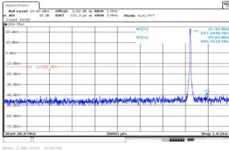
Band V-4132-HSDPA_Sub2-30~1000
