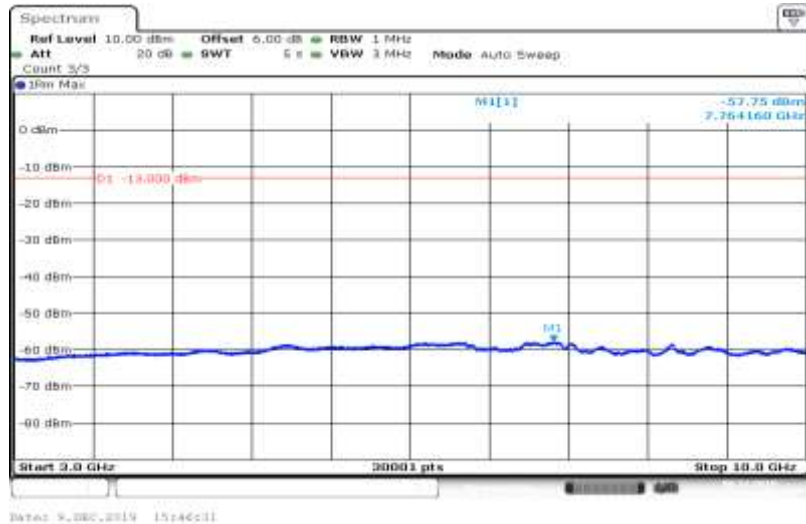
Band V-4132-HSUPA_Sub2-3000~10000
