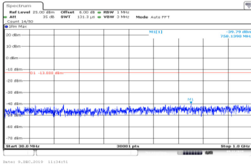
Band IV-1413-HSUPA_Sub3-30~1000
