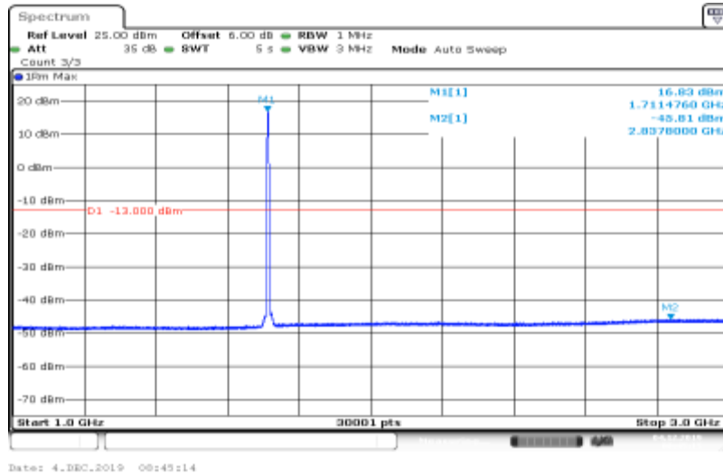
Band IV-1312-HSDPA_Sub2-1000~3000
