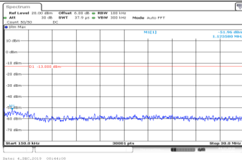
Band IV-1312-HSDPA_Sub2-0.15~30
