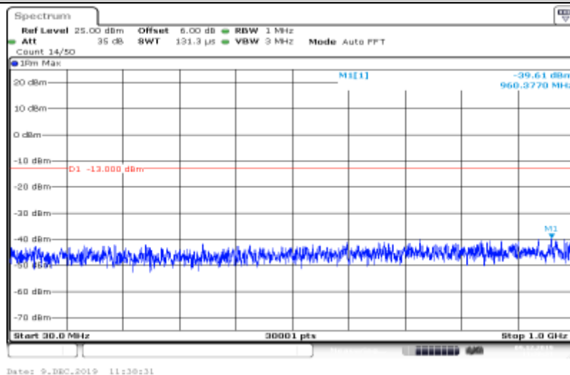
Band IV-1413-HSUPA_Sub4-30~1000
