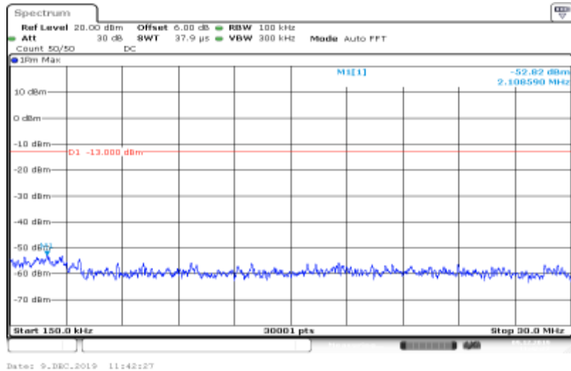
Band IV-1413-HSUPA_Sub4-0.15~30
