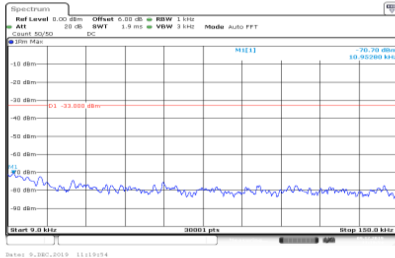
Band IV-1312-HSUPA_Sub3-0.009~0.15
