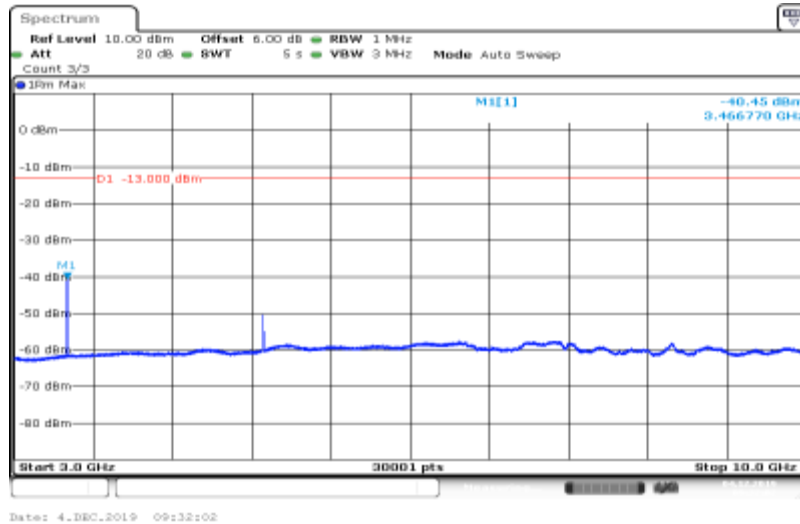
Band IV-1413-HSDPA_Sub4-3000~10000
