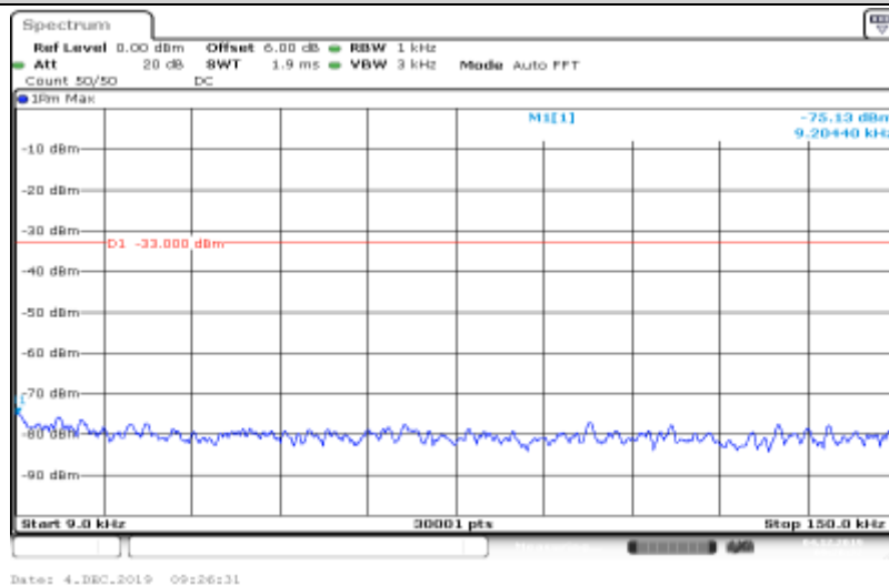
Band IV-1413-HSDPA_Sub3-0.009~0.15
