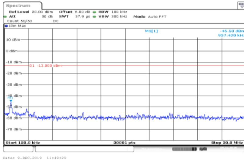
Band IV-1513-HSUPA_Sub5-0.15~30
