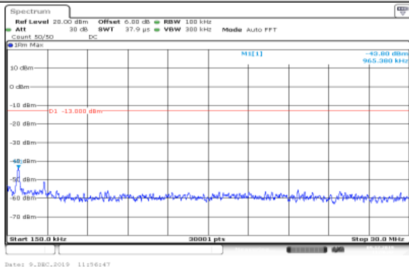
Band IV-1513-HSUPA_Sub3-0.15~30
