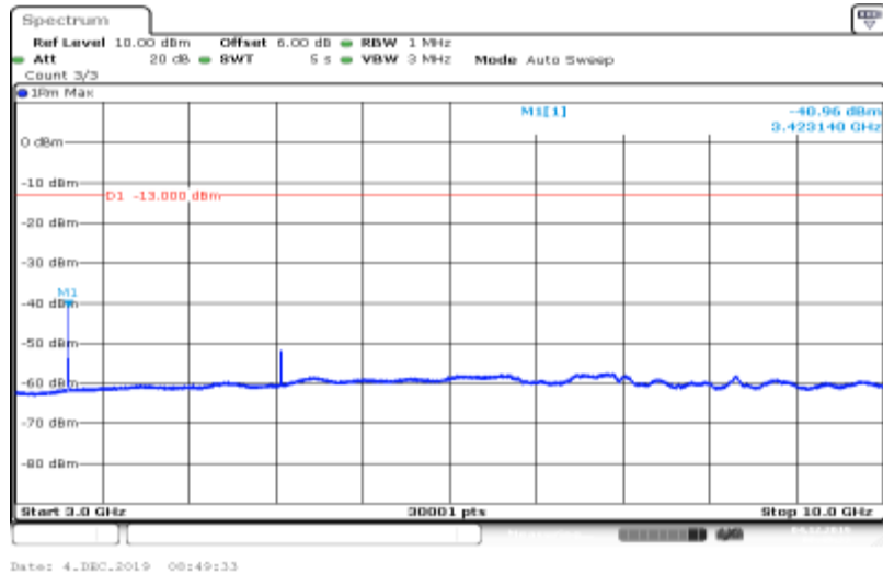
Band IV-1312-HSDPA_Sub3-3000~10000
