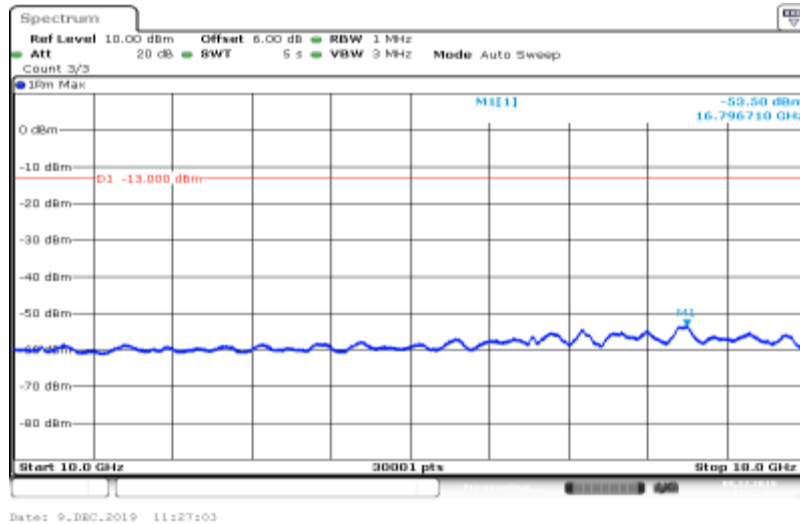
Band IV-1312-HSUPA_Sub3-10000~18000
