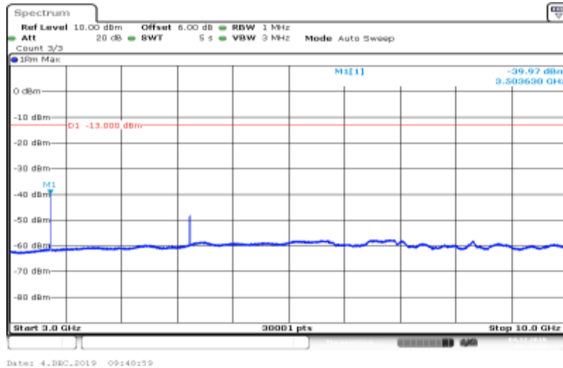
Band IV-1513-HSDPA_Sub3-3000~10000
