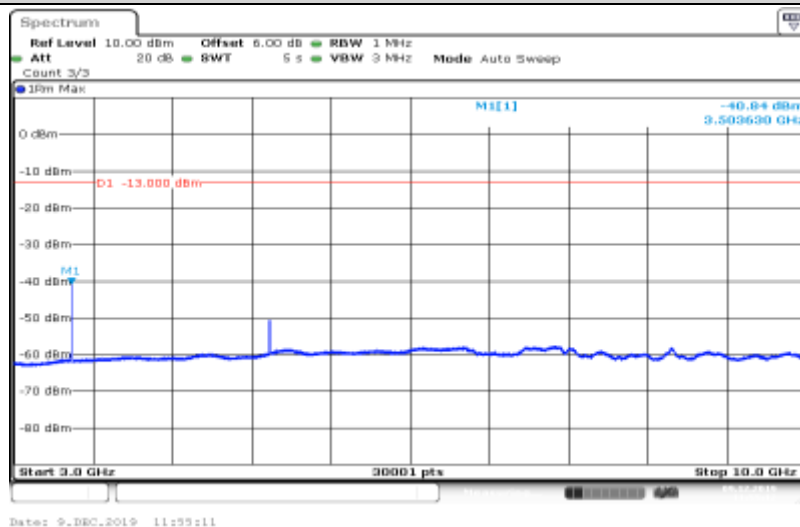
Band IV-1513-HSUPA_Sub3-3000~10000
