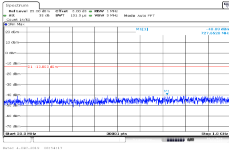
Band IV-1312-HSDPA_Sub2-30~1000
