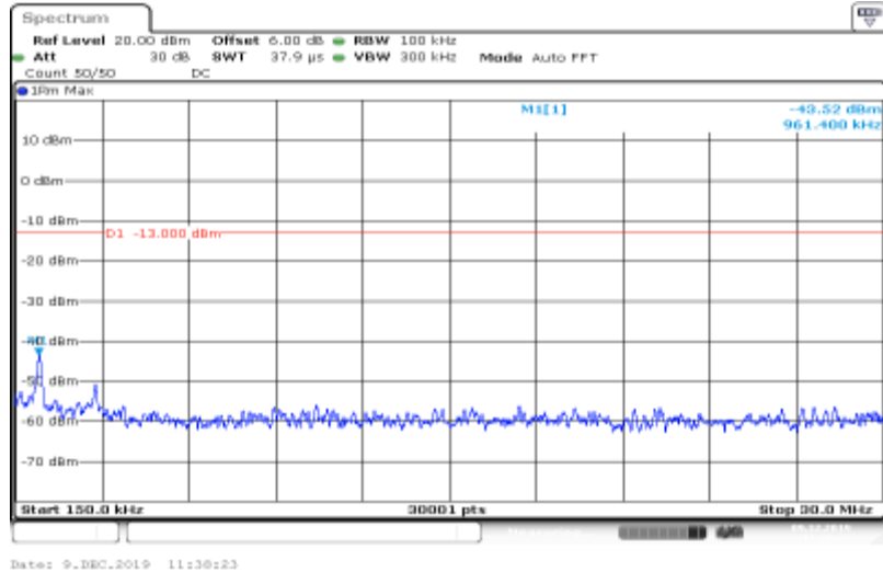
Band IV-1413-HSUPA_Sub5-0.15~30
