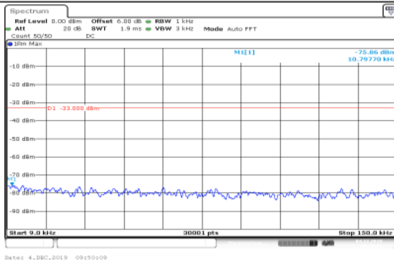
Band IV-1513-HSDPA_Sub3-0.009~0.15
