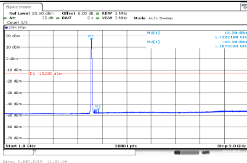
Band IV-1312-HSUPA_Sub5-1000~3000
