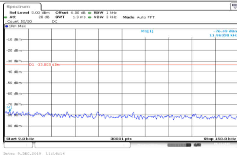
Band IV-1312-HSUPA_Sub5-0.009~0.15
