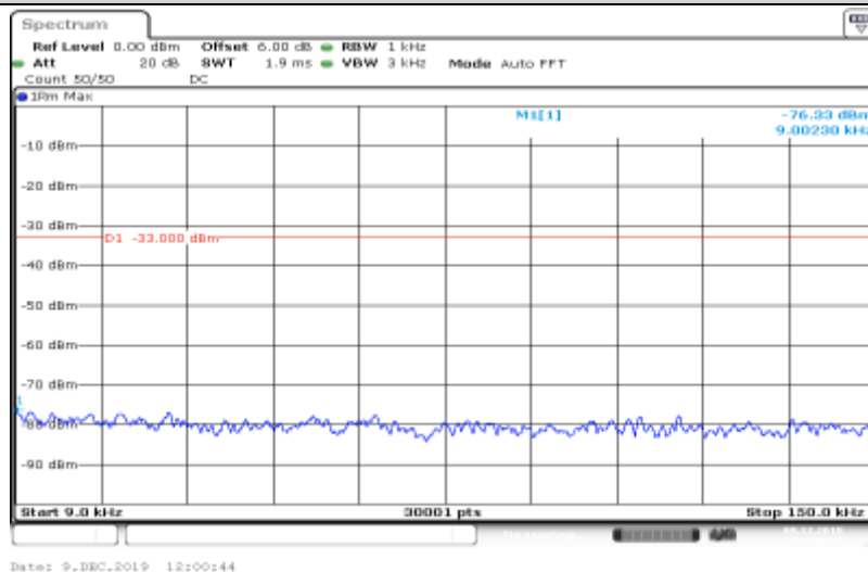
Band IV-1513-HSUPA_Sub5-0.009~0.15
