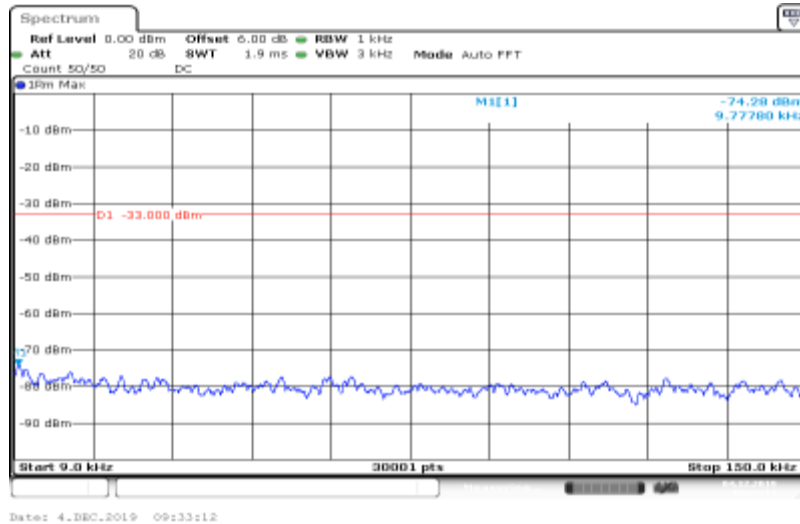
Band IV-1413-HSDPA_Sub2-0.009~0.15
