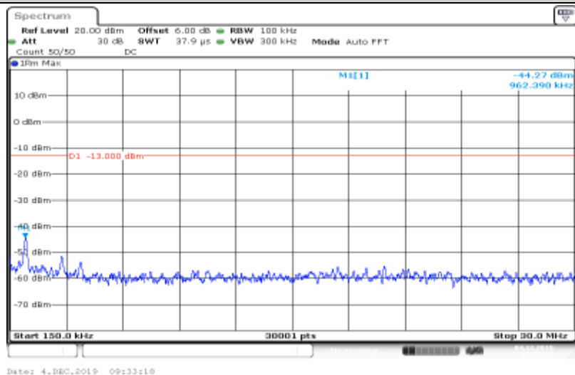
Band IV-1413-HSDPA_Sub2-0.15~30
