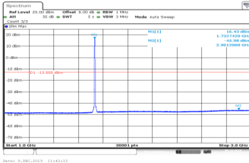
Band IV-1413-HSUPA_Sub3-1000~3000
