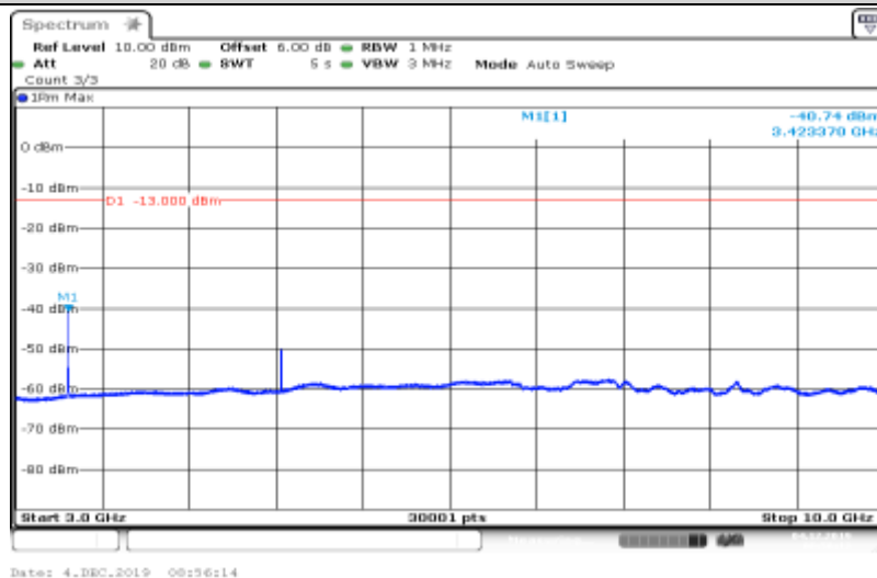
Band IV-1312-HSDPA_Sub2-3000~10000
