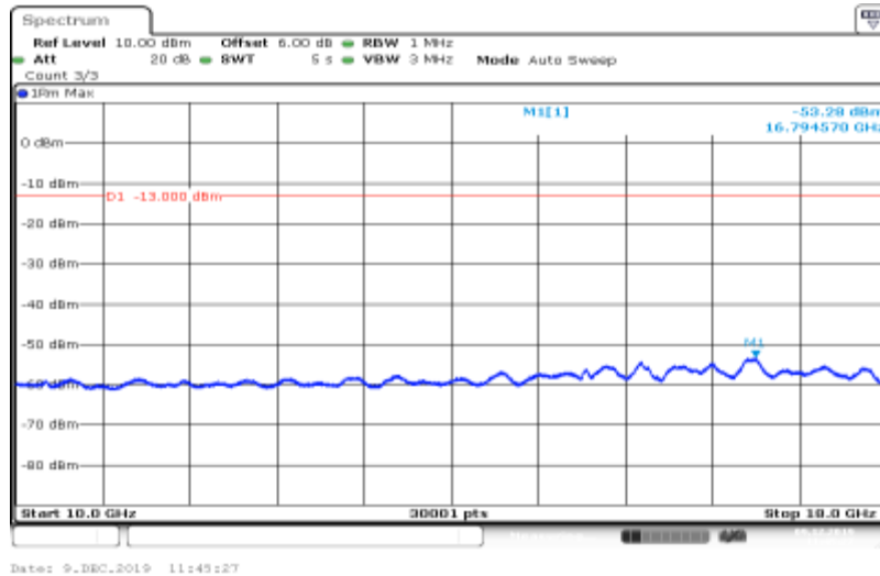
Band IV-1413-HSUPA_Sub2-10000~18000
