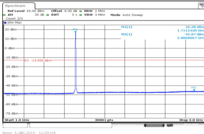
Band IV-1312-HSUPA_Sub2-1000~3000
