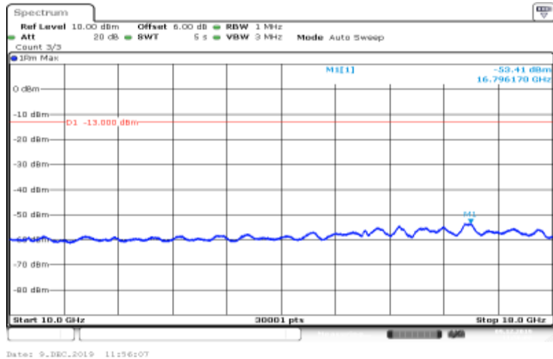
Band IV-1513-HSUPA_Sub3-10000~18000
