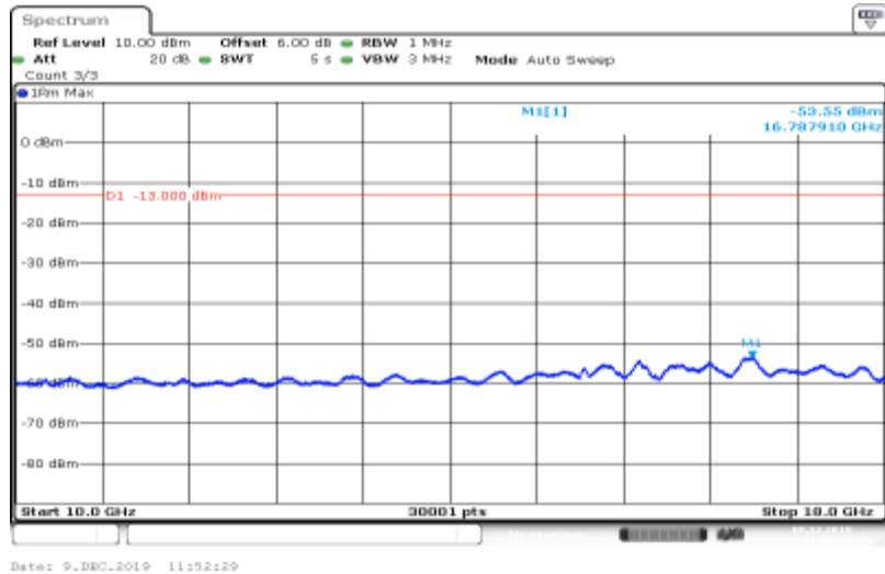
Band IV-1513-HSUPA_Sub2-10000~18000
