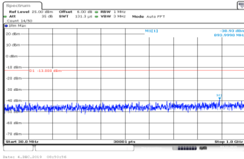
Band IV-1312-HSDPA_Sub3-30~1000
