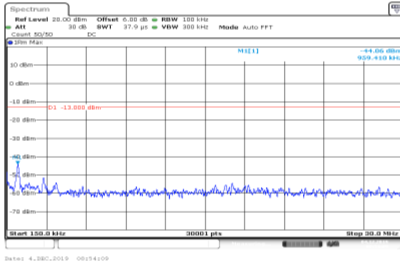
Band IV-1312-HSDPA_Sub3-0.15~30
