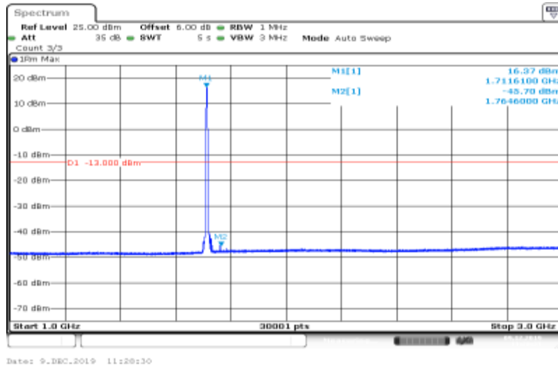
Band IV-1312-HSUPA_Sub3-1000~3000
