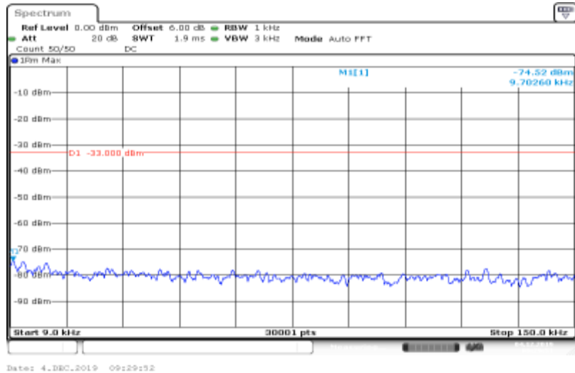
Band IV-1413-HSDPA_Sub4-0.009~0.15
