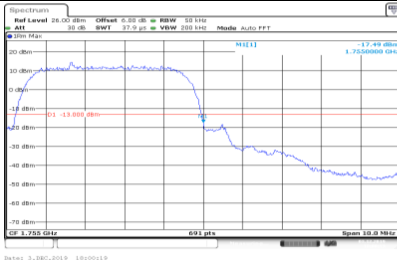
Band IV-1513-HSDPA_Sub3
