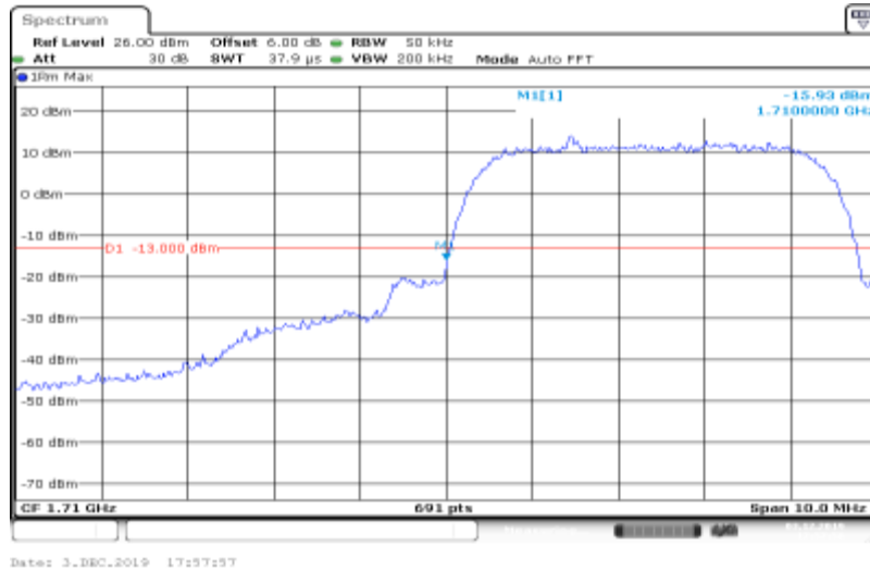
Band IV-1312-HSDPA_Sub3
