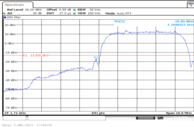
Band IV-1312-HSDPA_Sub1
