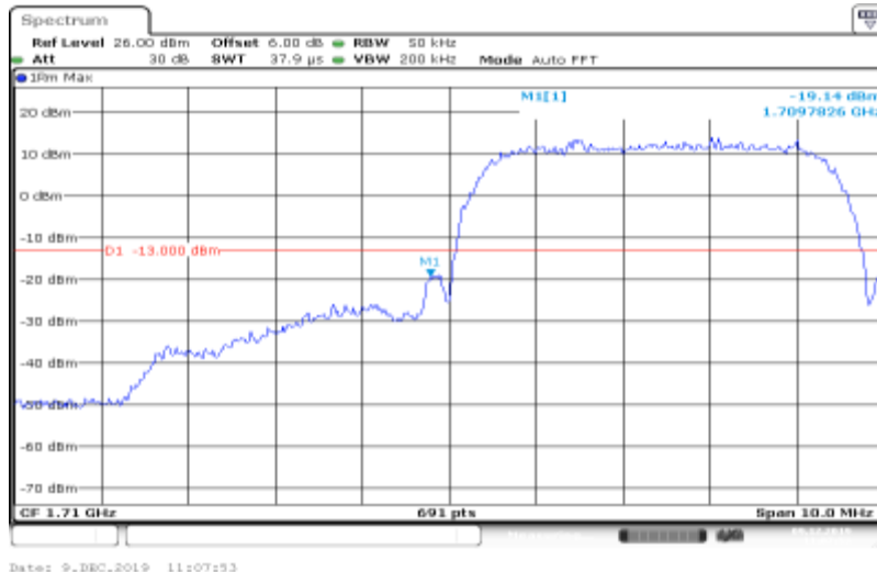
Band IV-1312-HSUPA_Sub5
