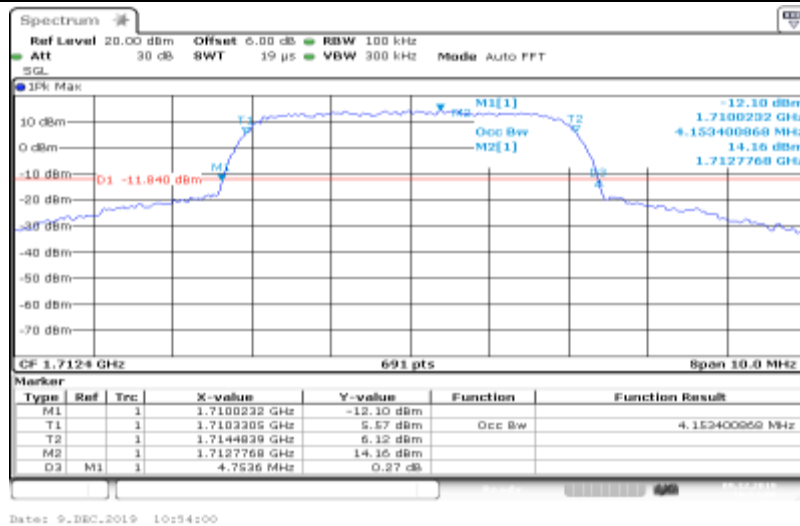
Band IV-1312-HSUPA_Sub4
