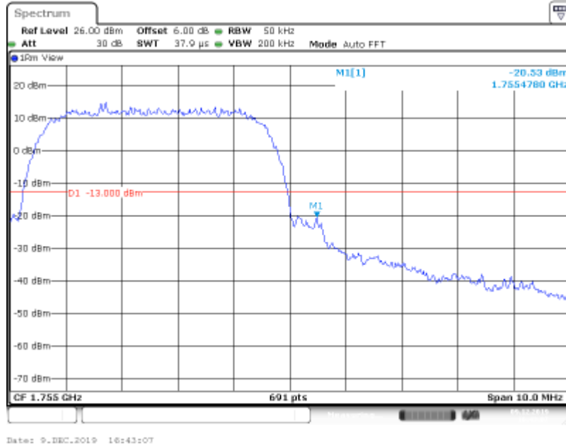
Band IV-1513-HSUPA_Sub4
