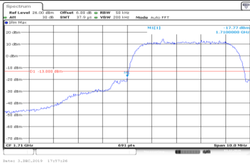
Band IV-1312-HSDPA_Sub2
