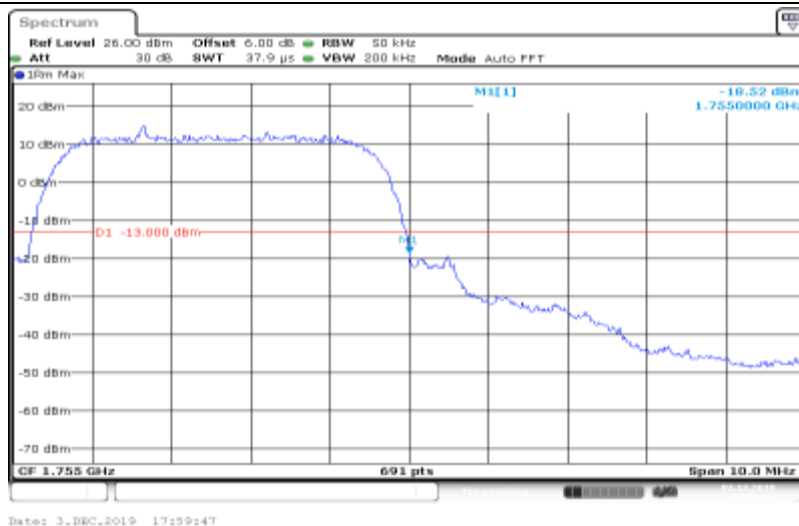
Band IV-1513-HSDPA_Sub2
