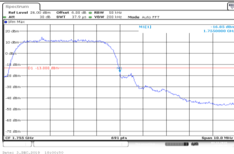
Band IV-1513-HSDPA_Sub3
