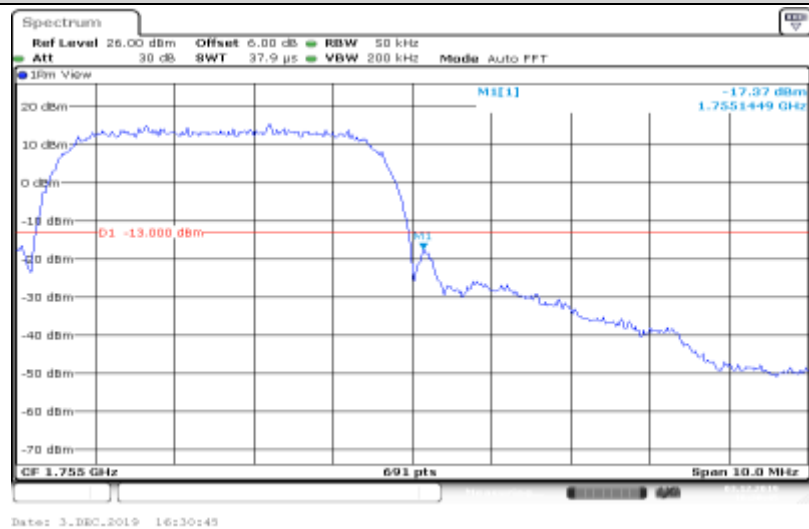
Band IV-1513
