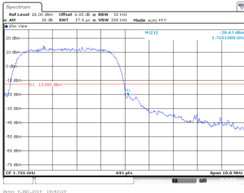
Band IV-1513-HSUPA_Sub5
