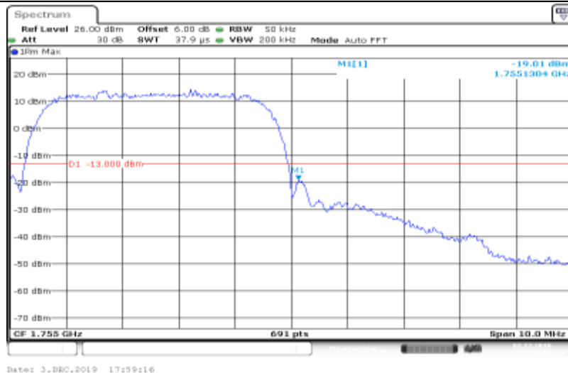
Band IV-1513-HSDPA_Sub1
