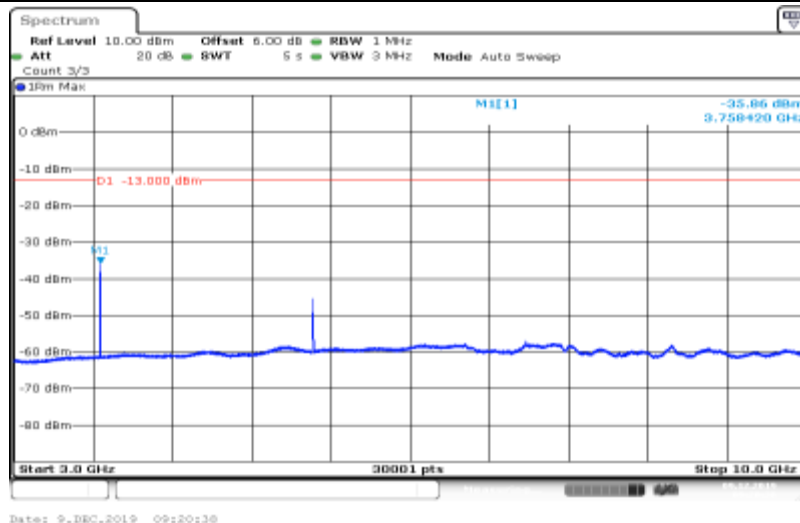
Band II-9400-HSUPA_Sub3-3000~10000
