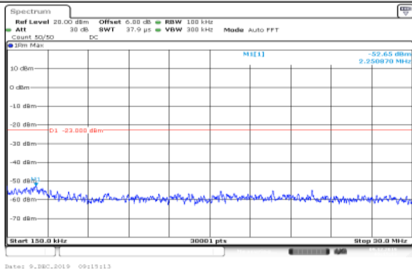
Band II-9400-HSUPA_Sub3-0.15~30
