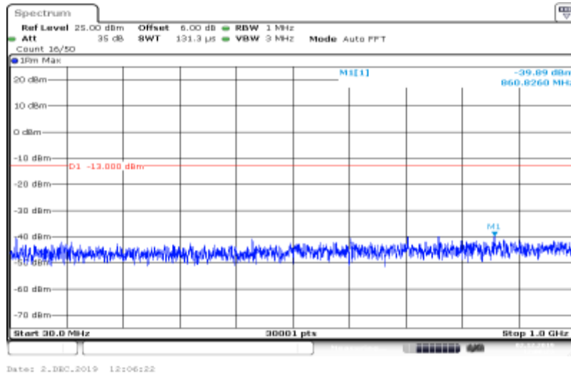
Band II-9538-HSDPA_Sub3-30~1000
