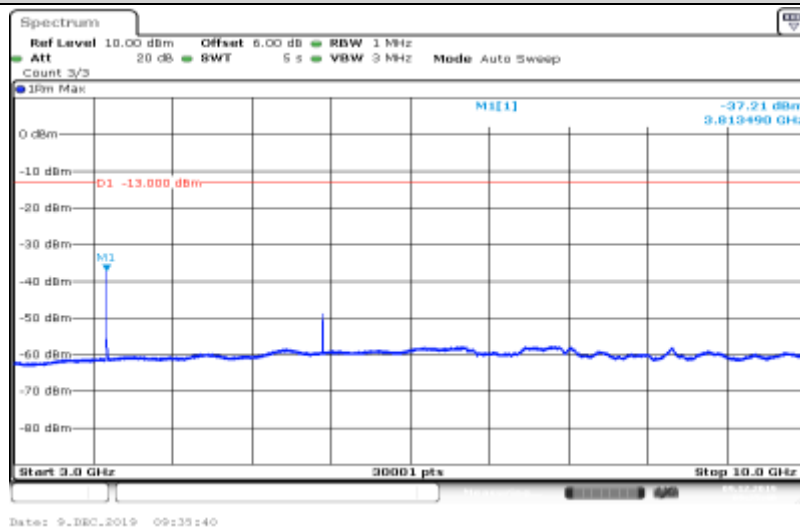
Band II-9538-HSUPA_Sub3-3000~10000
