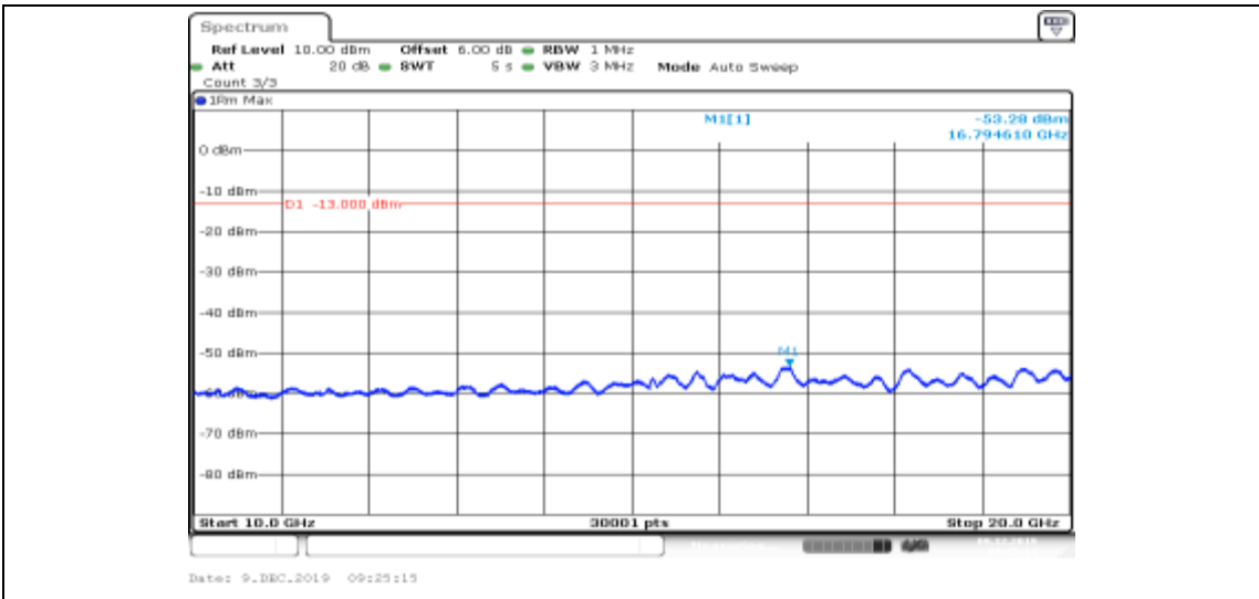
Band II-9538-HSUPA_Sub2-10000~20000
