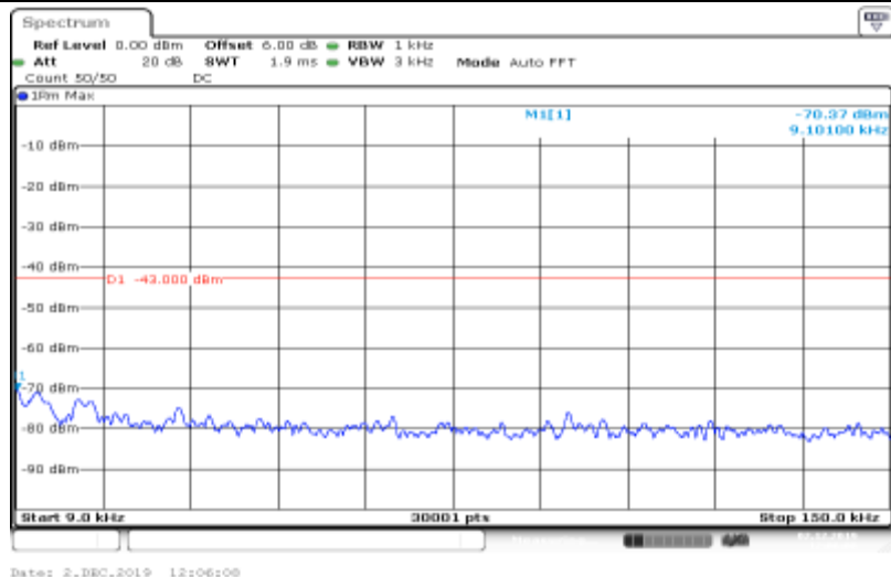
Band II-9538-HSDPA_Sub2-0.009~0.15
