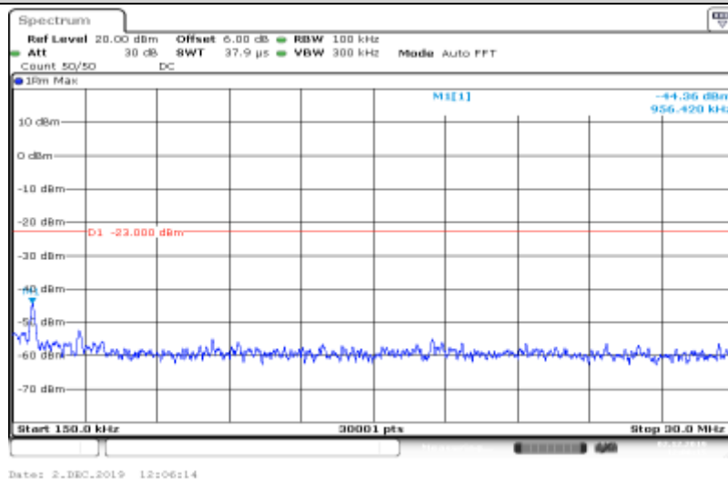
Band II-9538-HSDPA_Sub3-0.15~30
