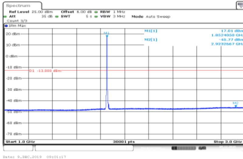
Band II-9262-HSUPA_Sub3-1000~3000
