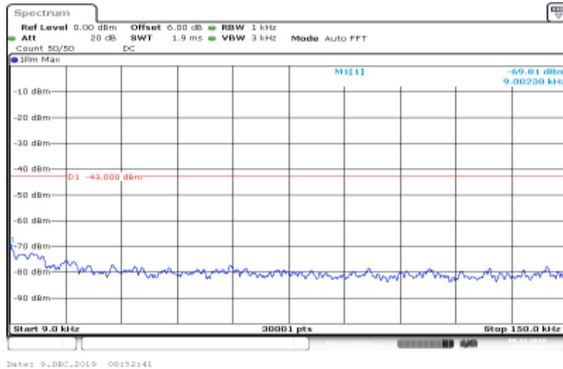
Band II-9262-HSUPA_Sub3-0.009~0.15
