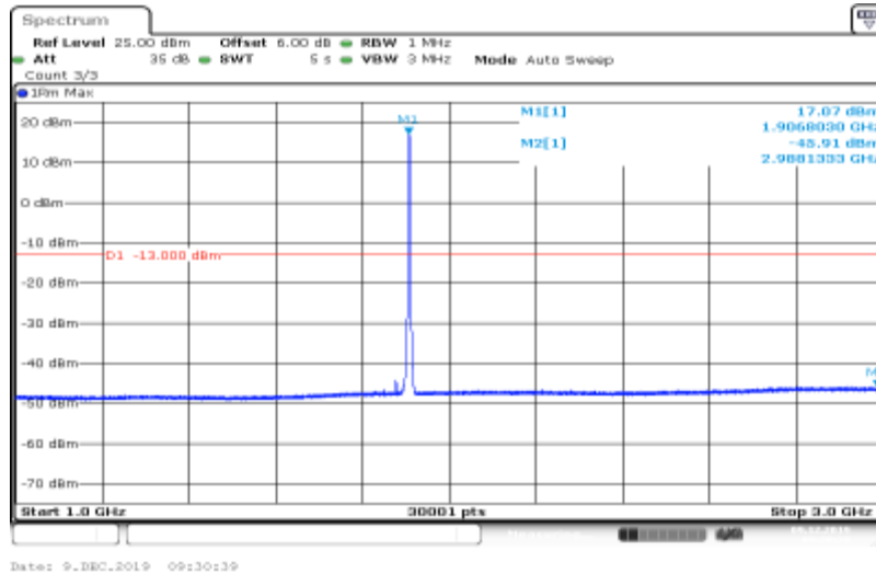
Band II-9538-HSUPA_Sub3-1000~3000
