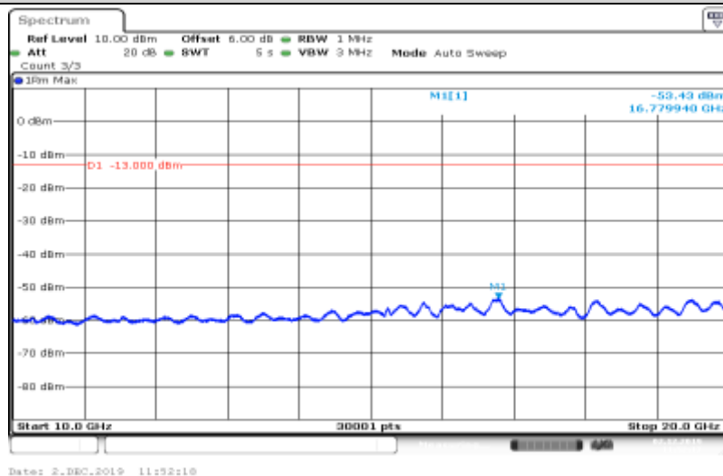
Band II-9400-HSDPA_Sub1-10000~20000
