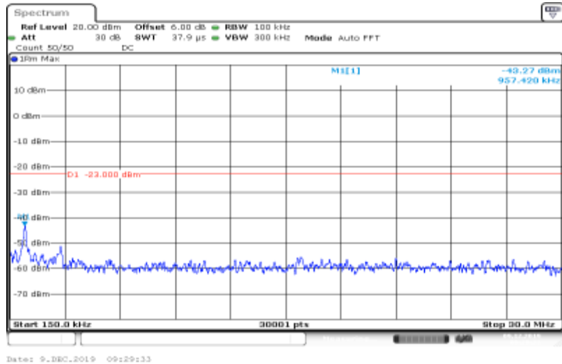
Band II-9538-HSUPA_Sub3-0.15~30
