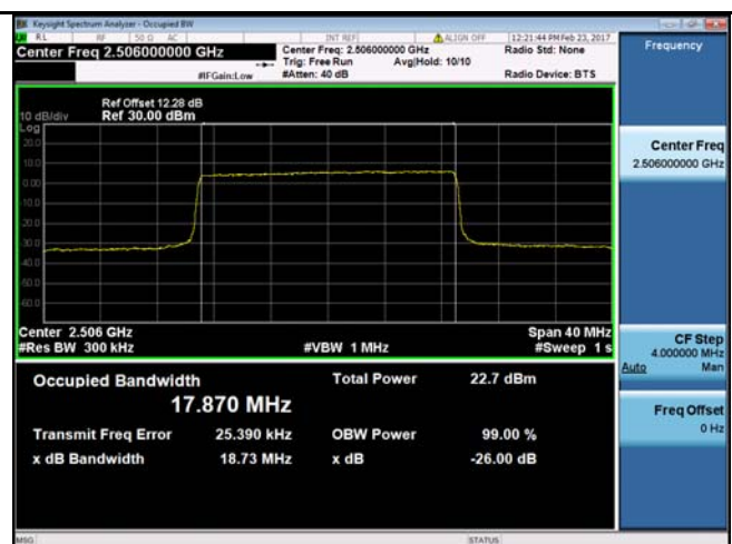
LTE band 41 - Low CH 16QAM-20
