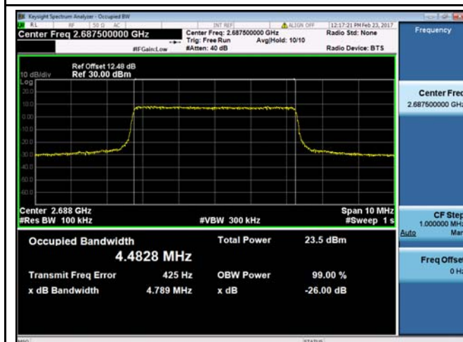
LTE band 41 - High CH QPSK-5
