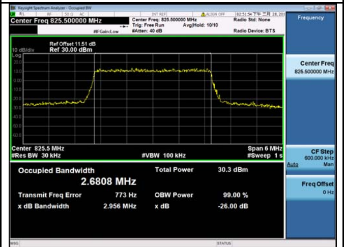
LTE band 26 - Low CH 16QAM-3
