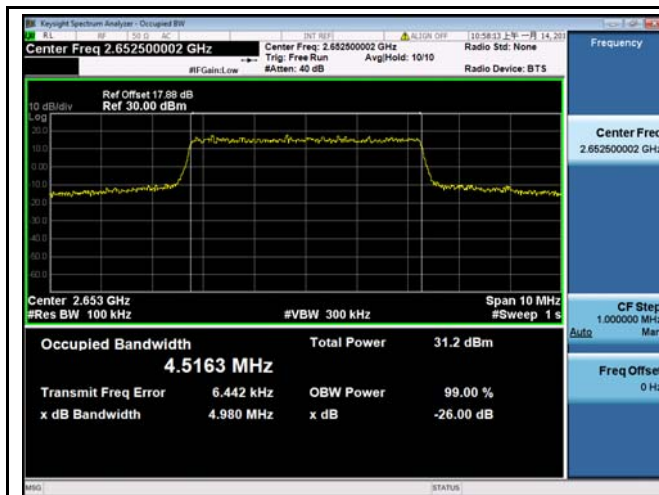
LTE band 41 - High CH QPSK-5
