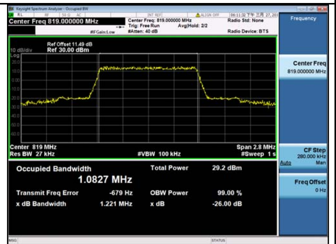
LTE band 26 - Low CH 16QAM-1.4
