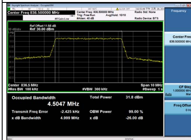
LTE band 26 - Middle CH QPSK-5
