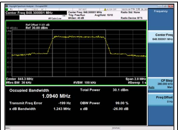
LTE band 26 - High CH 16QAM-1.4
