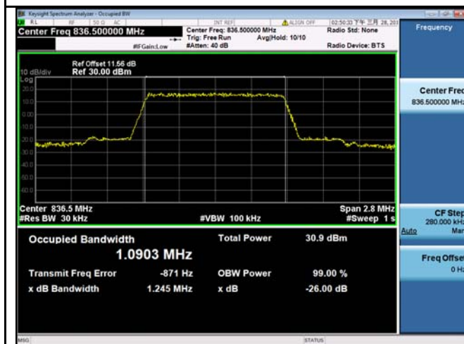
LTE band 26 - Middle CH QPSK-1.4
