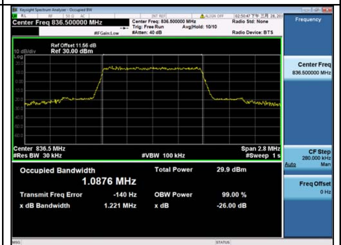
LTE band 26 - Middle CH 16QAM-1.4
