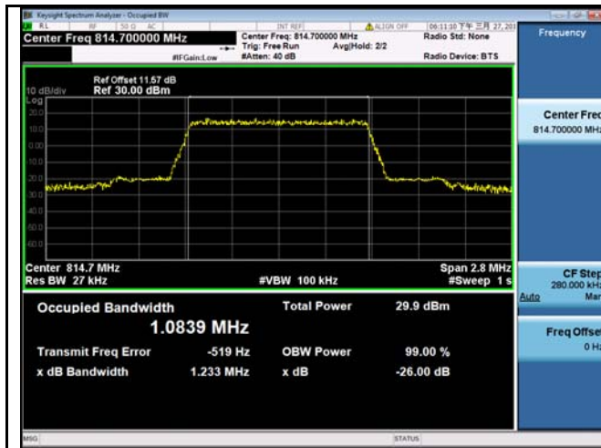
LTE band 26 - Low CH QPSK-1.4
