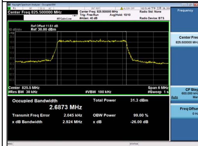
LTE band 26 - Low CH QPSK-3
