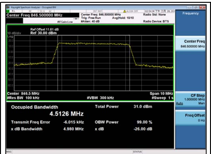
LTE band 26 - High CH 16QAM-5
