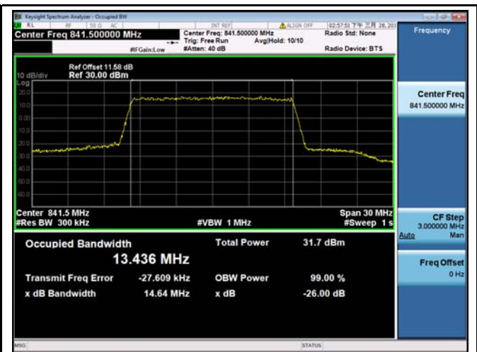
LTE band 26 - High CH 16QAM-15
