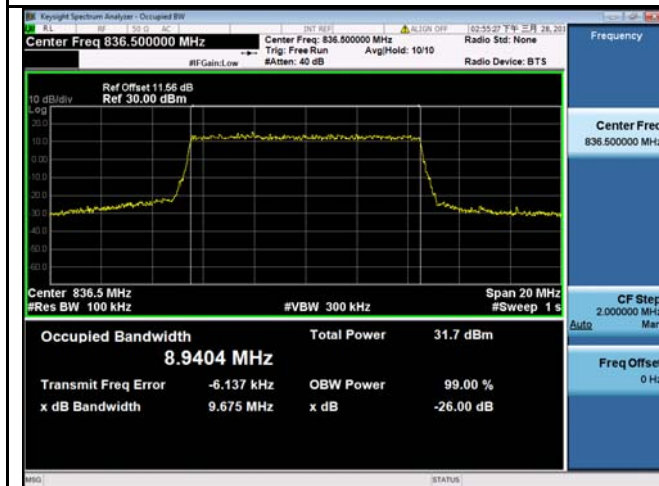
LTE band 26 - Middle CH QPSK-10
