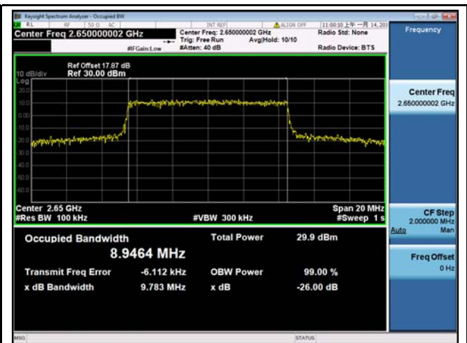
LTE band 41 - High CH 16QAM-10
