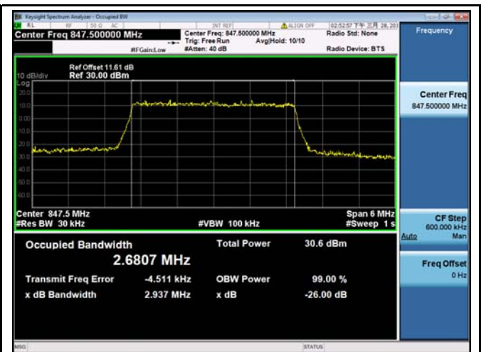
LTE band 26 - High CH 16QAM-3
