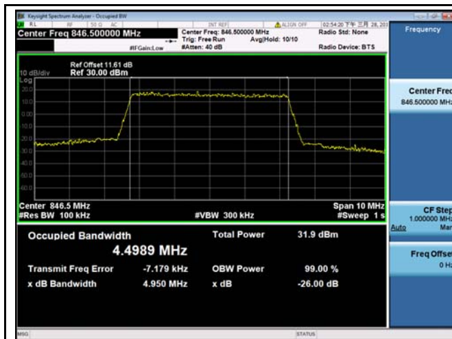
LTE band 26 - High CH QPSK-5
