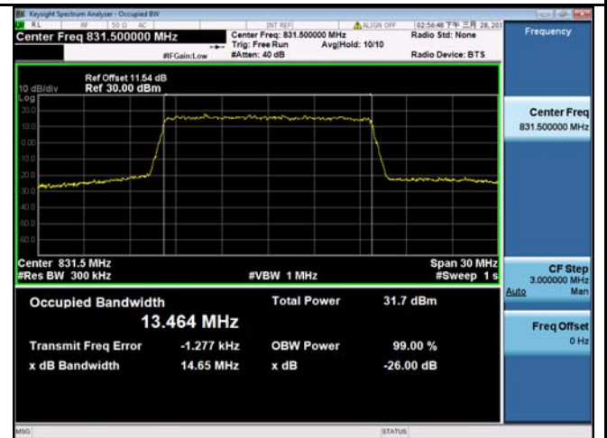
LTE band 26 - Low CH 16QAM-15
