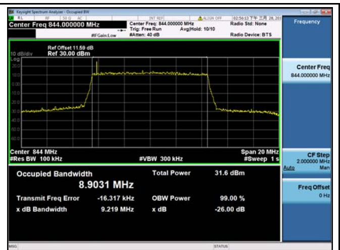
LTE band 26 - High CH 16QAM-10
