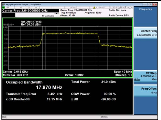
LTE band 41 - High CH 16QAM-20
