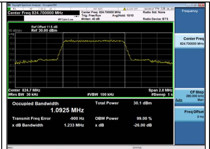
LTE band 26 - Low CH 16QAM-1.4
