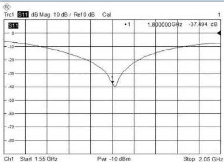
Return loss
