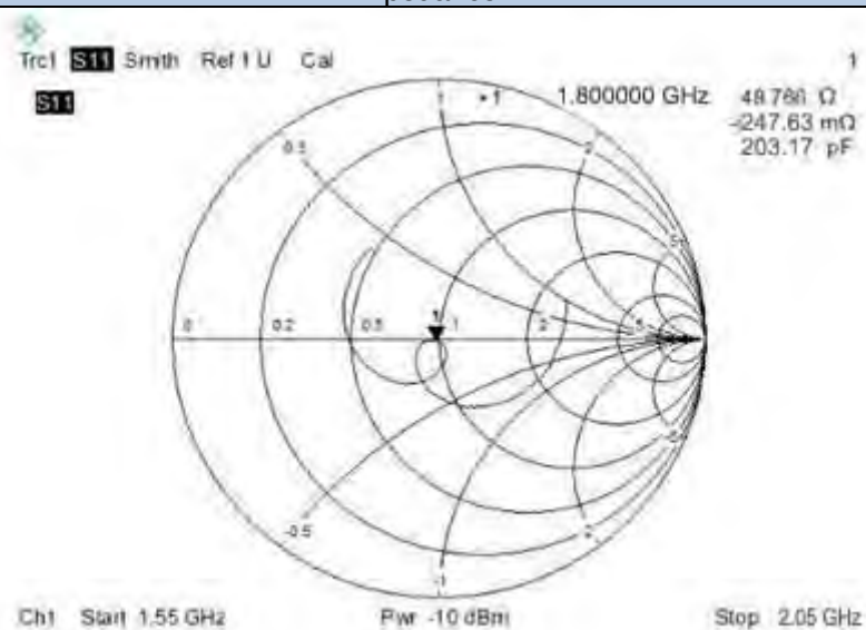
Impedance
