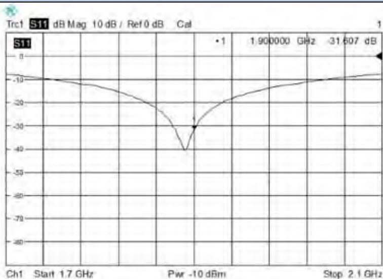
Return loss
