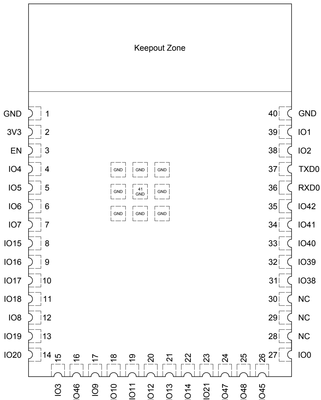
Figure 1: Pin Layout (Top View)
