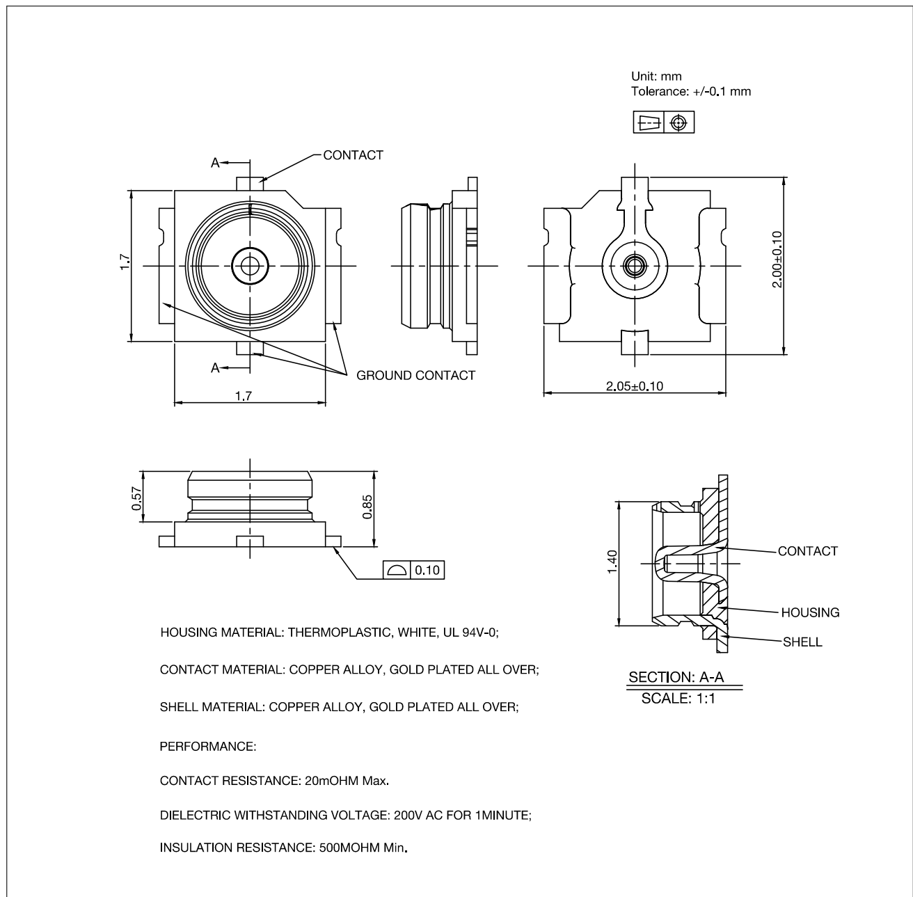
Figure 8: U.FL Connector Dimensions
