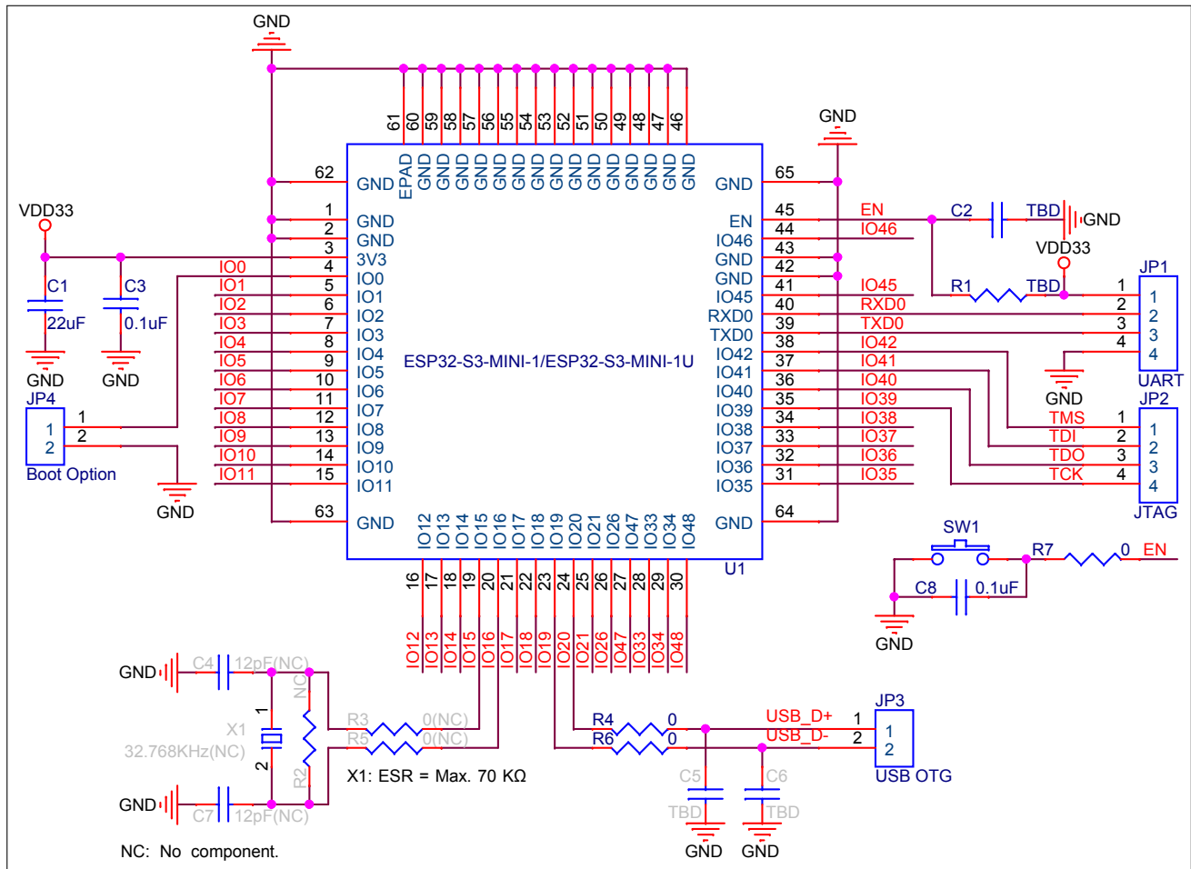
Figure 5: Peripheral Schematics
