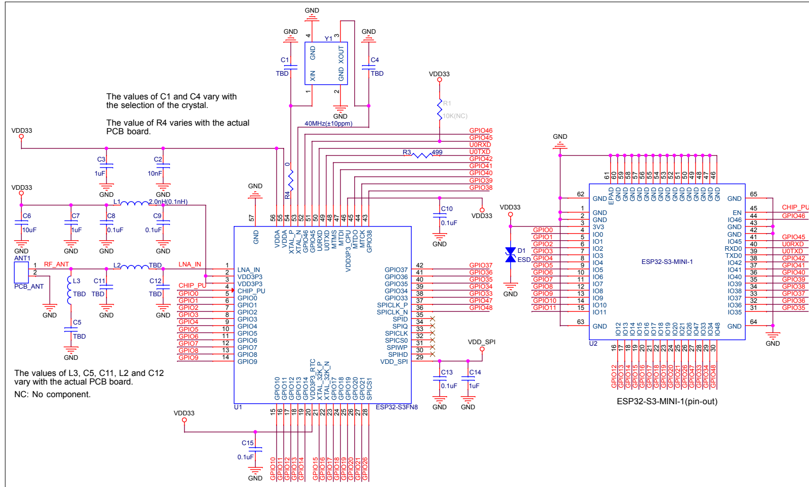
Figure 4: ESP32-S3-MINI-1 Schematics
