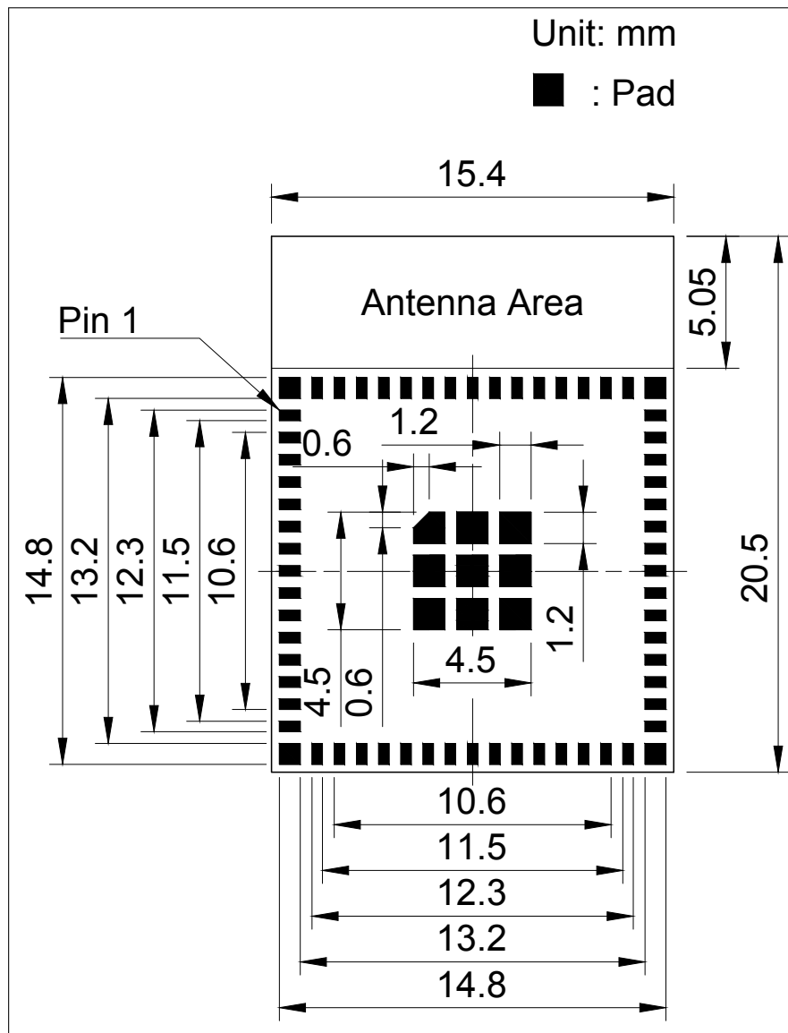
Figure 7: ESP32-S3-MINI-1 Recommended PCB Land Pattern
