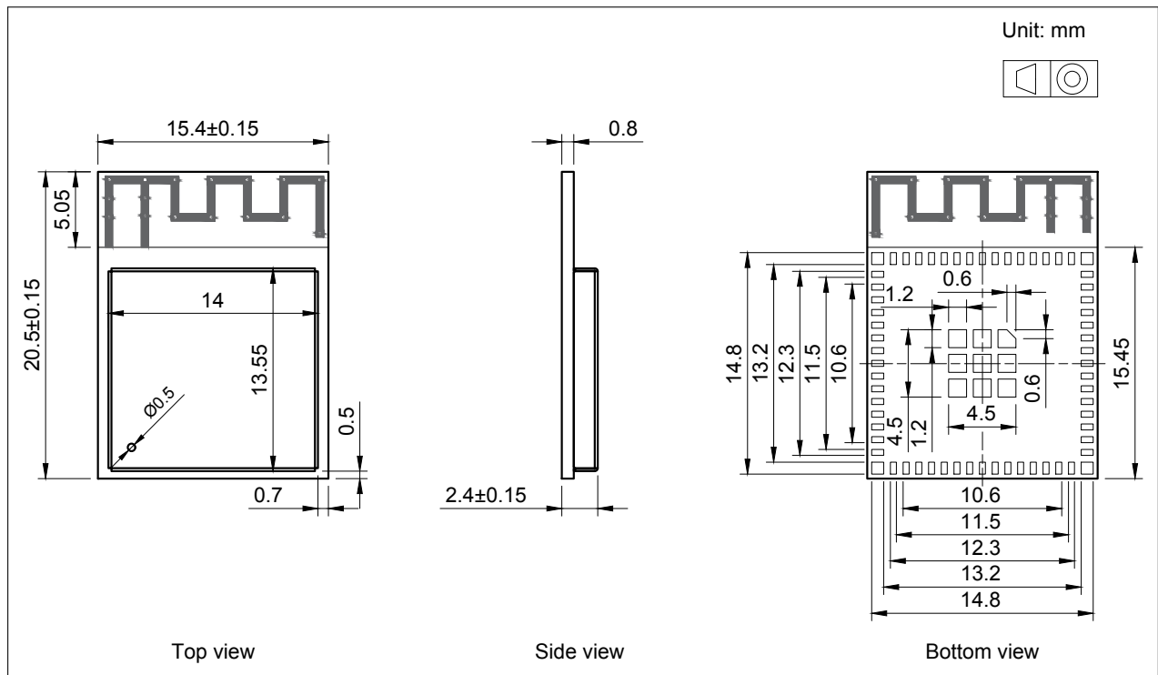
Figure 6: ESP32-S3-MINI-1 Physical Dimensions
