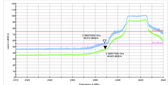
802.11n HT20 -Channel 2 Peak+ Average
