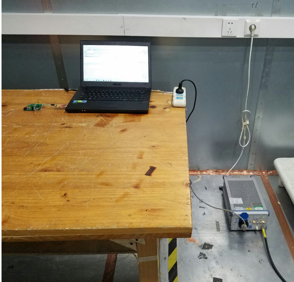
Picture 2 Conducted Emission Test Setup
