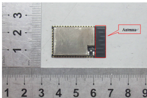
ESP32-S2-WROOM
