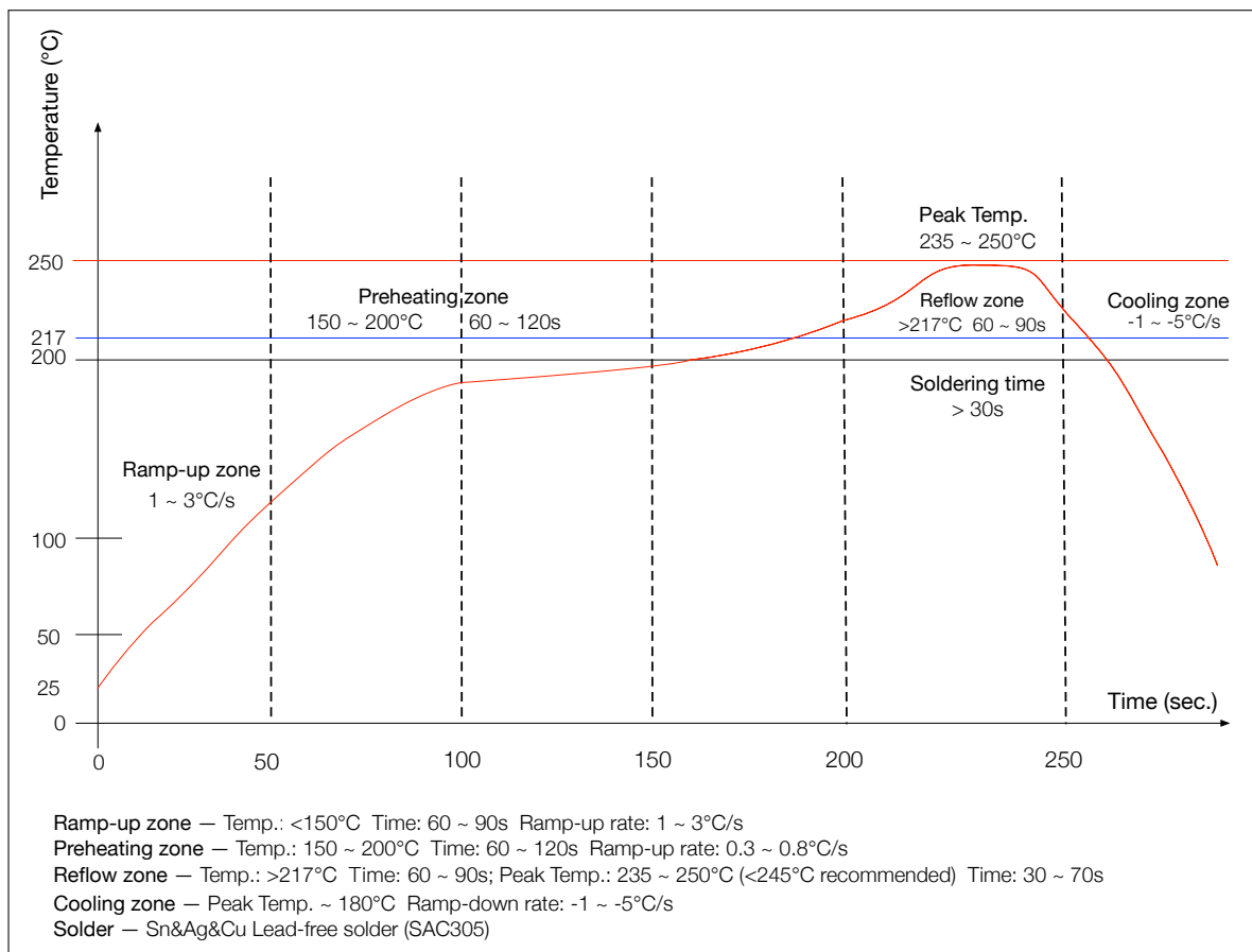
Figure 6: Reflow Profile
