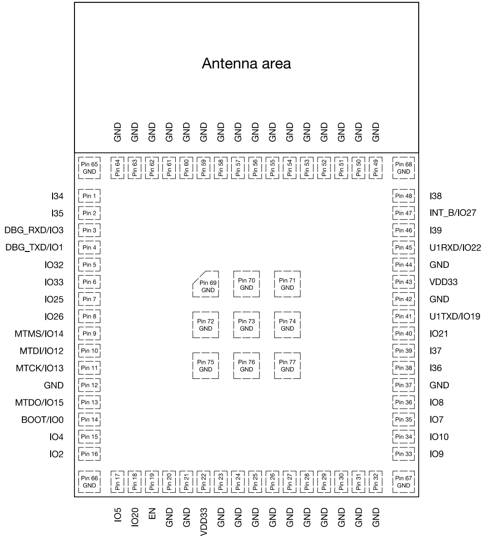
Figure 1: Pin Layout of ESP32-PICO-V3-ZERO (Top View)
