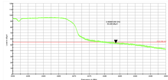
802.11n HT40 -Channel 9 Average
