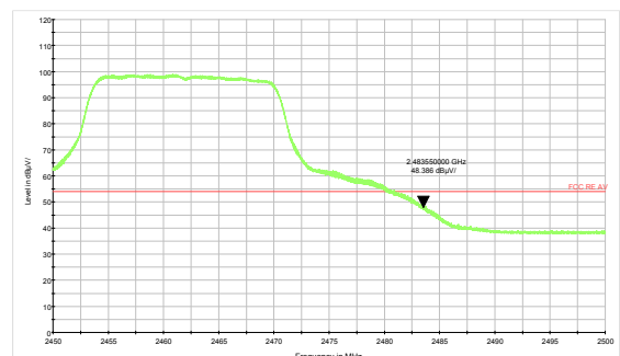
802.11g-Channel 11 Average
