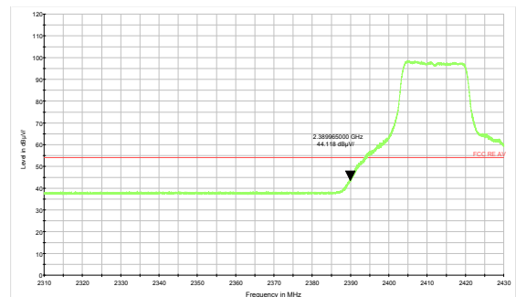
802.11g-Channel 1 Average
