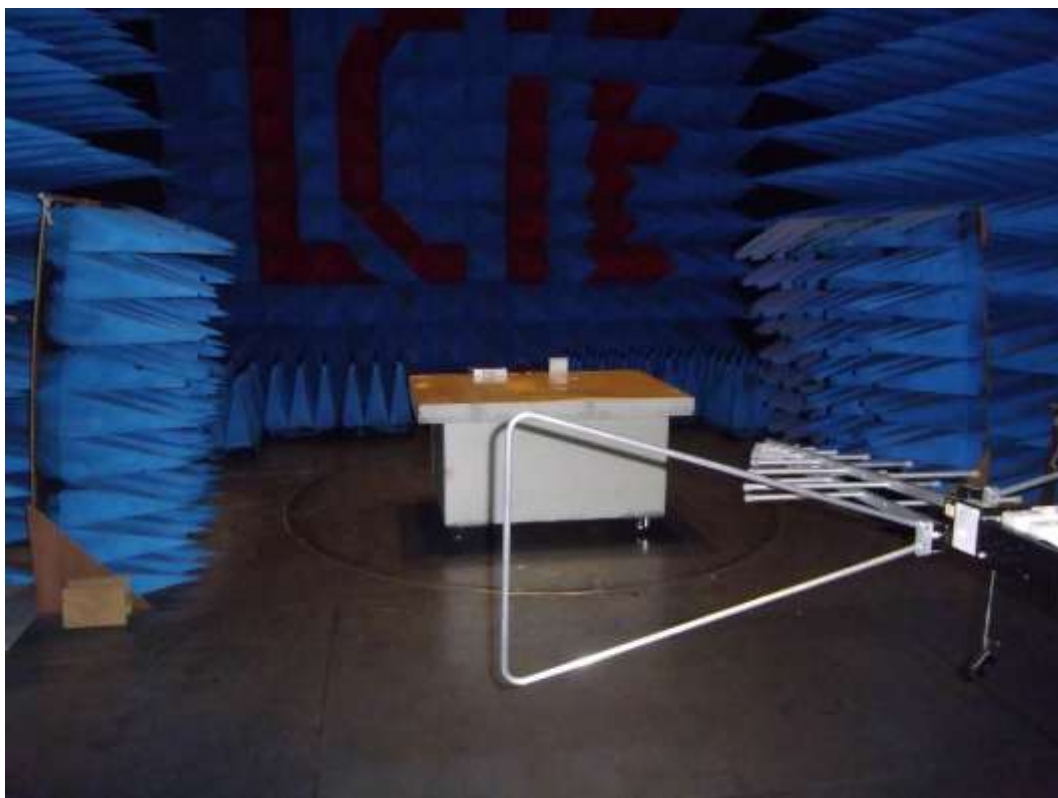
Test setup for Unwanted Emissions into Restricted Frequency Bands
