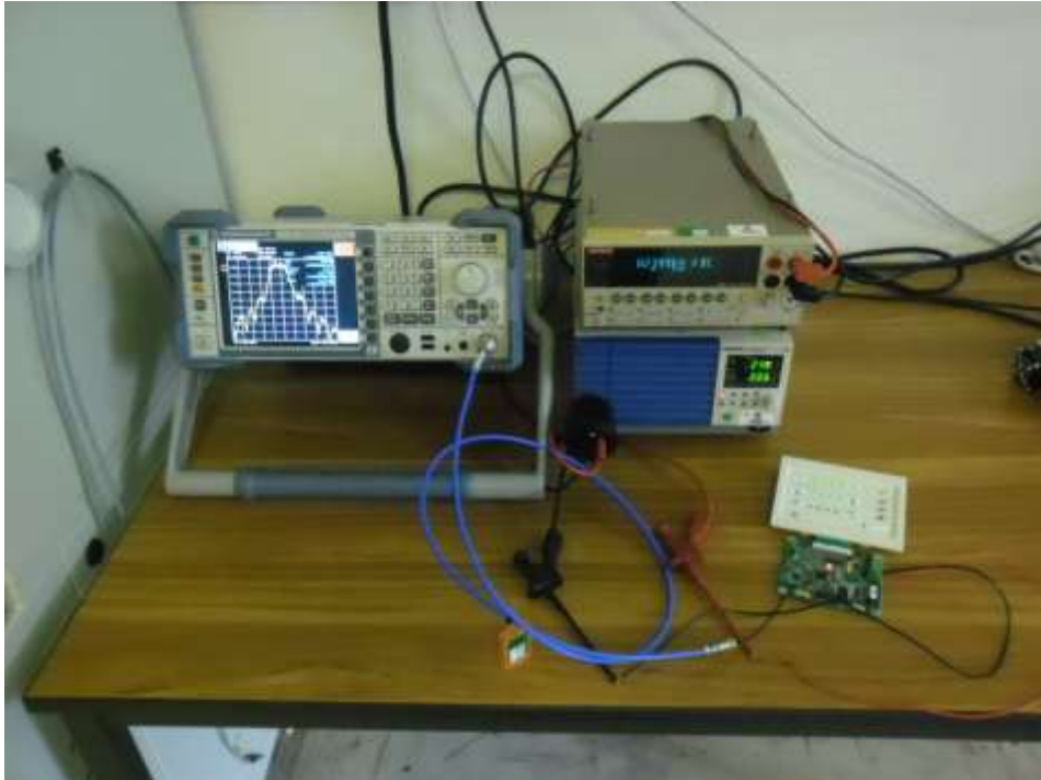
Test setup for -6dB Bandwidth
