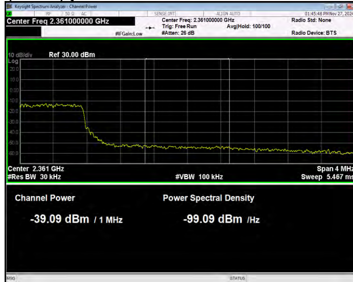
Band40(2350-2360) QPSK BW=5MHz Channel=39225 RB Size=25 Position=#0 Normal
