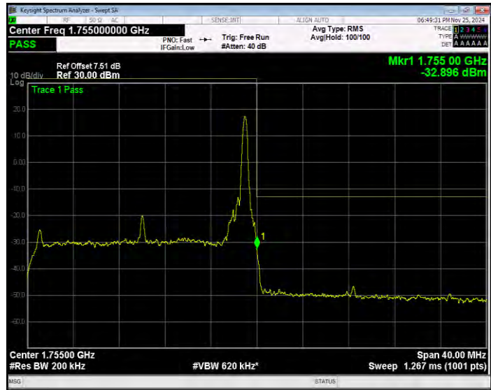
Band4 16QAM BW=20MHz Channel=20300 RB Size=100 Position=#0 Extended
