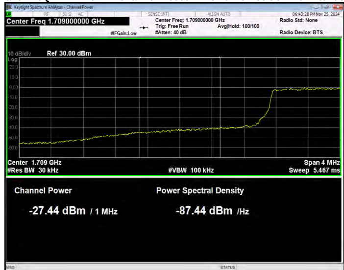
Band4 16QAM BW=3MHz Channel=19965 RB Size=15 Position=#0 Normal
