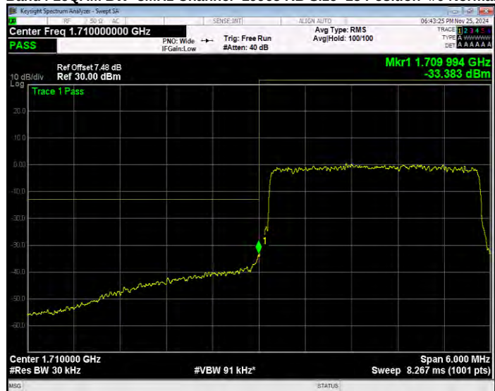
Band4 16QAM BW=3MHz Channel=20385 RB Size=1 Position=#0 Extended
