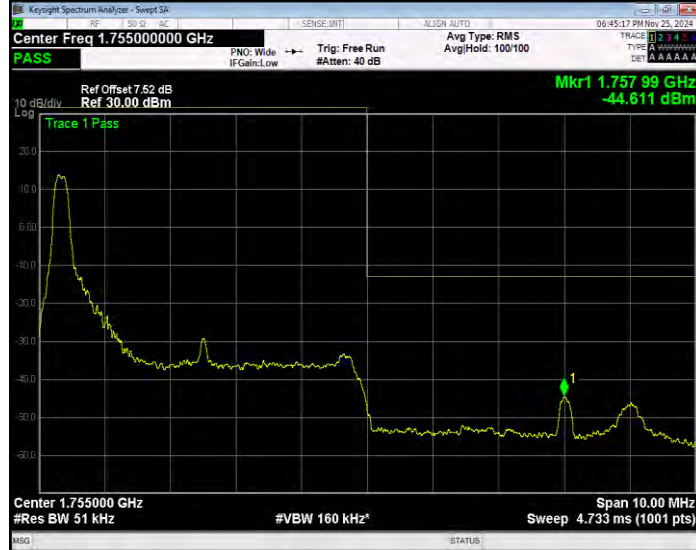
Band4 16QAM BW=5MHz Channel=20375 RB Size=1 Position=#Max Extended
