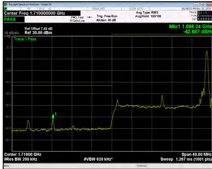
Band4 16QAM BW=20MHz Channel=20050 RB Size=100 Position=#0 Extended
