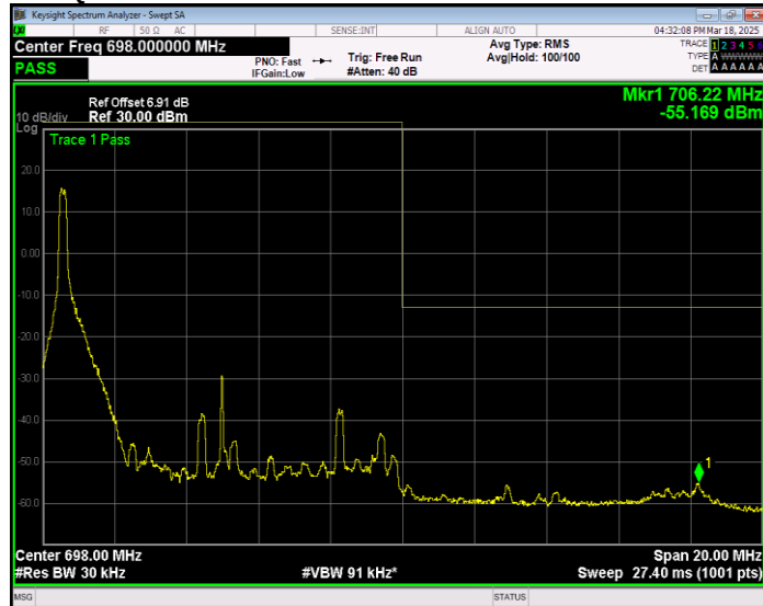
Band71 QPSK BW=10MHz Channel=133422 RB Size=1 Position=#Max Extended
