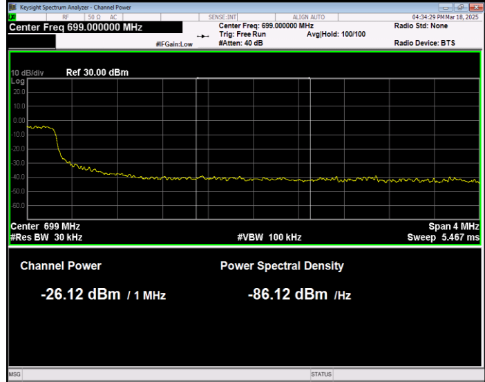
Band71 QPSK BW=20MHz Channel=133222 RB Size=1 Position=#0 Extended
