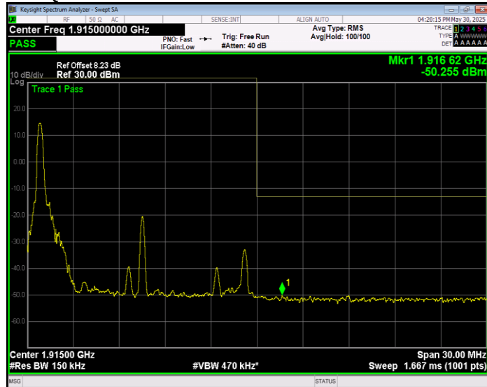
Band25 QPSK BW=15MHz Channel=26615 RB Size=1 Position=#Max Extended
