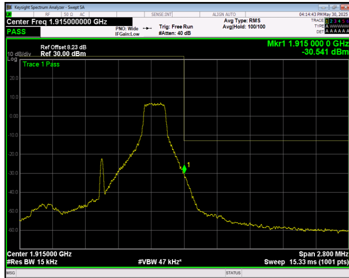
Band25 QPSK BW=1.4MHz Channel=26683 RB Size=6 Position=#0 Extended
